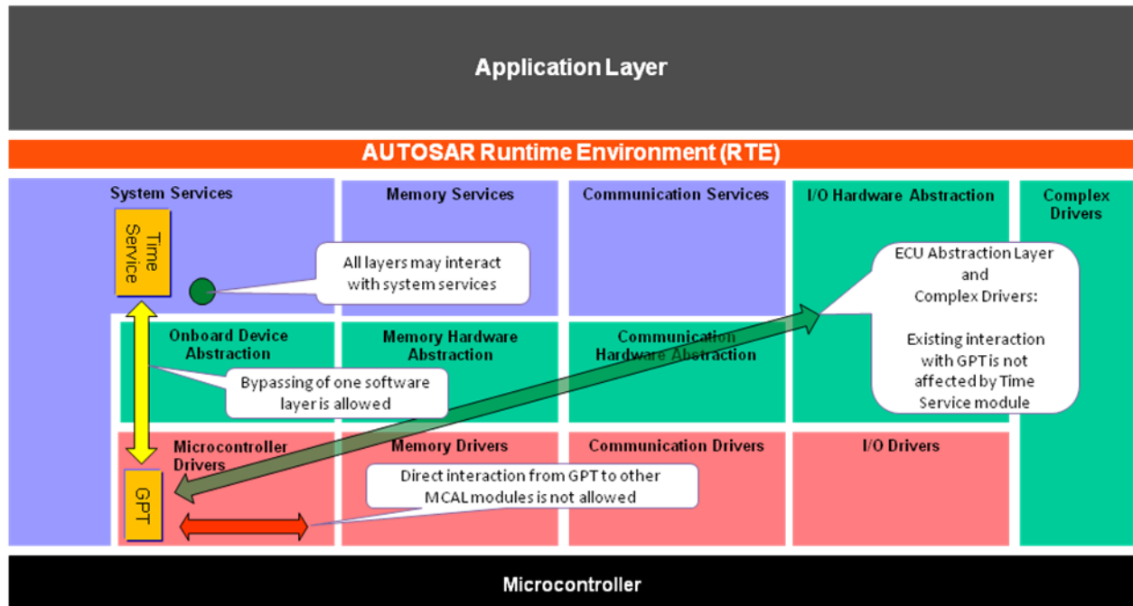
Figure 1 – Architectural overview
