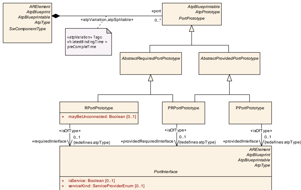
Figure 4.3: Software-Components and Ports
