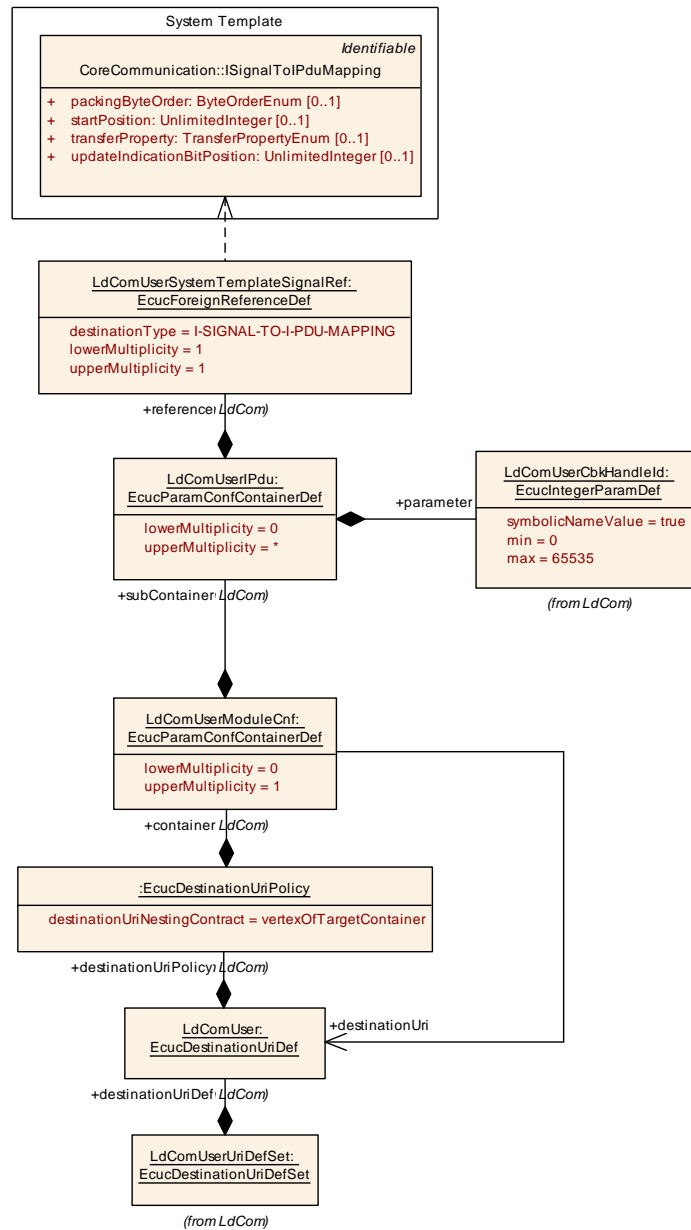
Figure 8.46: Configuration of LdCom User Module Cnf
