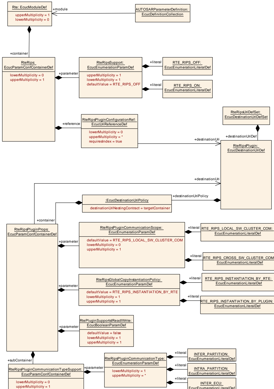
Figure 8.39: Configuration of RTE Implementation Plug-Ins
