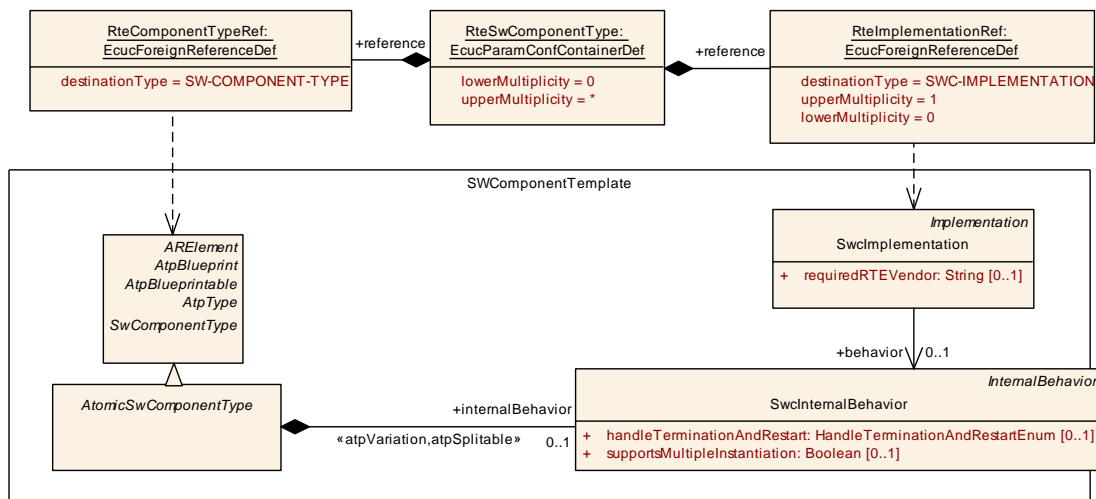
Figure 8.20: Selection of the Implementation for an AtomicSwComponentType
