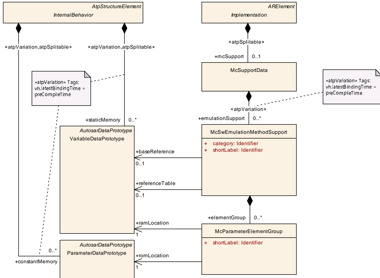
Figure 4.33: Structure of the McSwEmulationMethodSupport element
