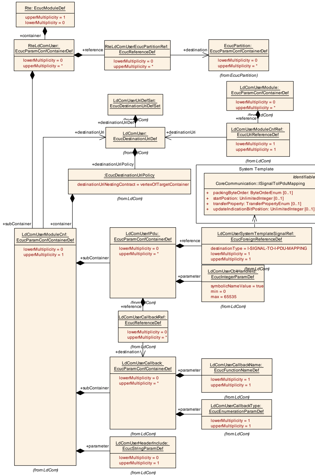
Figure 8.45: Configuration of LdCom User
