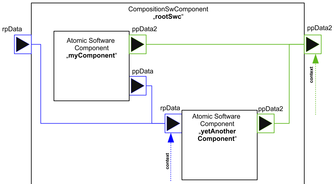
Figure 7.4: N:1 Data Communication Graph involving Cross Cluster Communication
