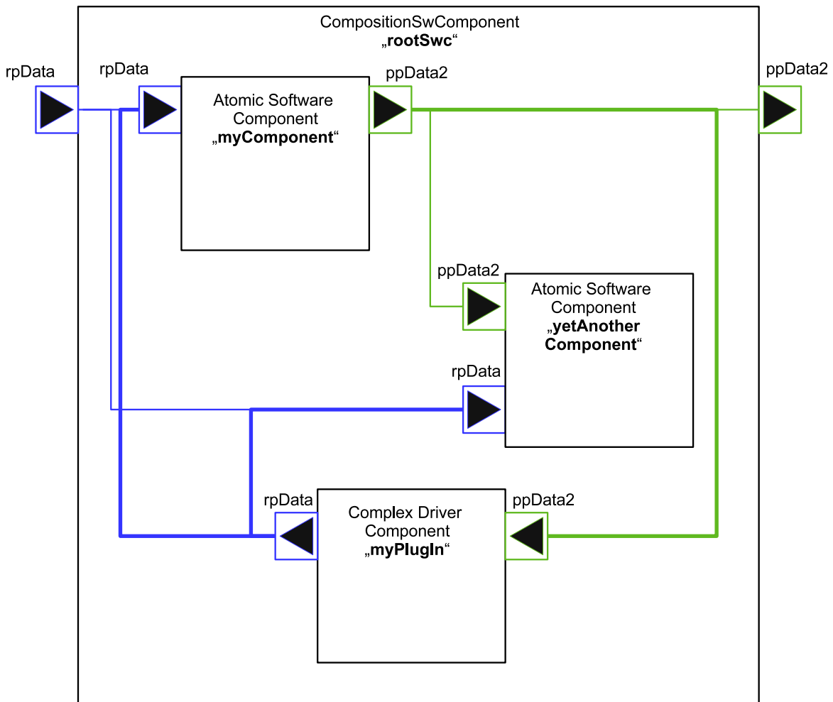
Figure 7.9: Example of implicit communication via RTE Implementation Plug-In
