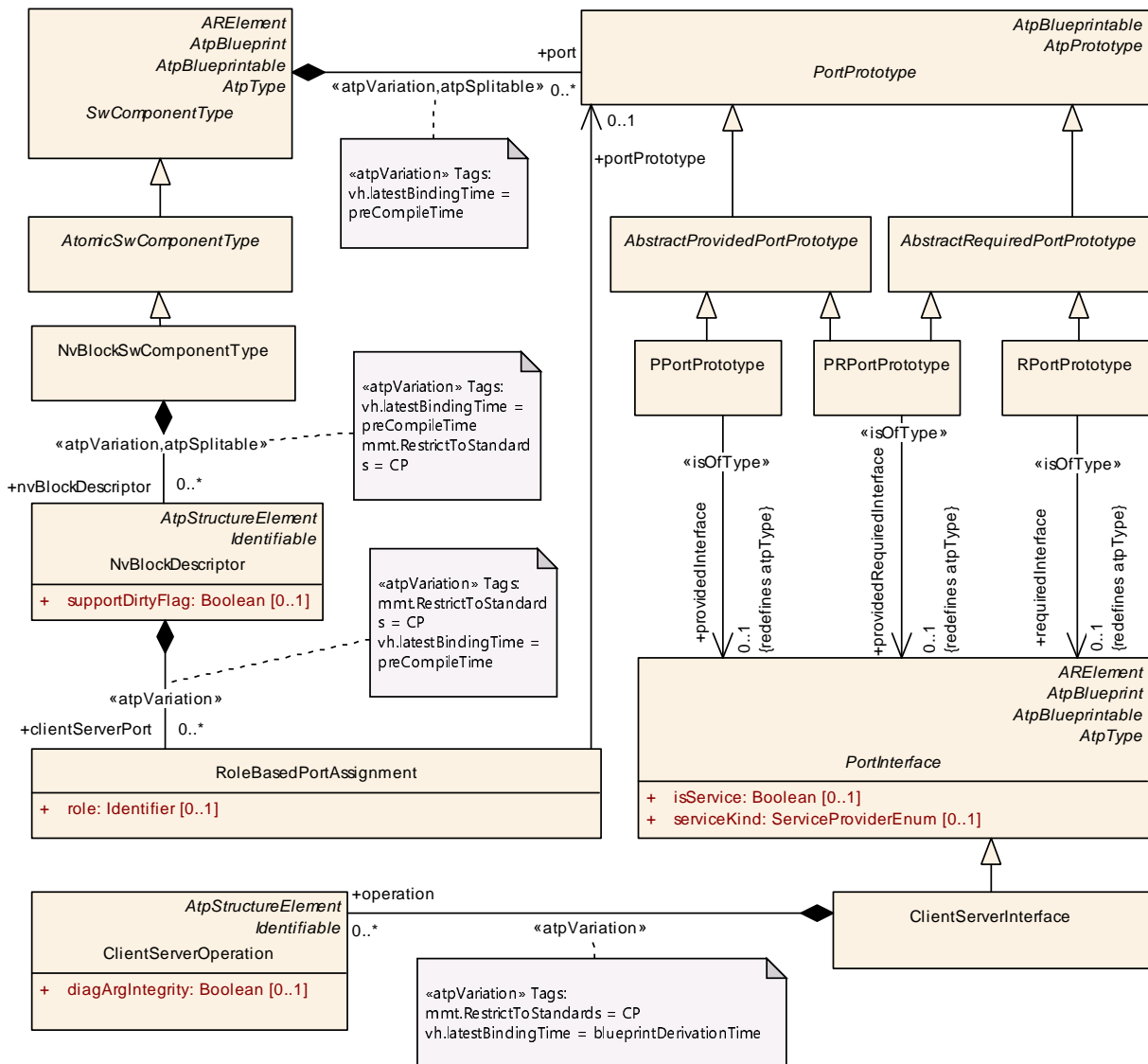
Figure 4.39: NVM notifications
