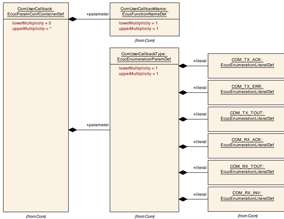
Figure 8.44: Configuration of Com Callbacks
