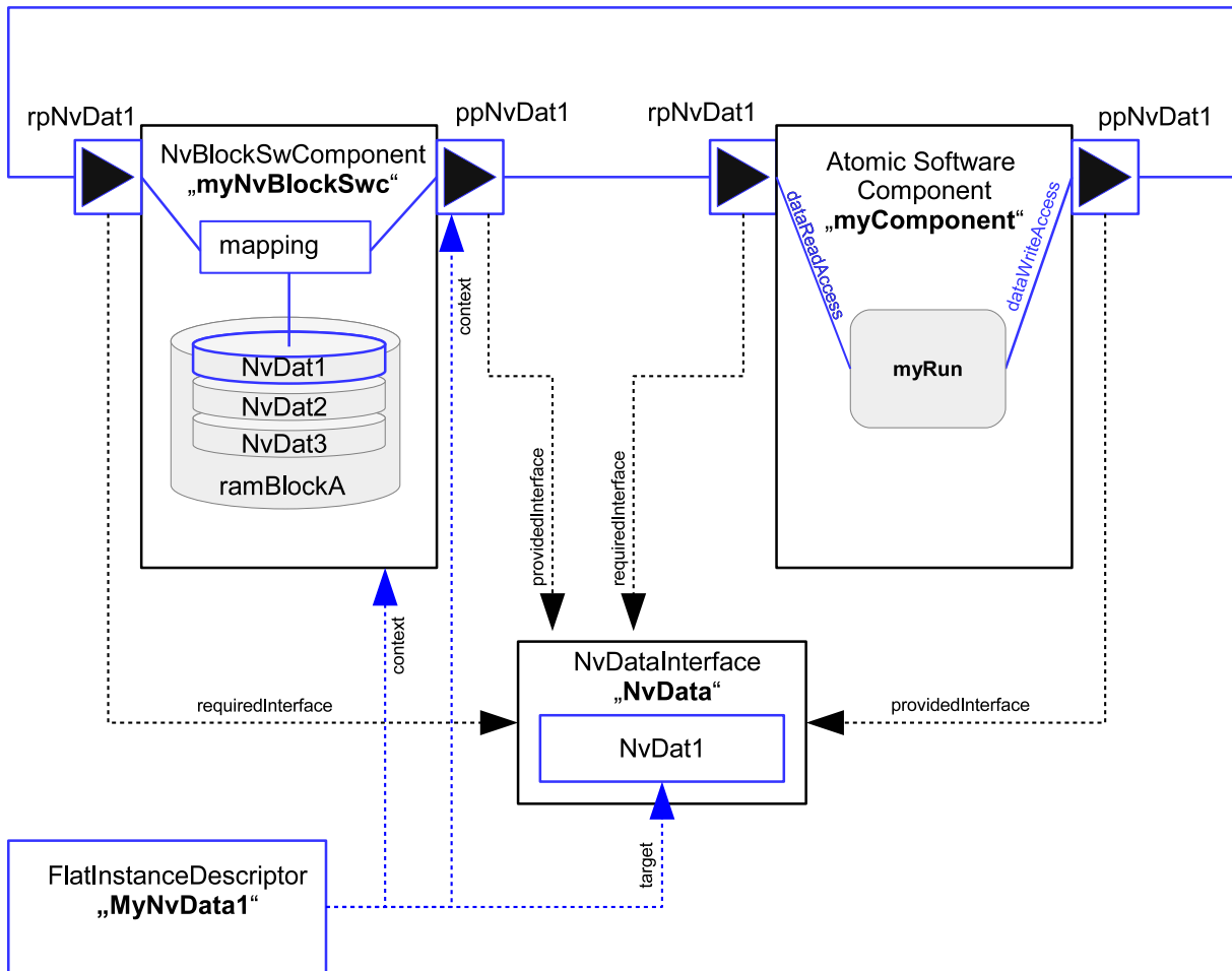
Figure 7.6: Data Communication Graph involving a NvBlockSwComponent
