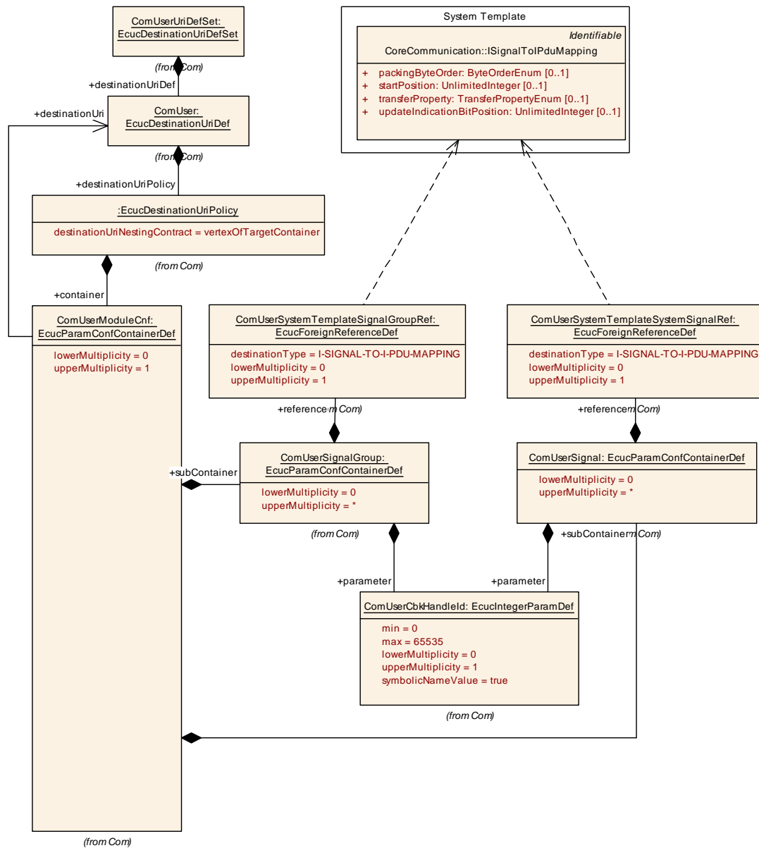
Figure 8.43: Configuration of Com User Module Cnf
