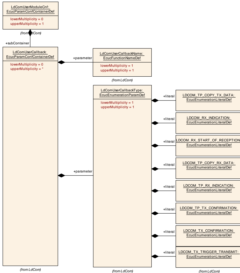
Figure 8.47: Configuration of LdCom Callbacks
