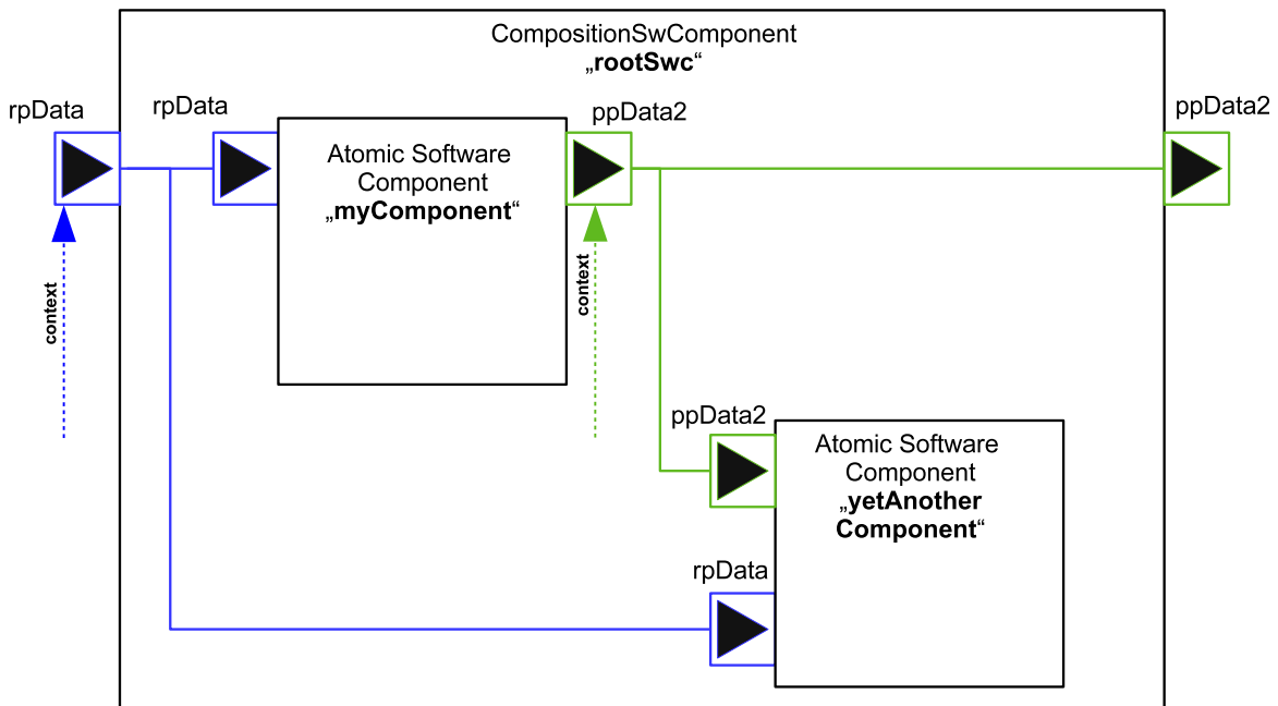
Figure 7.3: 1:N Data Communication Graph involving Cross Cluster Communication
