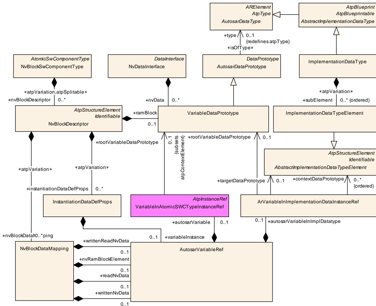
Figure 4.37: NvBlockDataMapping
