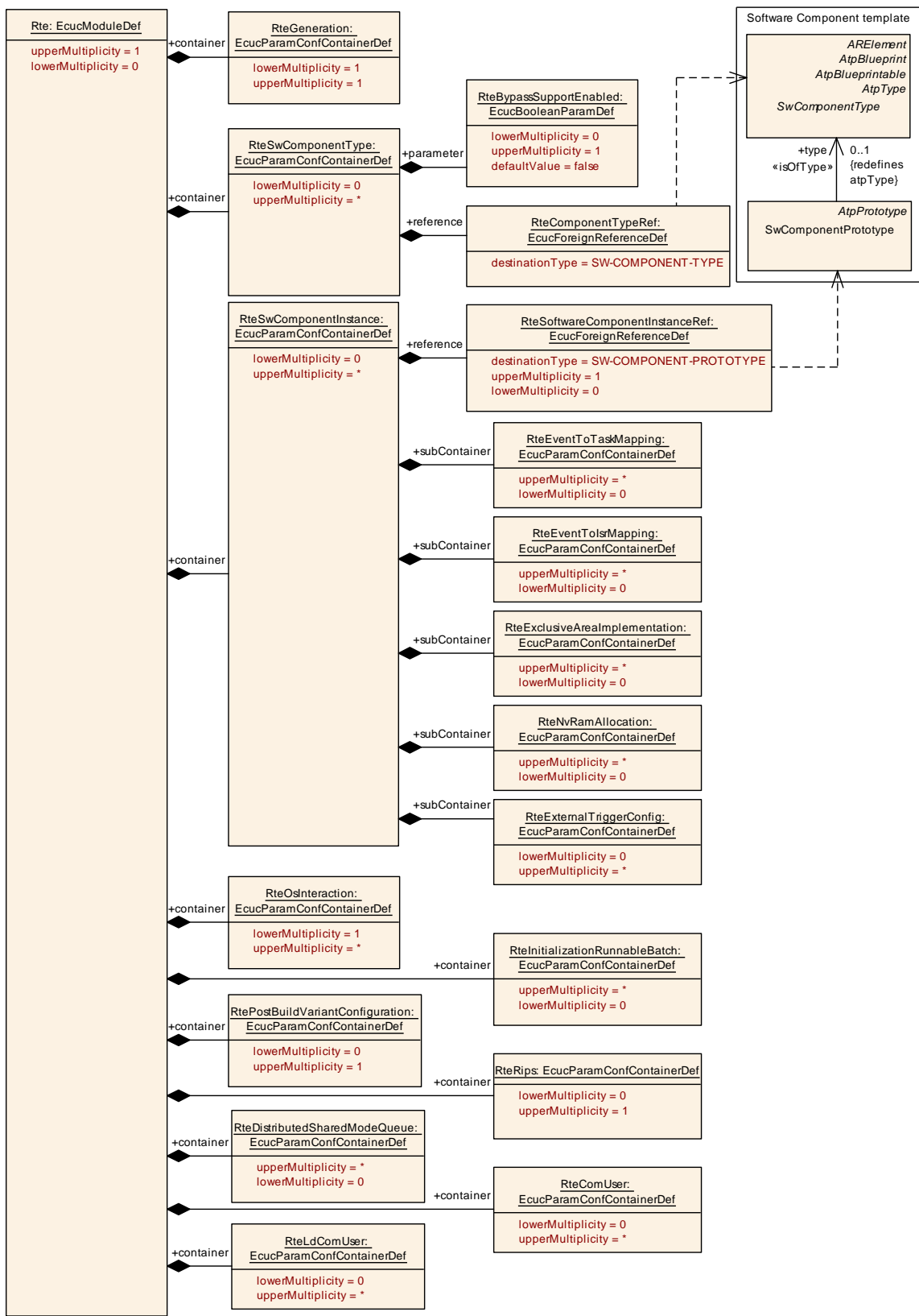
Figure 8.2: RTE configuration overview
