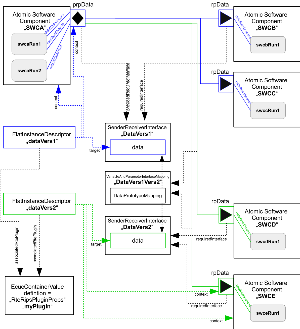
Figure 7.5: Data Communication Graph with conversion
