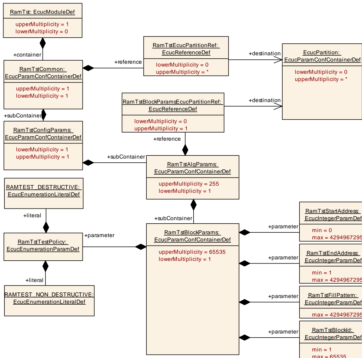
Figure 19: RamTstBlockParams
