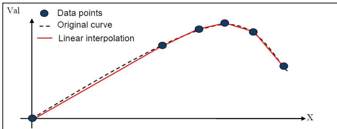
Figure 8.2: Linear interpolation
