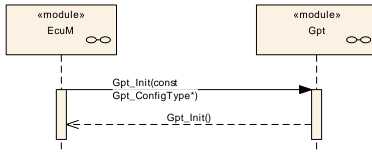
Figure 6: Sequence Diagram - Gpt_Init
