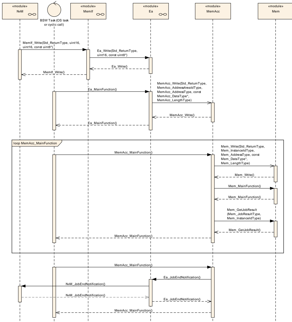
Figure 5: Sequence diagram “Ea_Write”
