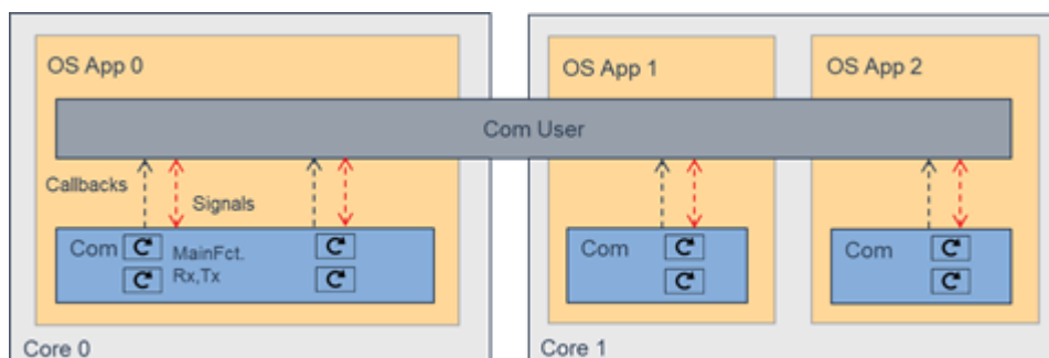
Figure 11 A partition unpecific Com user and its interaction with partition specific Com instances
