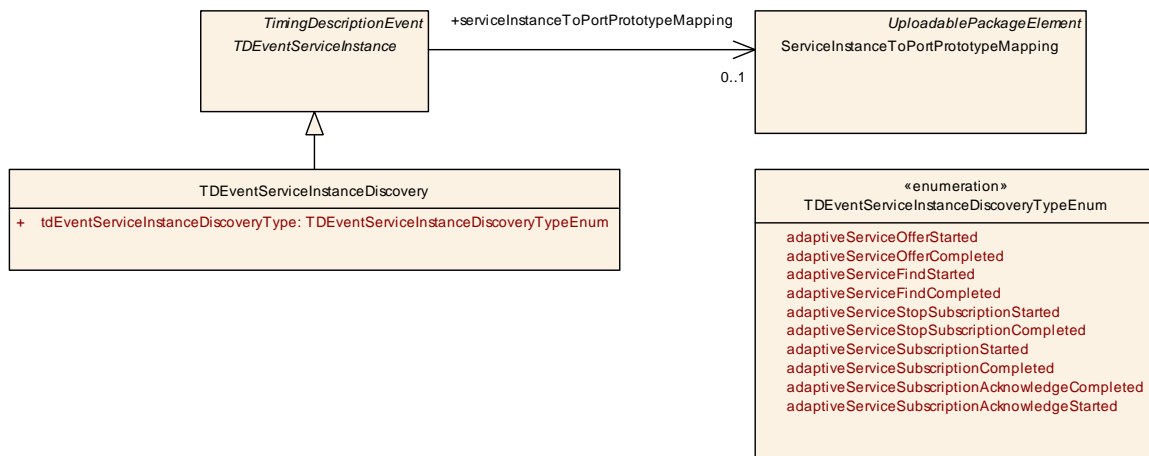
Figure 5.11: Adaptive Service Discovery
