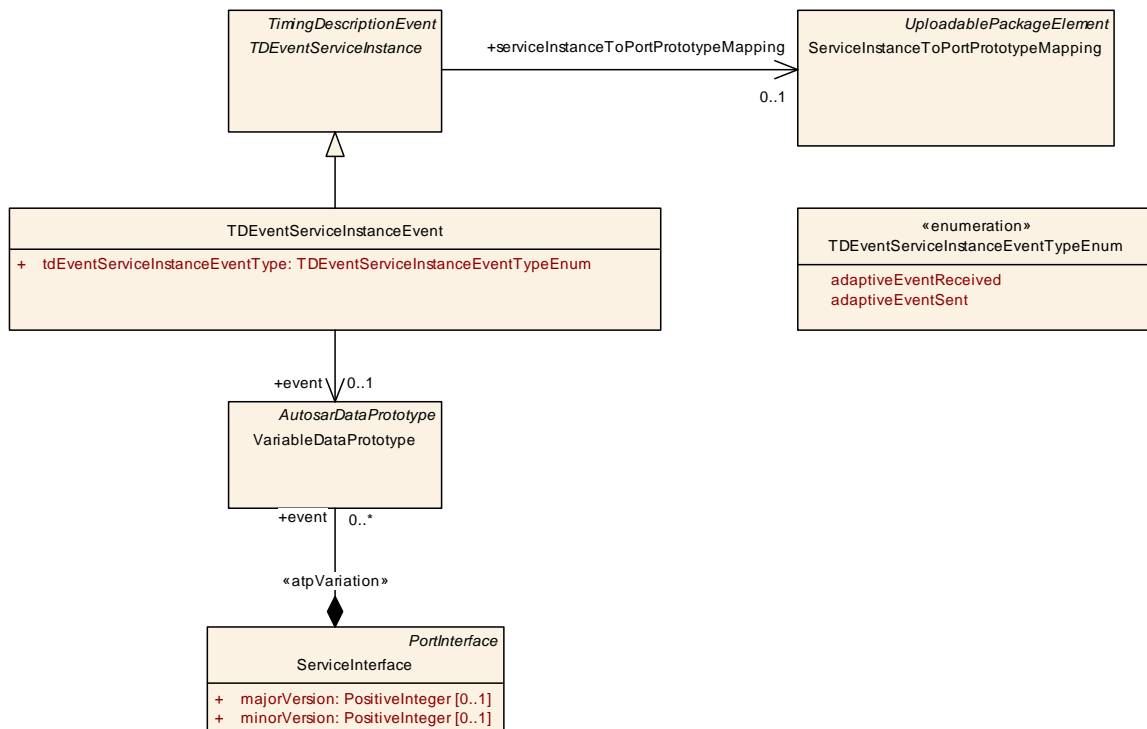
Figure 5.8: Adaptive Service Event
