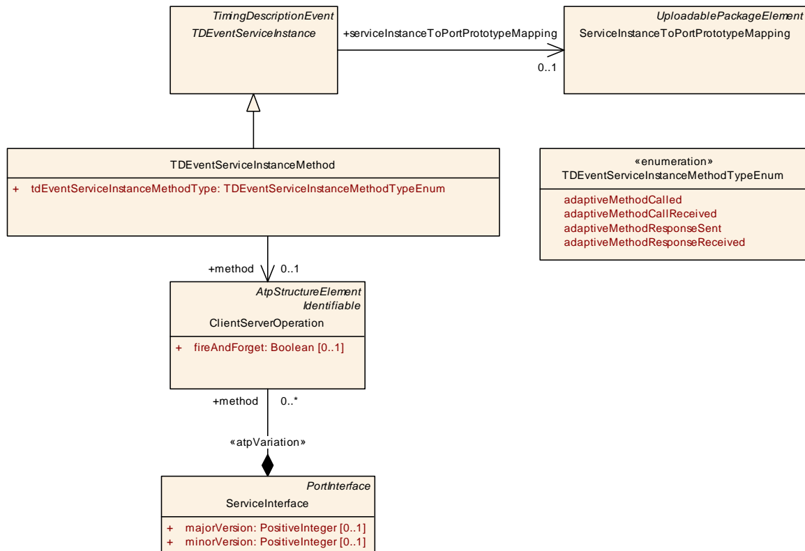
Figure 5.10: Adaptive Service Method
