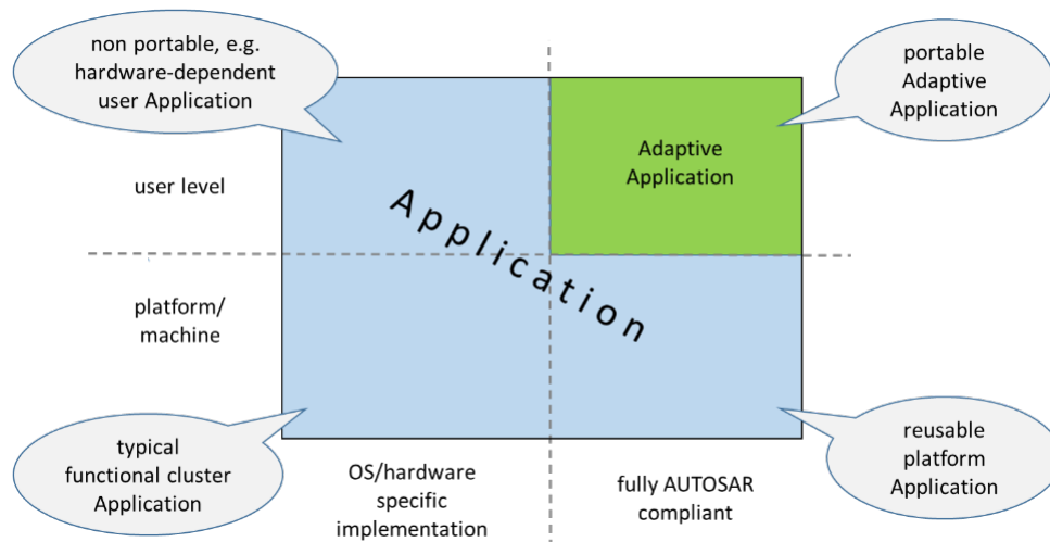
Figure 4.2: Applications
