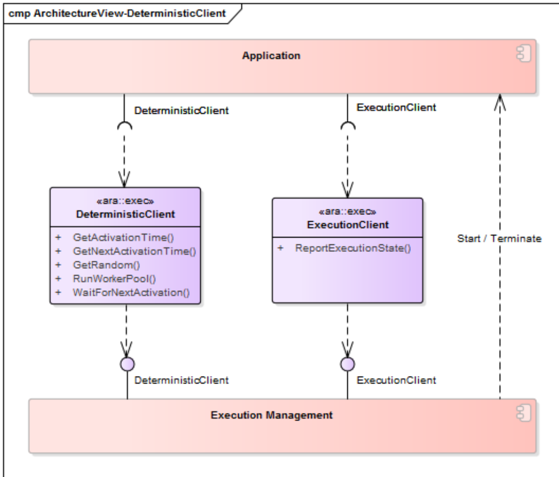
Figure 6.2: Deterministic Client
