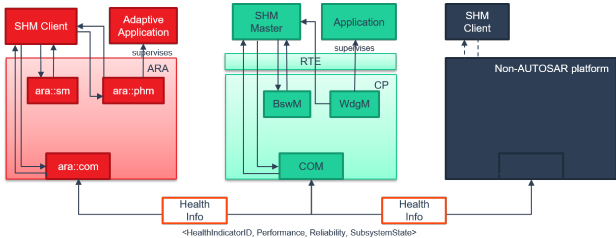
Figure 17.2: SHM overview
