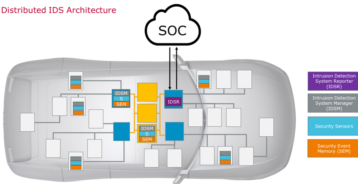
Figure 19.1: Distributed IDS Architecture
