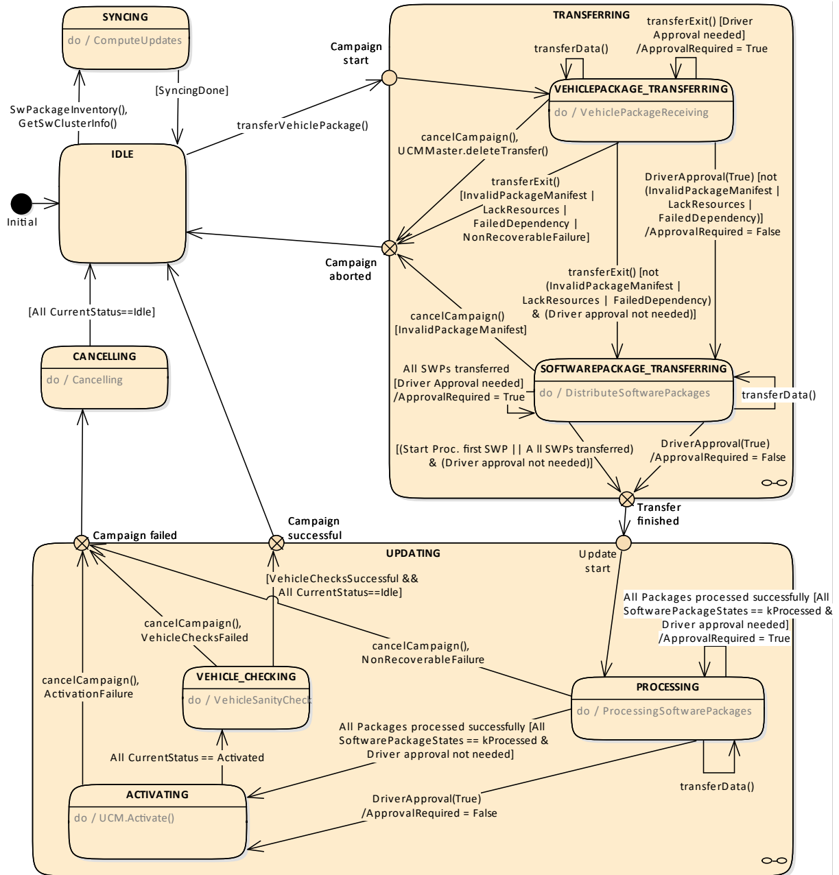
Figure 13.9: UCM Master state machine
