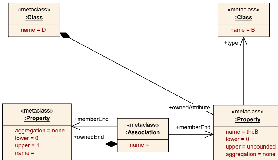
Figure 3.3: Representation of association (aggregation = none)
