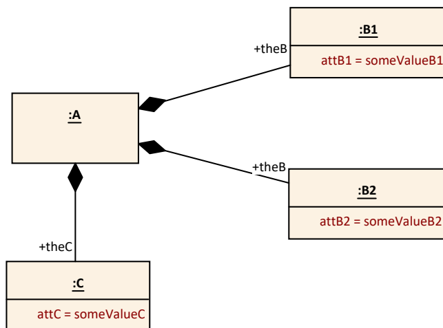
Figure 5.14: Example instance of composite property
