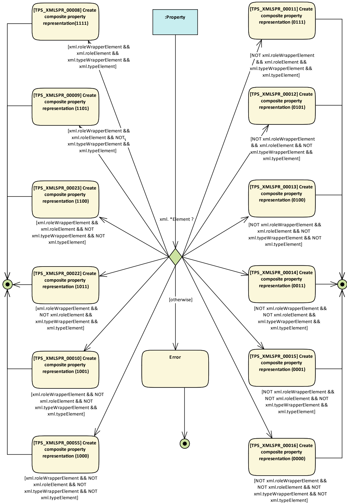
Figure 5.12: Property representation (aggregation composite)
