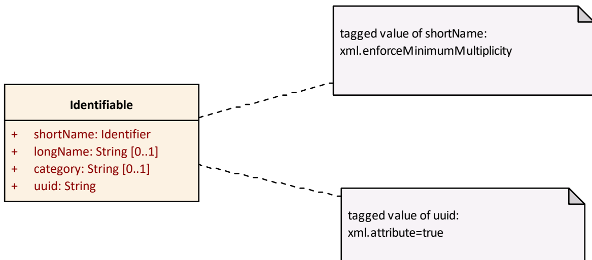
Figure 5.3: UML example - Create xsd:group
