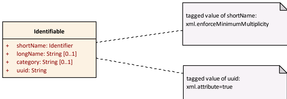
Figure 5.4: UML example - Create xsd:attributeGroup
