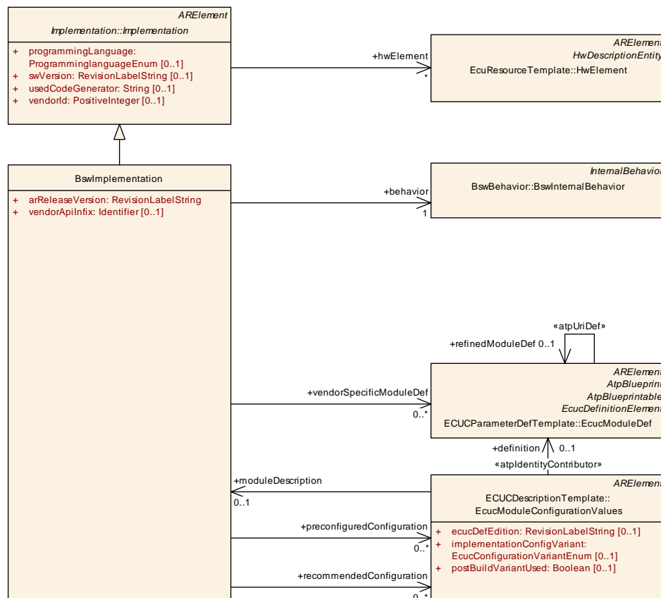
Figure 7.1: Overview of class BswImplementation
