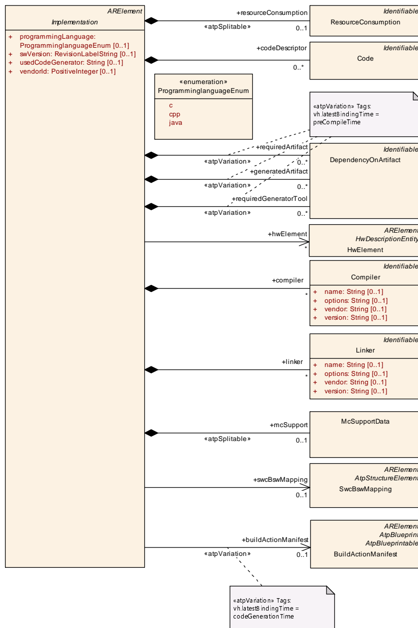
Figure 8.1: Overview of implementation description
