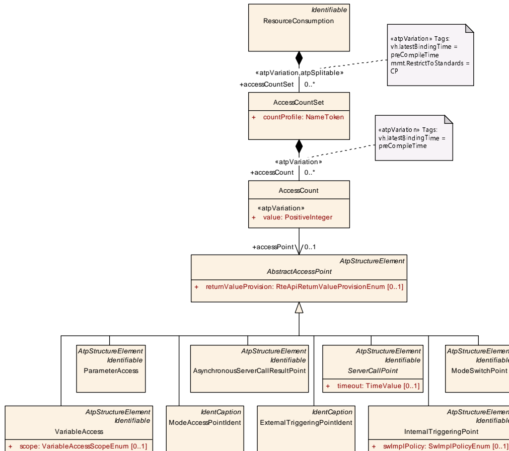
Figure 5.7: Overview AccessCountSet
