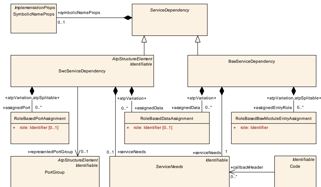
Figure 13.1: Concept of ServiceDependency for BSW and SWC
