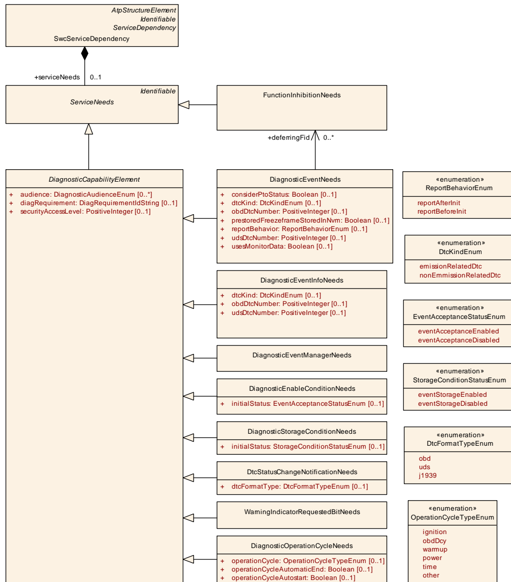
Figure 13.5: Class ServiceNeeds from CommonStructure and derived classes for diagnosis use cases
