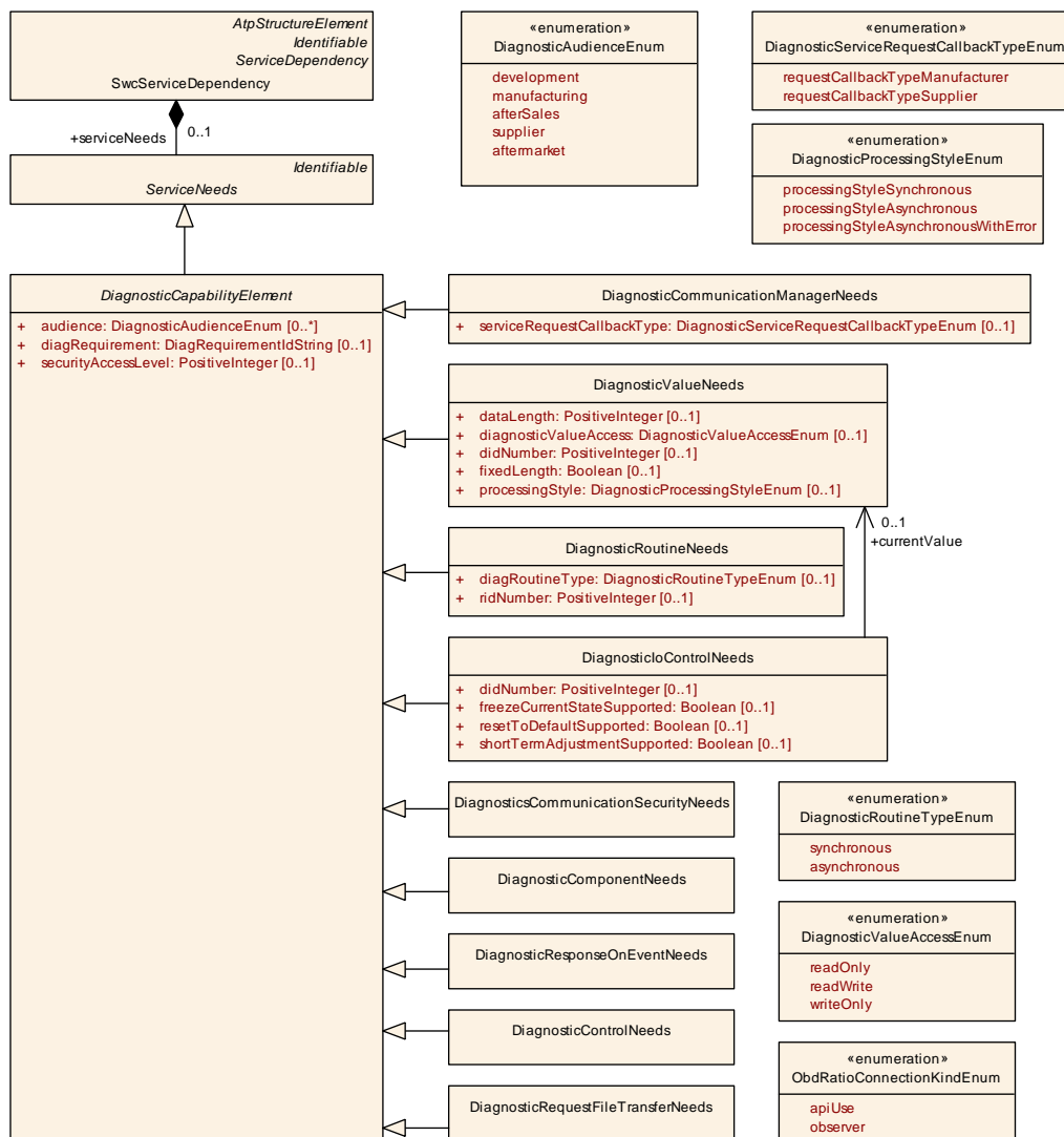
Figure 13.4: Class ServiceNeeds from CommonStructure and derived classes for diagnosis use cases
