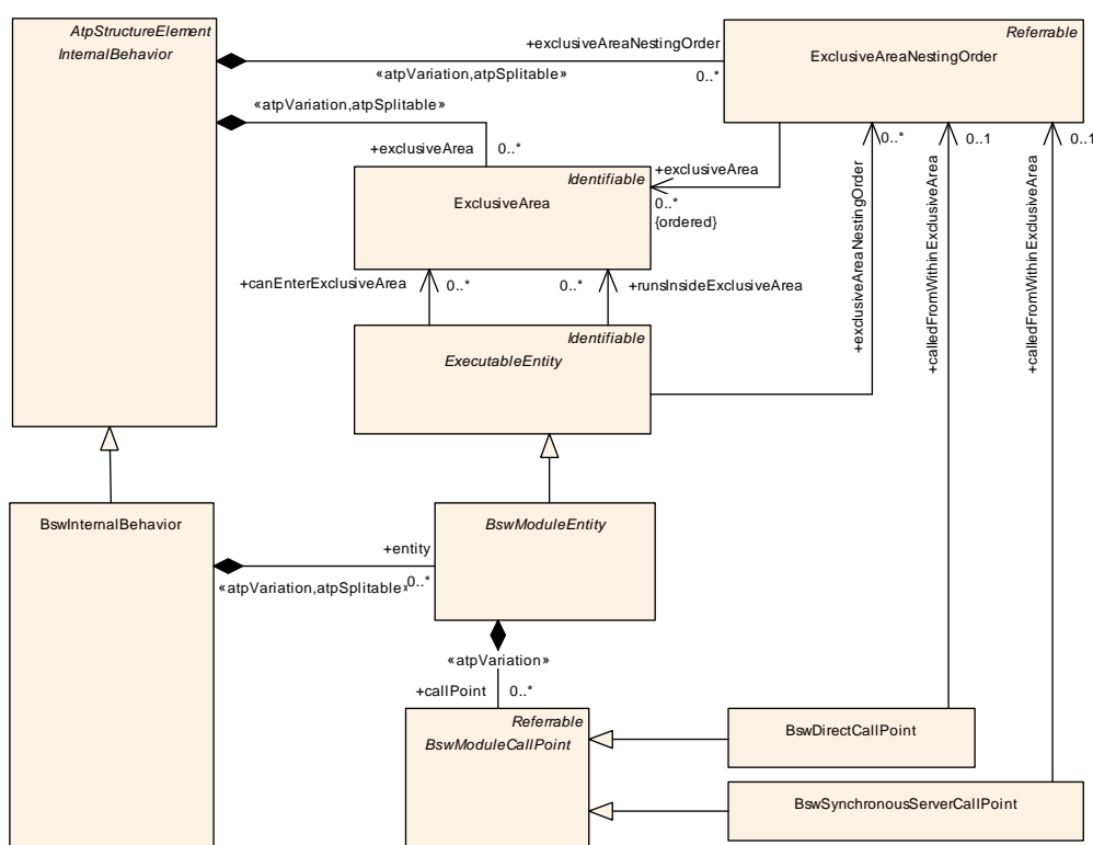
Figure 6.5: Details of defining ExclusiveAreas in BSWMDT
