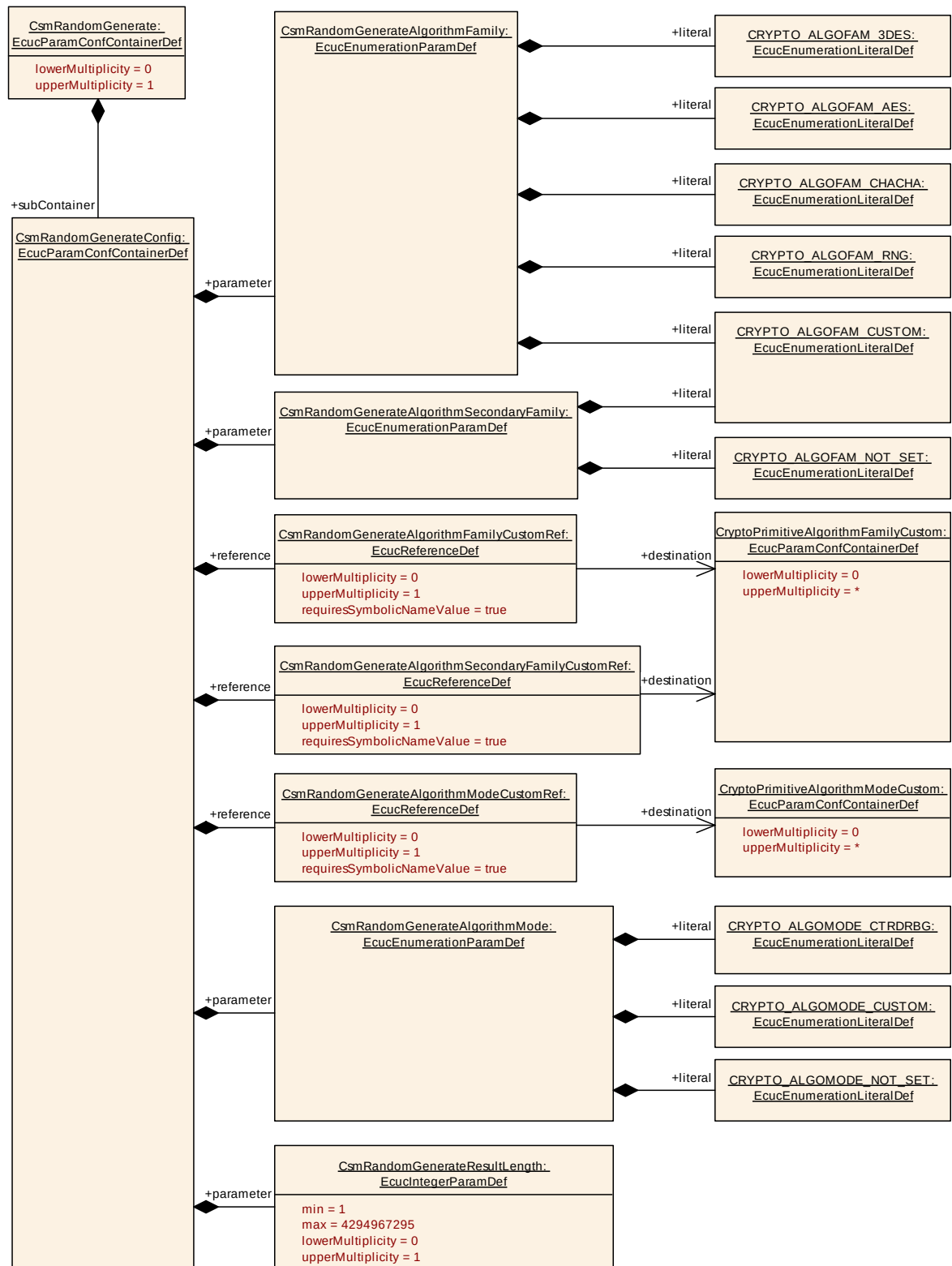
Figure 9-21 CsmRandomGenerate Layout
