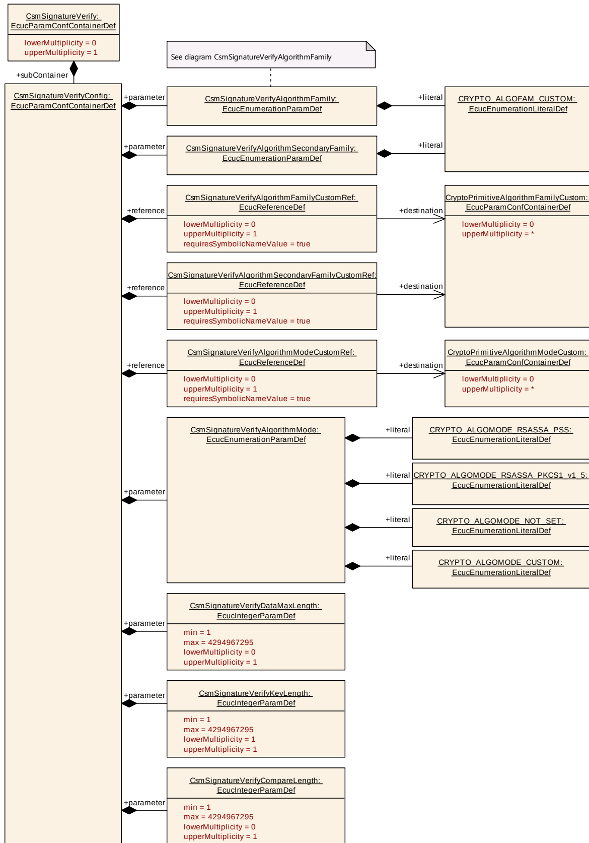
Figure 9-20 CsmSignatureVerify Layout
