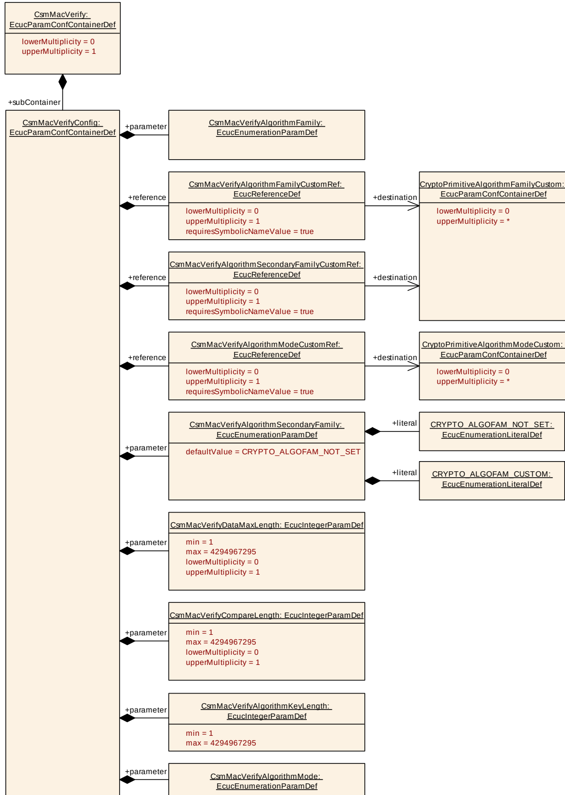
Figure 9-12 CsmMacVerify Layout
