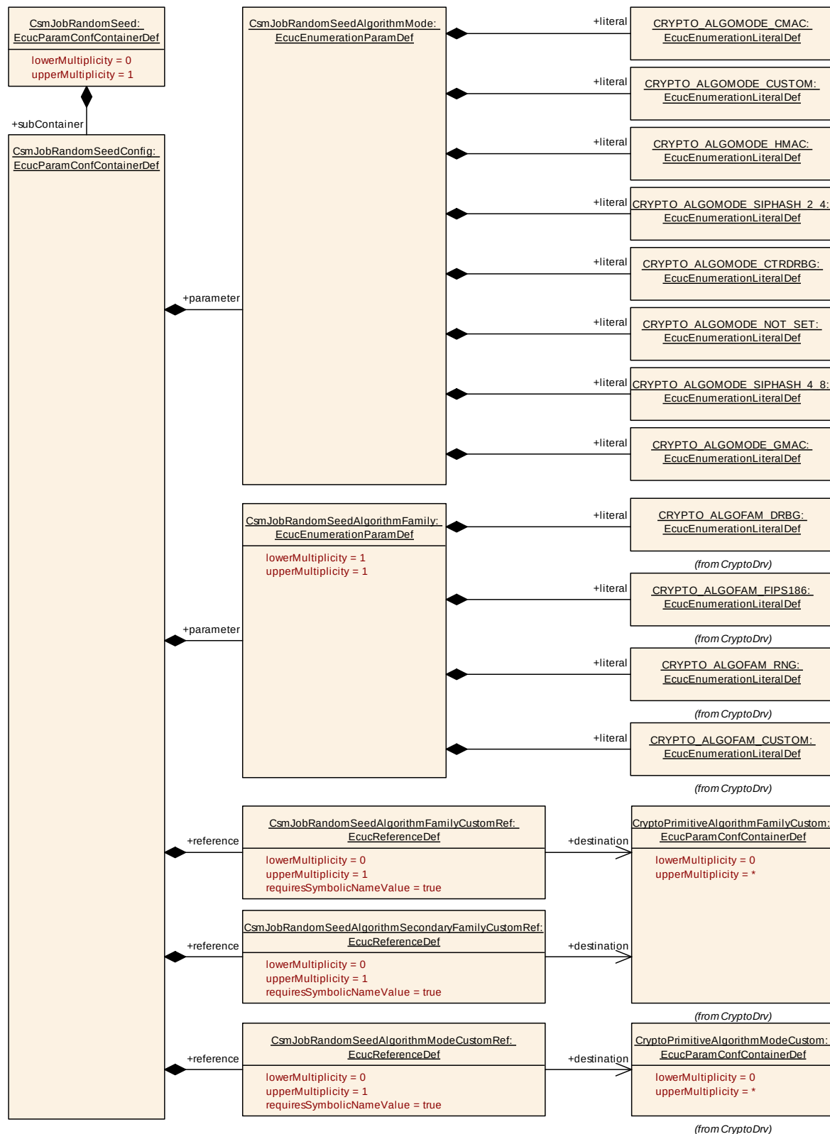
Figure 9-24 CsmJobRandomSeed Layout
