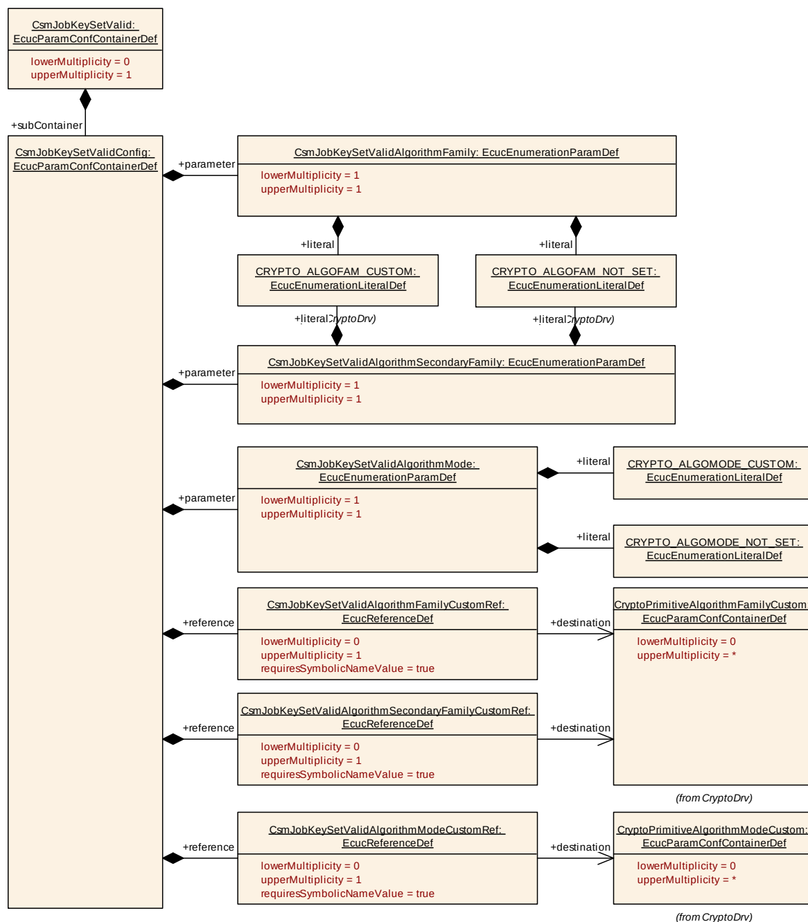
Figure 9-22 CsmJobKeySetValid Layout
