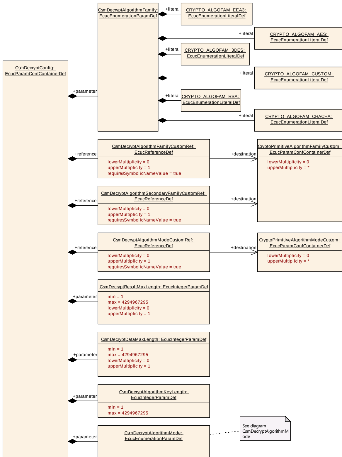
Figure 9-15 CsmDecrypt Layout
