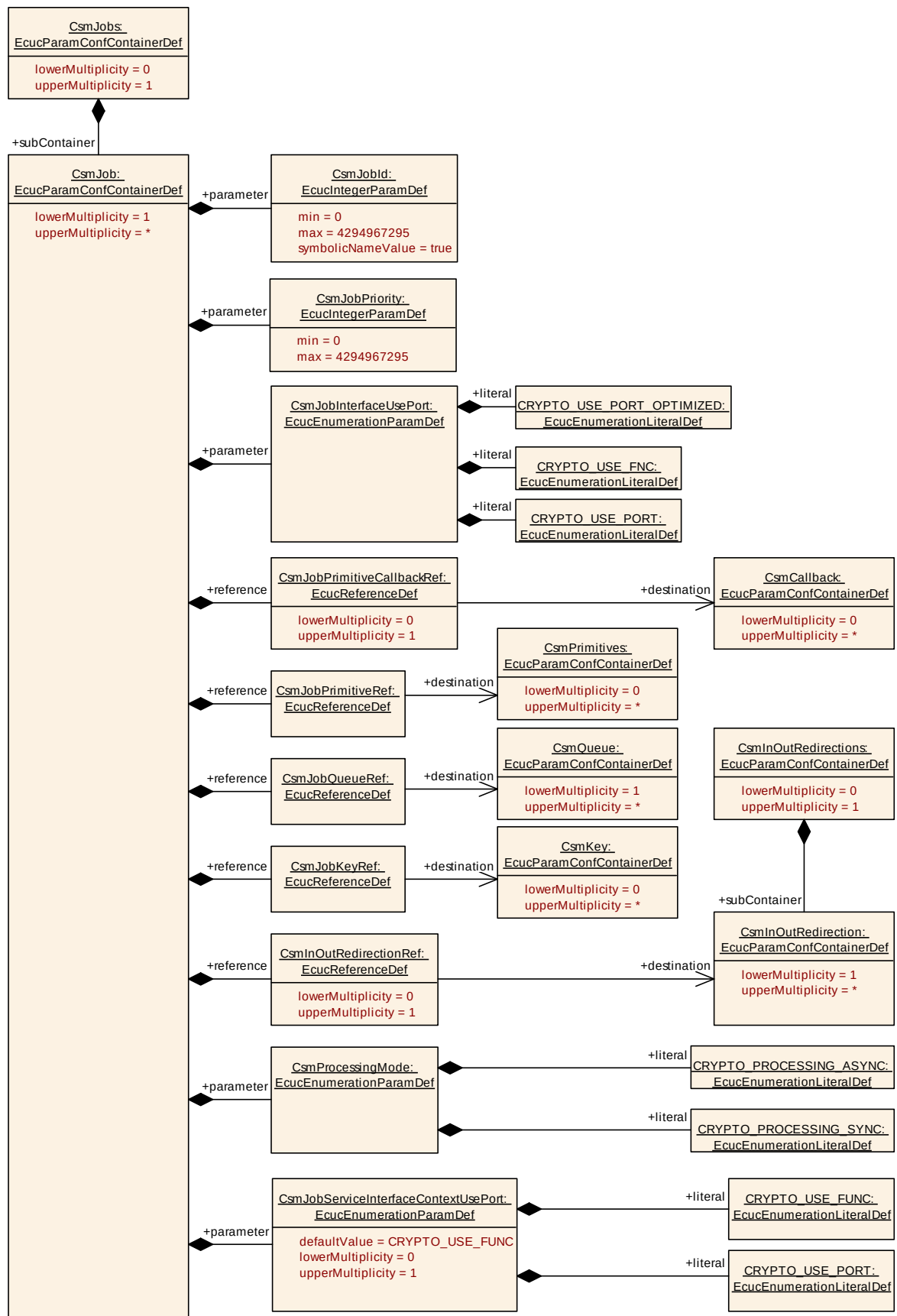
Figure 9-6 CsmJobs Layout
