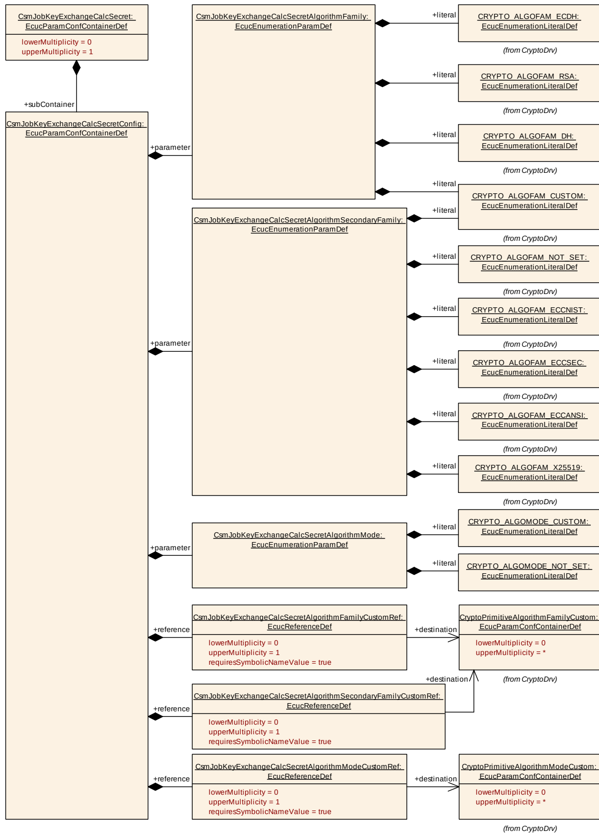
Figure 9-28 CsmJobKeyExchangeCalcSecret Layout
