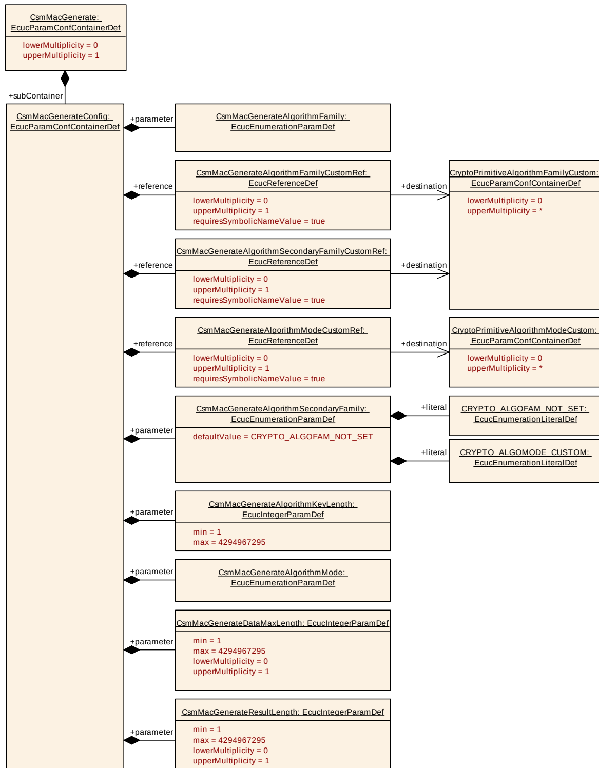
Figure 9-11 CsmMacGenerate Layout
