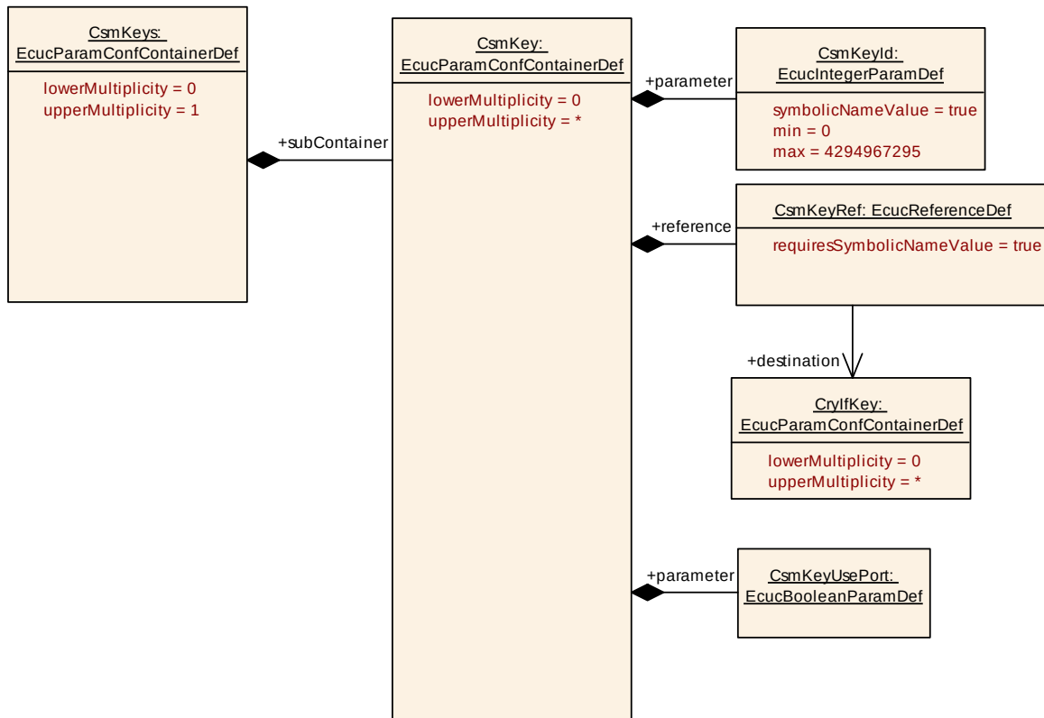
Figure 9-7 Crypto Service Manager Keys Layout
