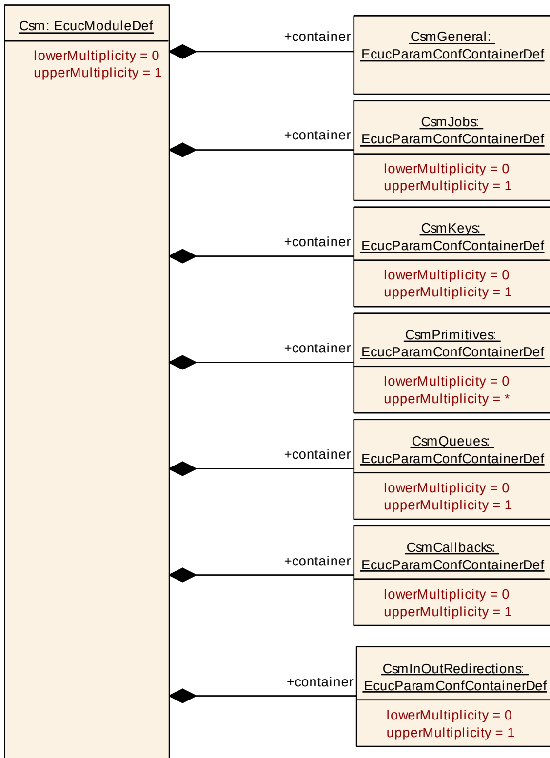
Figure 9-3 Crypto Service Manager Layout
