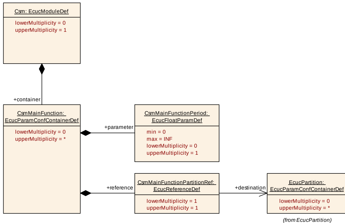
Figure 9-5 Crypto Service Manager MainFunction Layout
