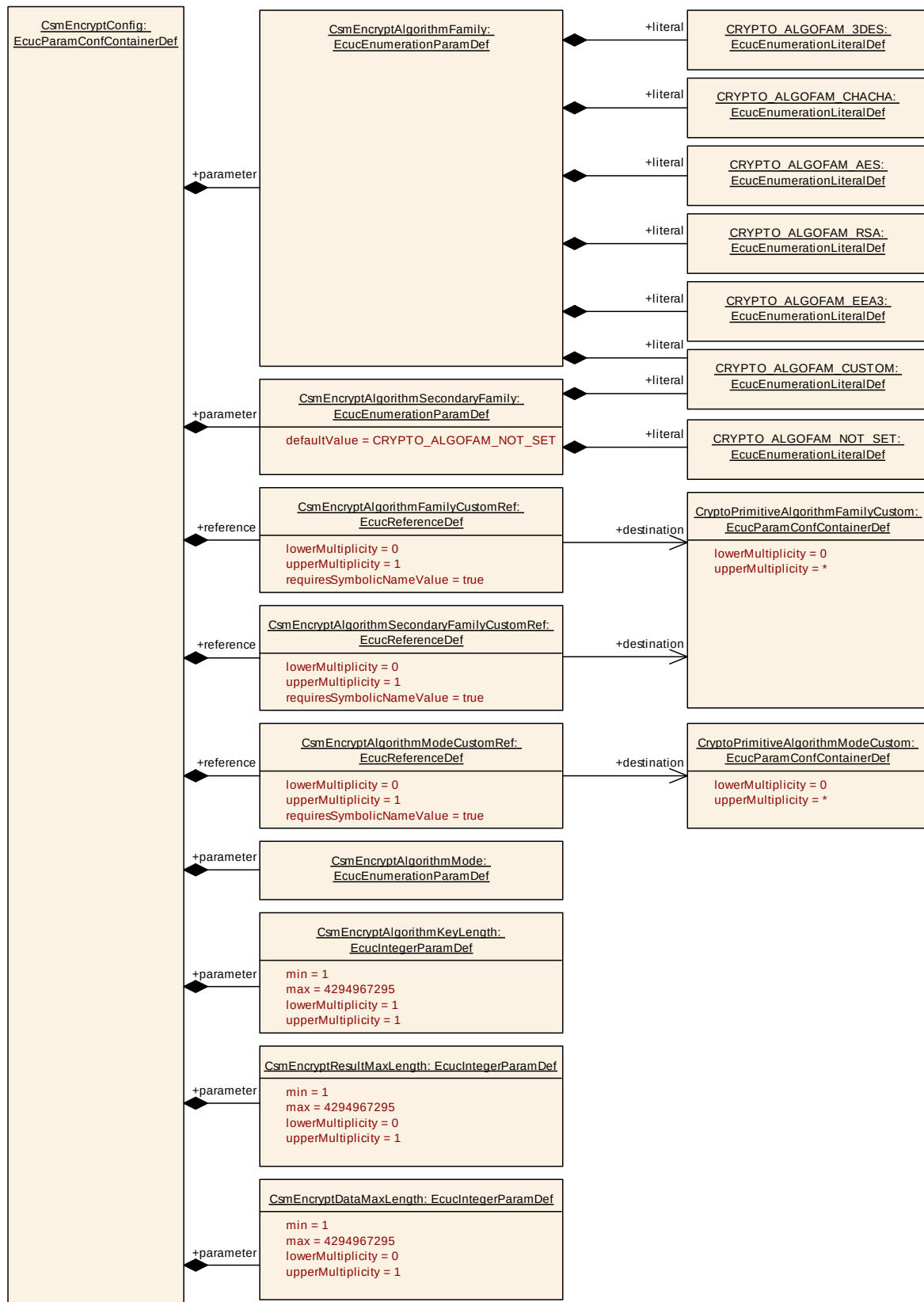
Figure 9-13 CsmEncrypt Layout
