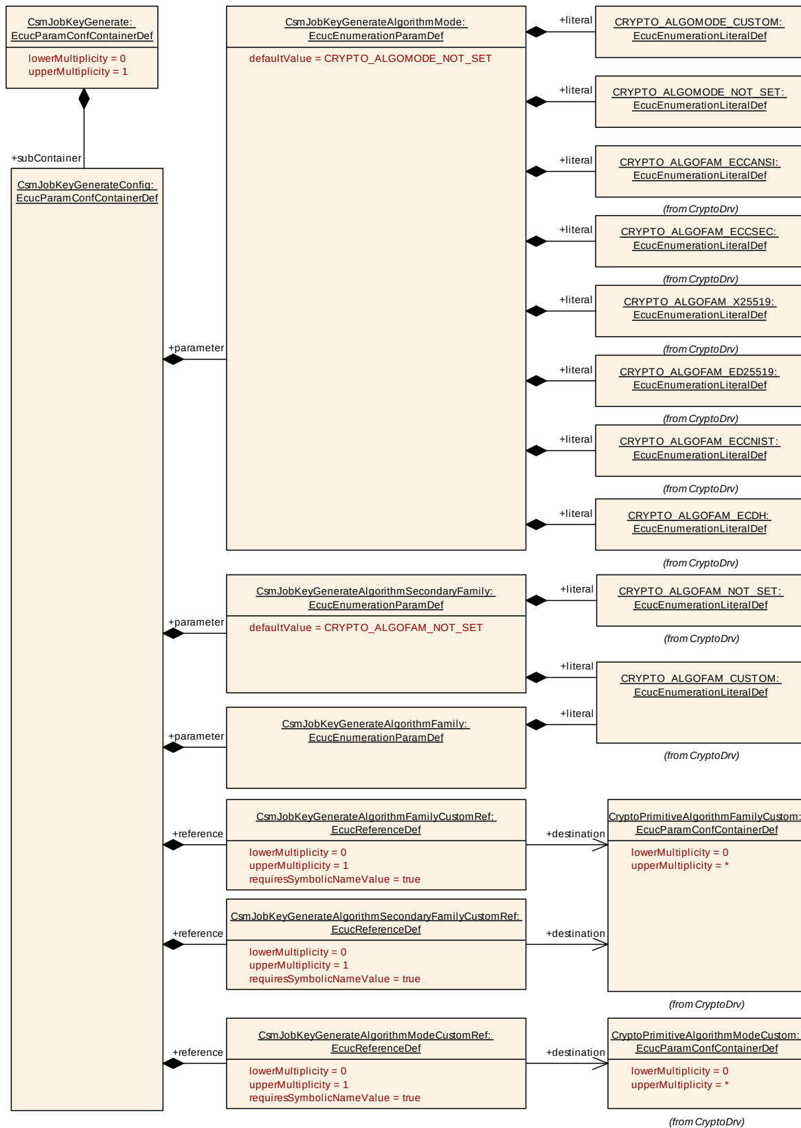
Figure 9-26 CsmJobKeyGenerate Layout
