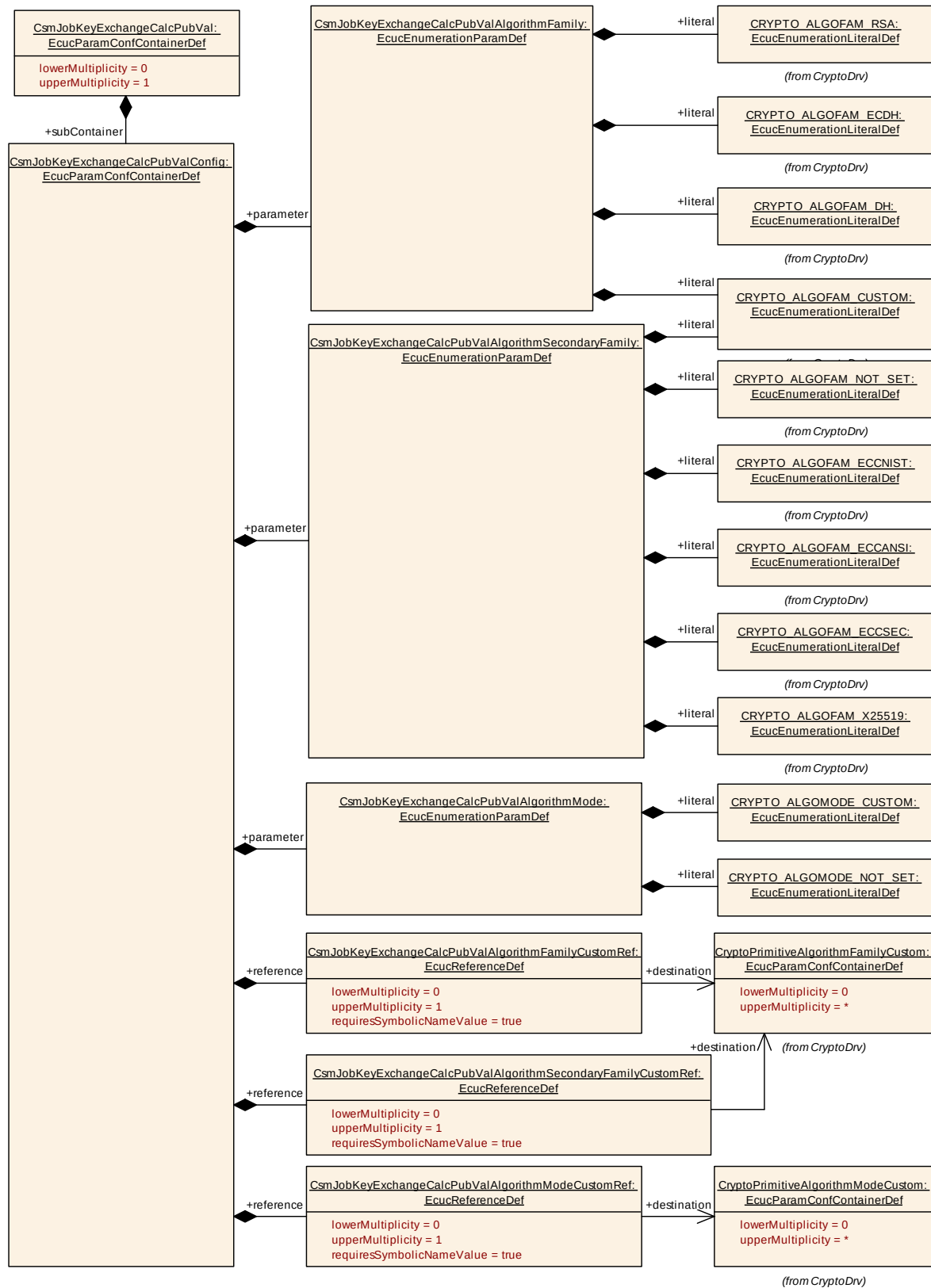
Figure 9-27 CsmJobKeyExchangeCalcPubVal Layout
