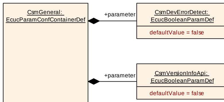
Figure 9-4 Crypto Service Manager General Layout
