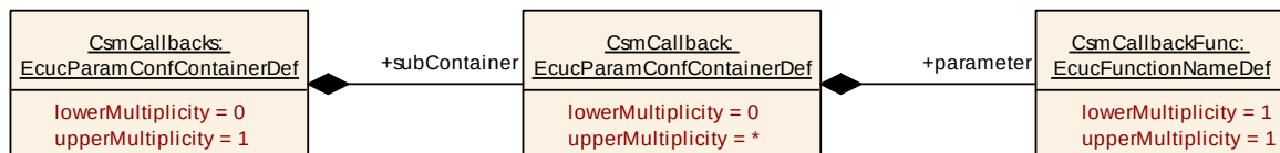
Figure 9-29 CsmCallbacks Layout
