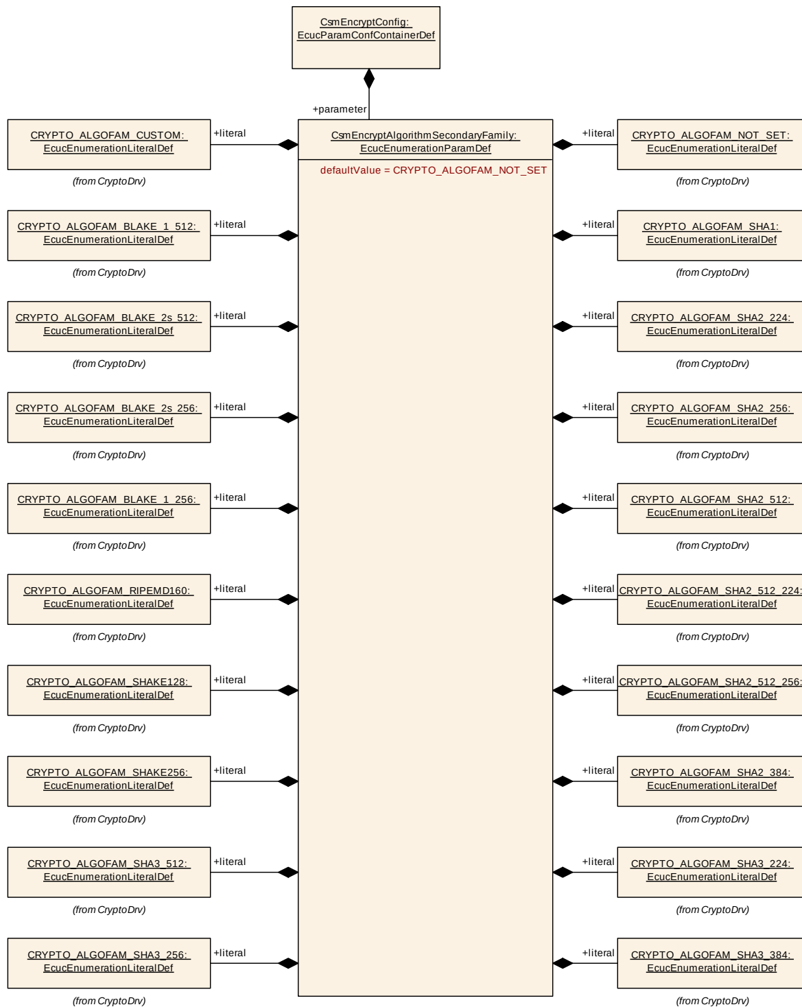
Figure 9-14 CsmEncryptAlgorithmSecondaryFamily Layout
