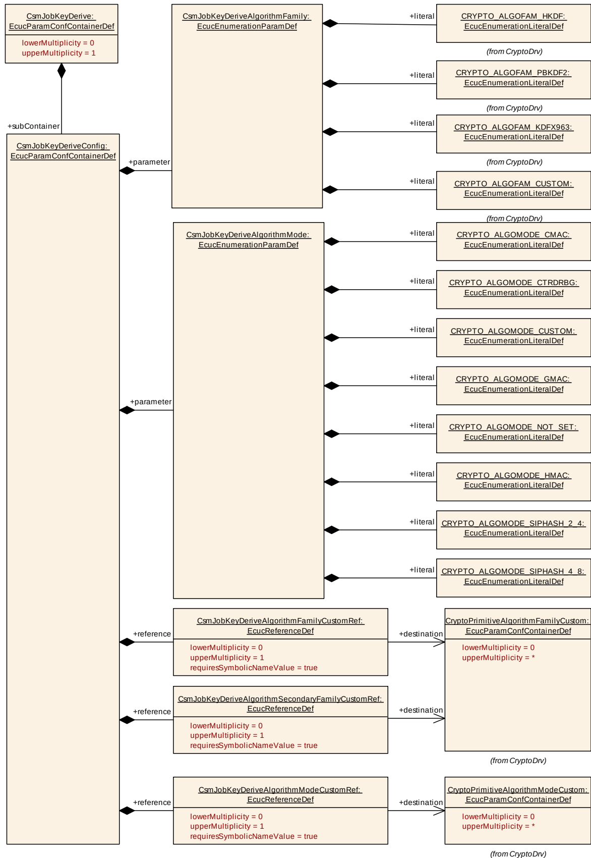
Figure 9-25 CsmJobKeyDerive Layout
