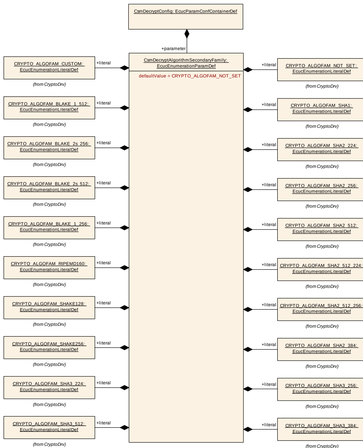
Figure 9-16 CsmDecryptAlgorithmSecondaryFamily Layout
