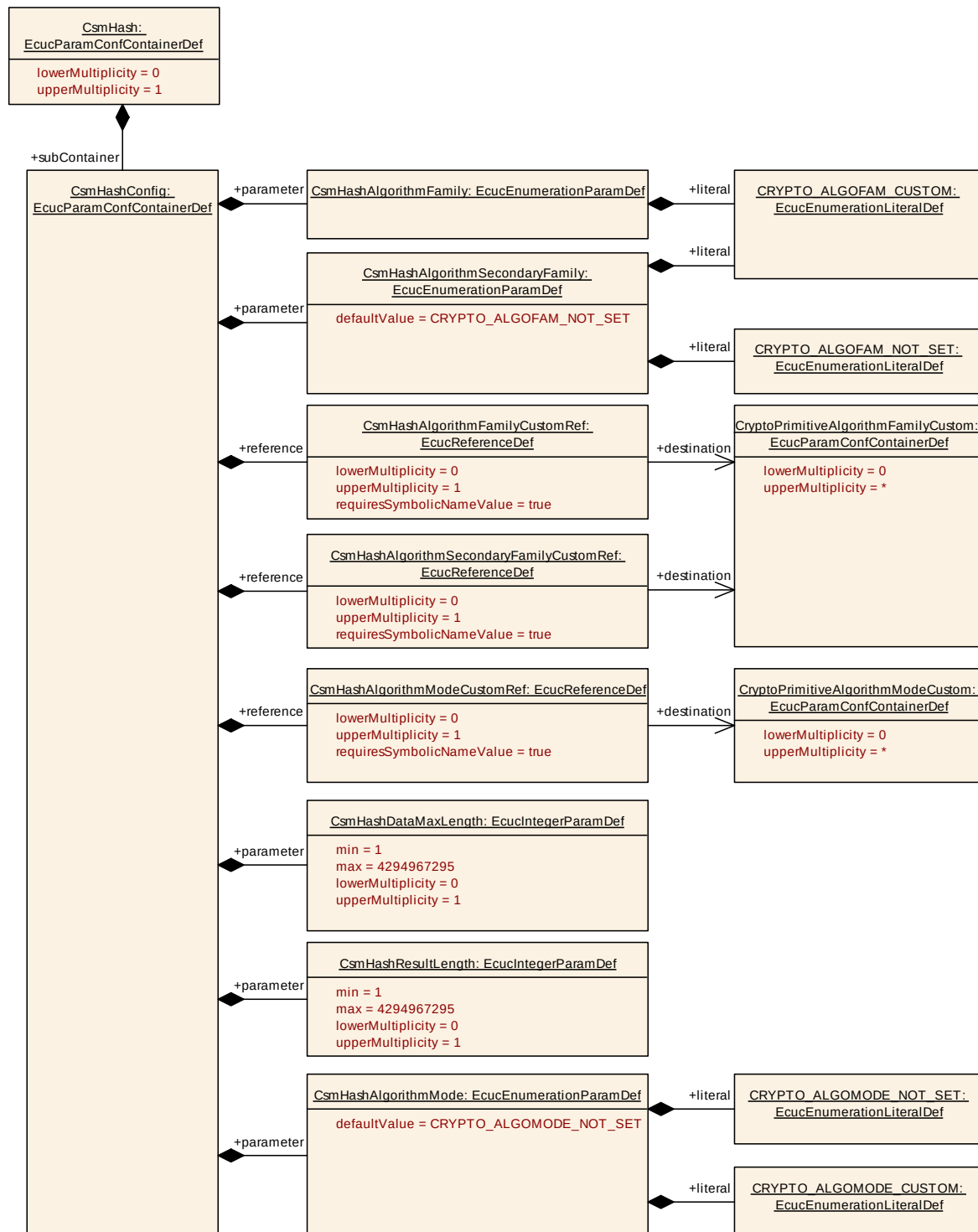
Figure 9-10 CsmHash Layout
