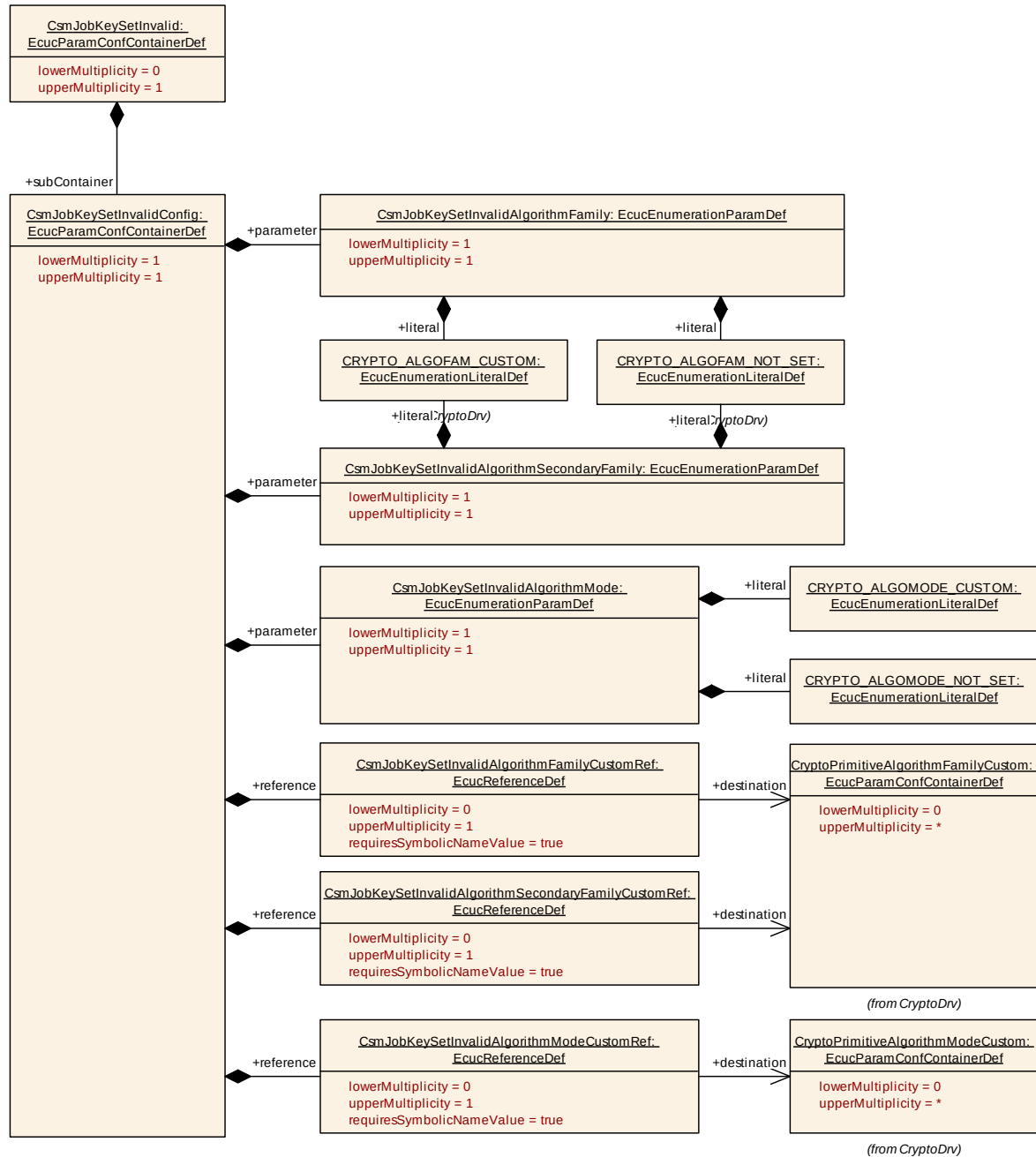
Figure 9-23 CsmJobKeySetInvalid Layout
