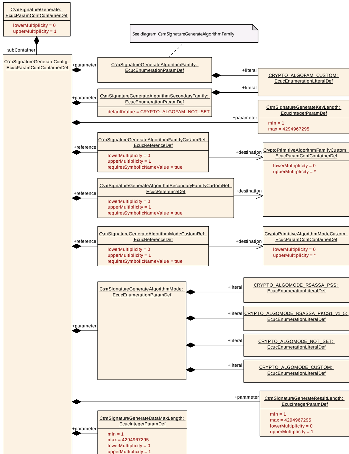
Figure 9-19 CsmSignatureGenerate Layout
