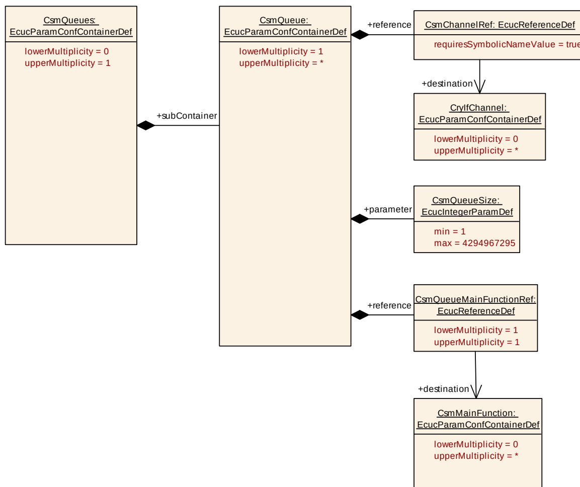
Figure 9-8 Crypto Service Manager Queues Layout
