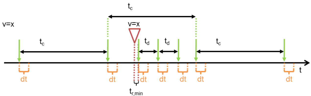
Figure 15: Use case 5 scenario a, TM MIXED , here n = 2 (without TMS switch)
