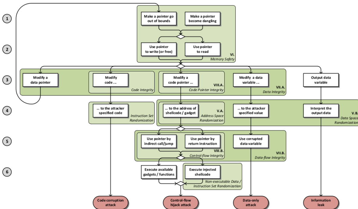
Figure A.1: Attack model from [3] demonstrating four attack types, policies mitigating the attacks in different attack stages
