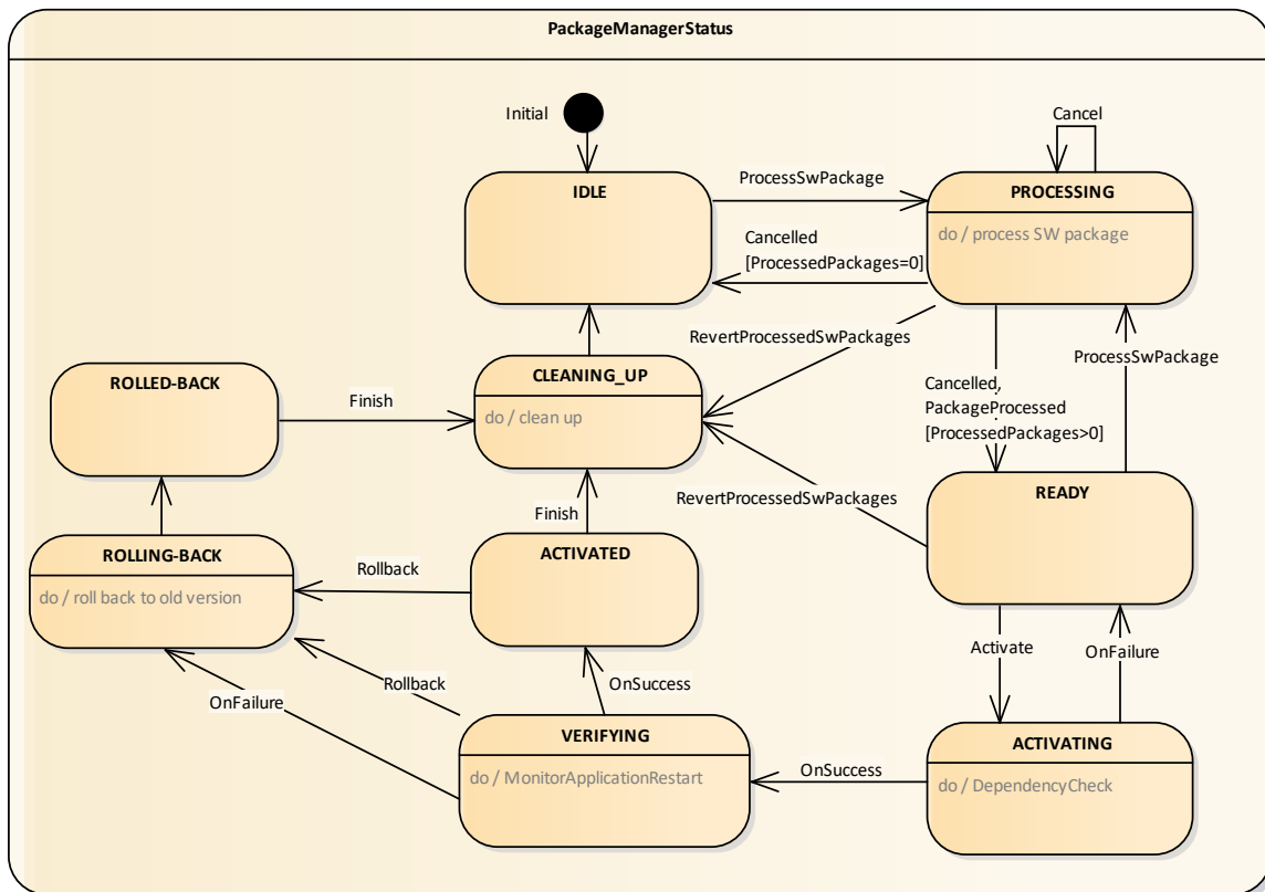
Figure 13-6 Overview Processing and Activation of Software Package
