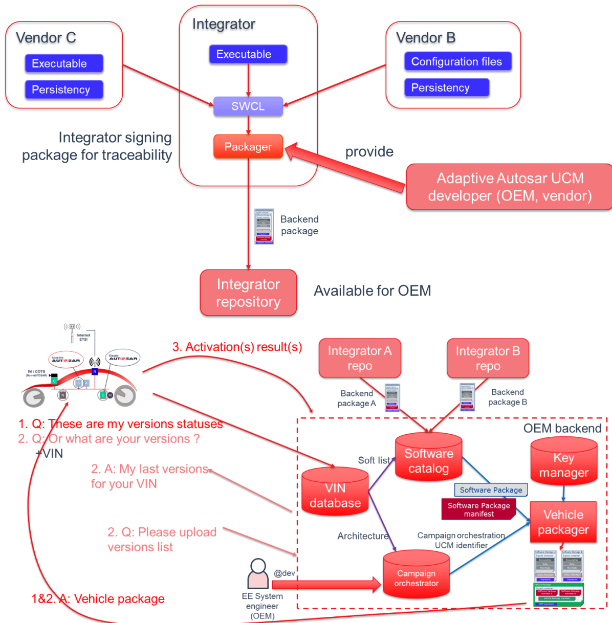
Figure 13-5 Packages distribution to vehicle
