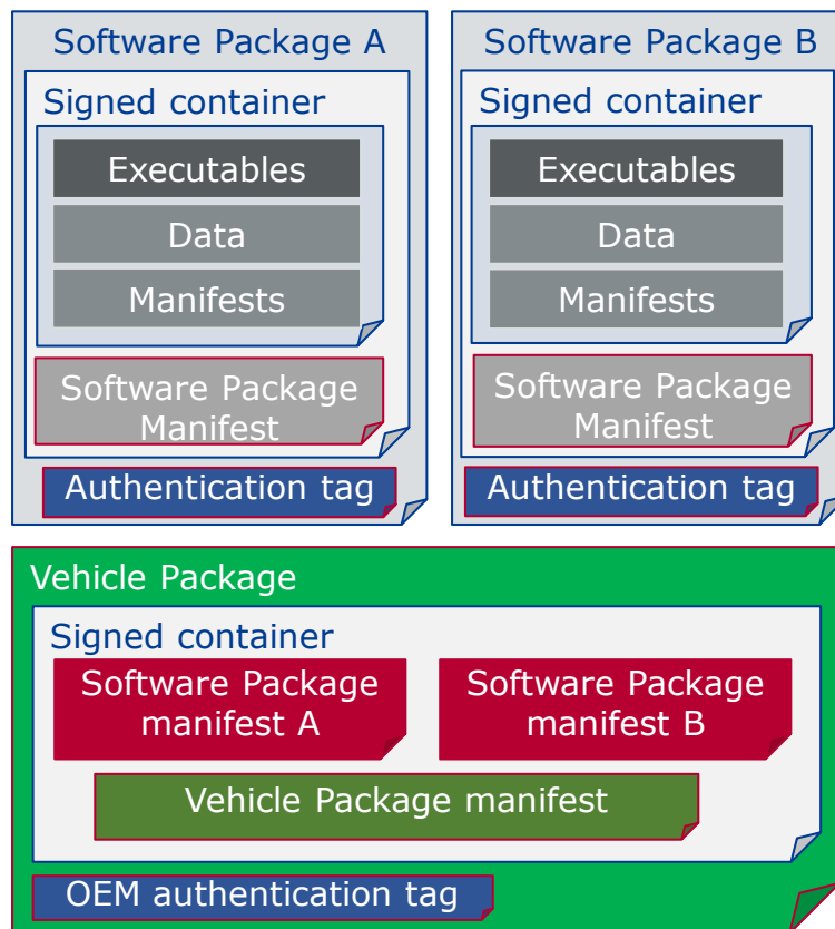
Figure 13-3 Overview Vehicle Package
