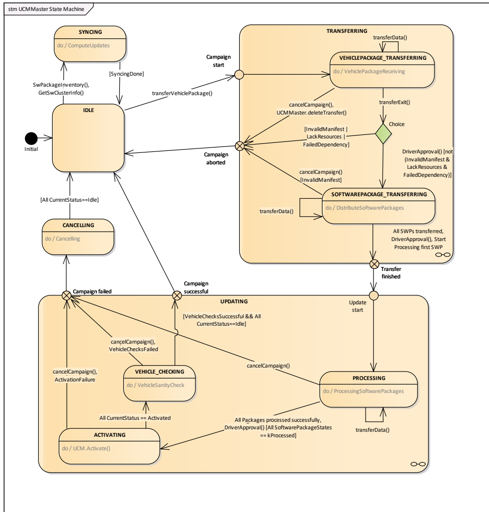
Figure 13-7 UCM Master state machine
