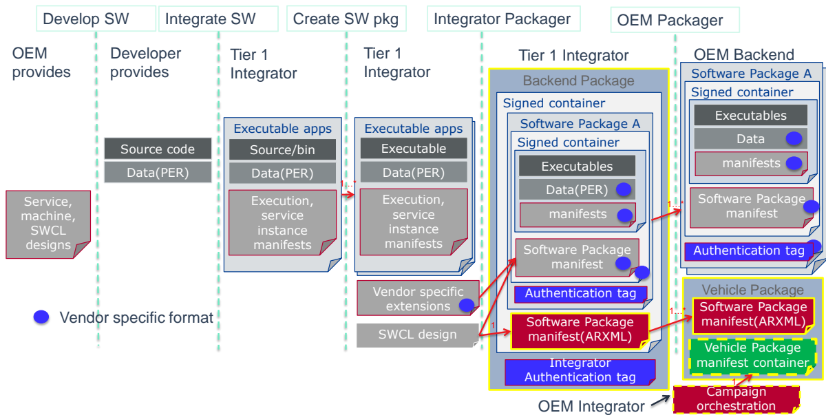
Figure 13-4 Packaging steps
