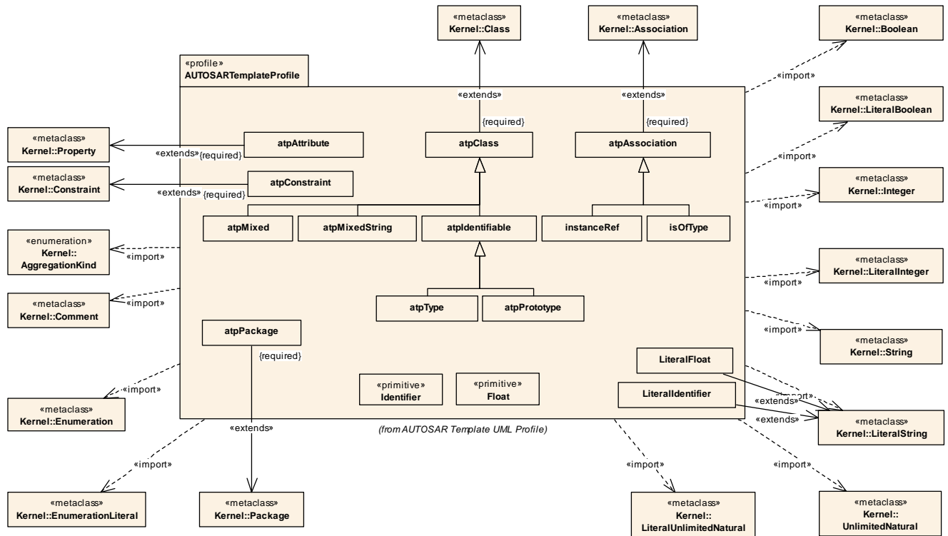
Figure 5-25: Overview of the UML Profile for AUTOSAR Templates.
