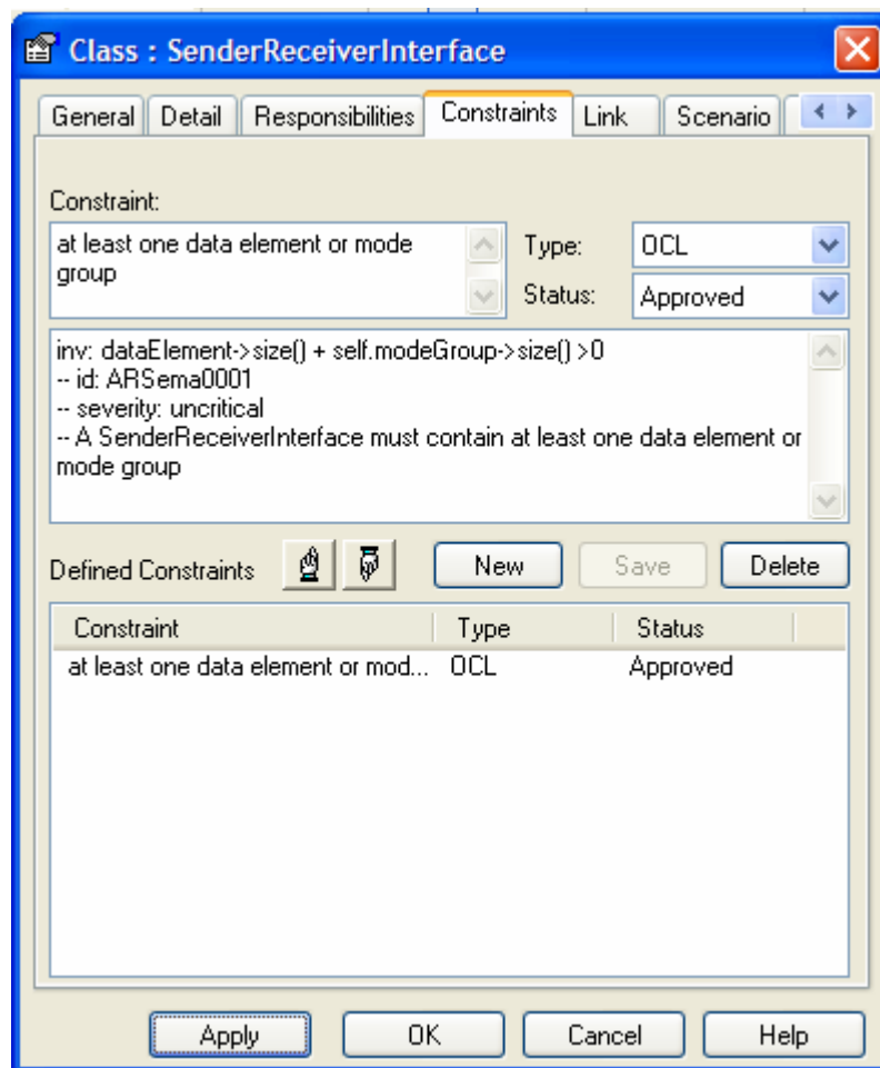
Figure 6-3: Constraint dialog in Enterprise Architect.
