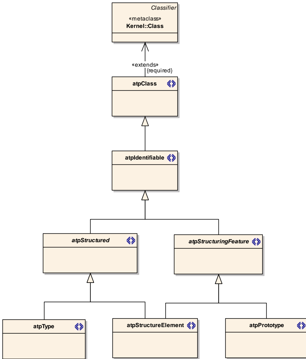
Figure 5-6: New stereotypes for types and prototypes.
