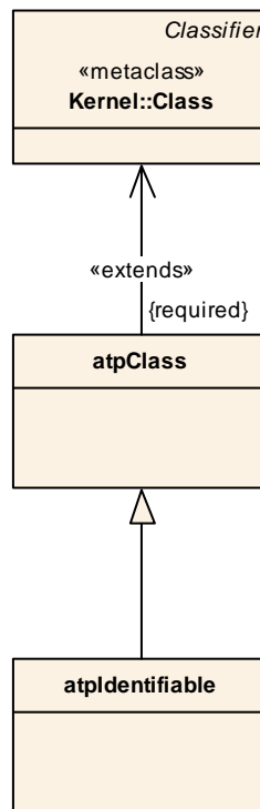
Figure 5-2: Stereotypes atpClass and atpIdentifiable .
