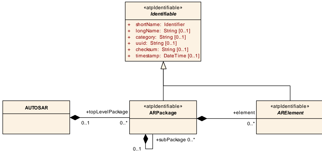
Figure 7-1: Infrastructure of an AUTOSAR template model.
