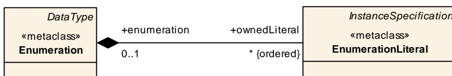
Figure 5-24: Definition of enumerations in UML 2.
