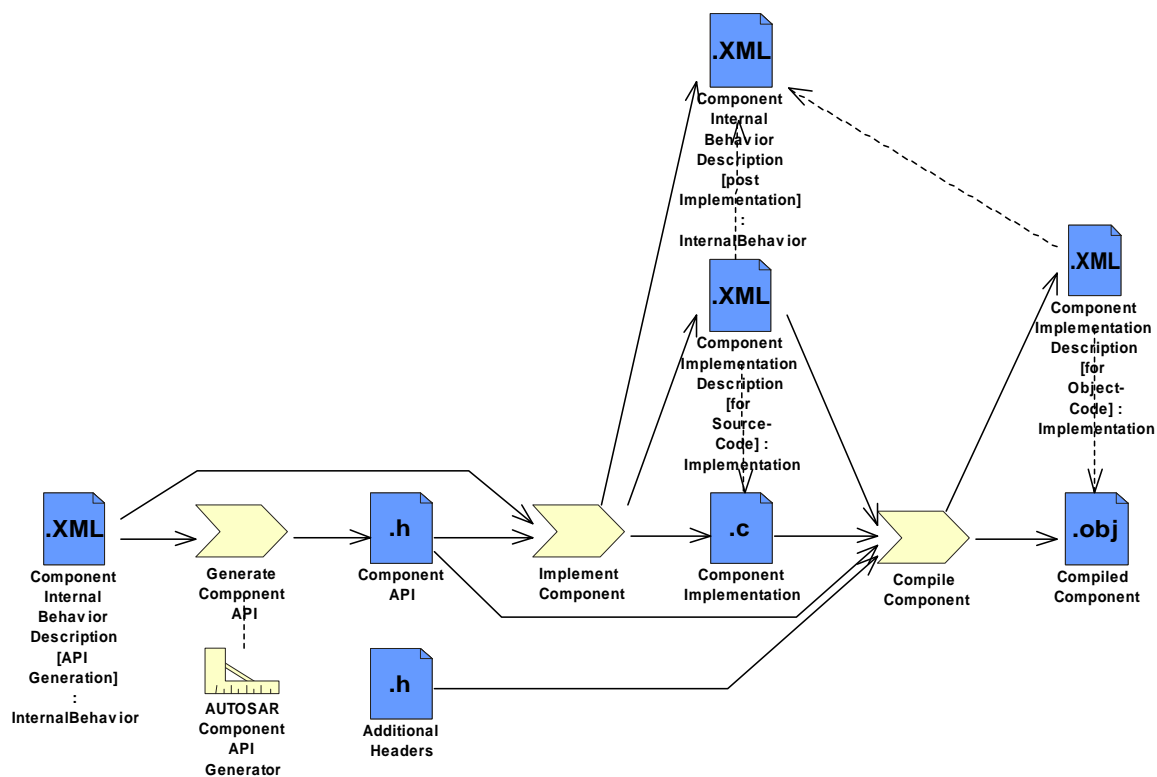
Figure 13: Component implementation part of the AUTOSAR Methodology
