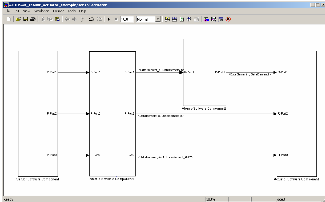
Figure 4: Sensor and Actuator Software Components communicating with application software components
