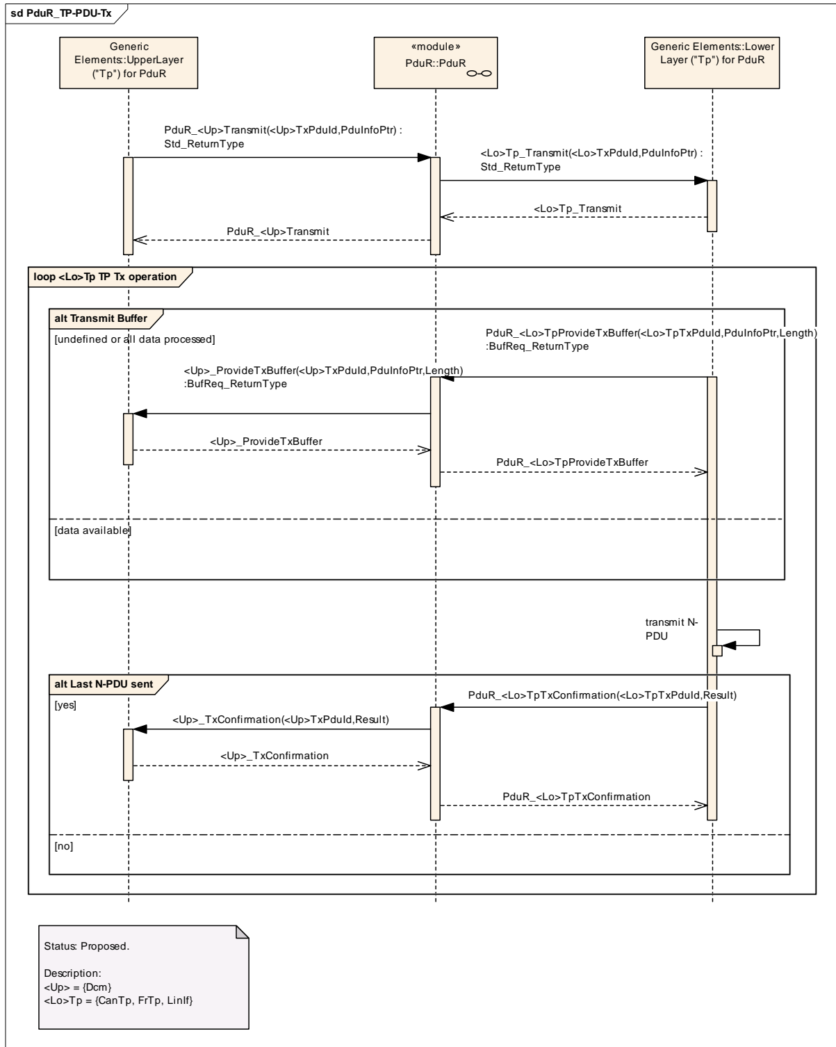
Figure 11: TP-PDU-Tx
