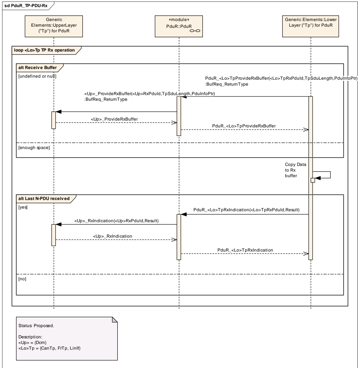
Figure 7: TP-PDU-Rx
