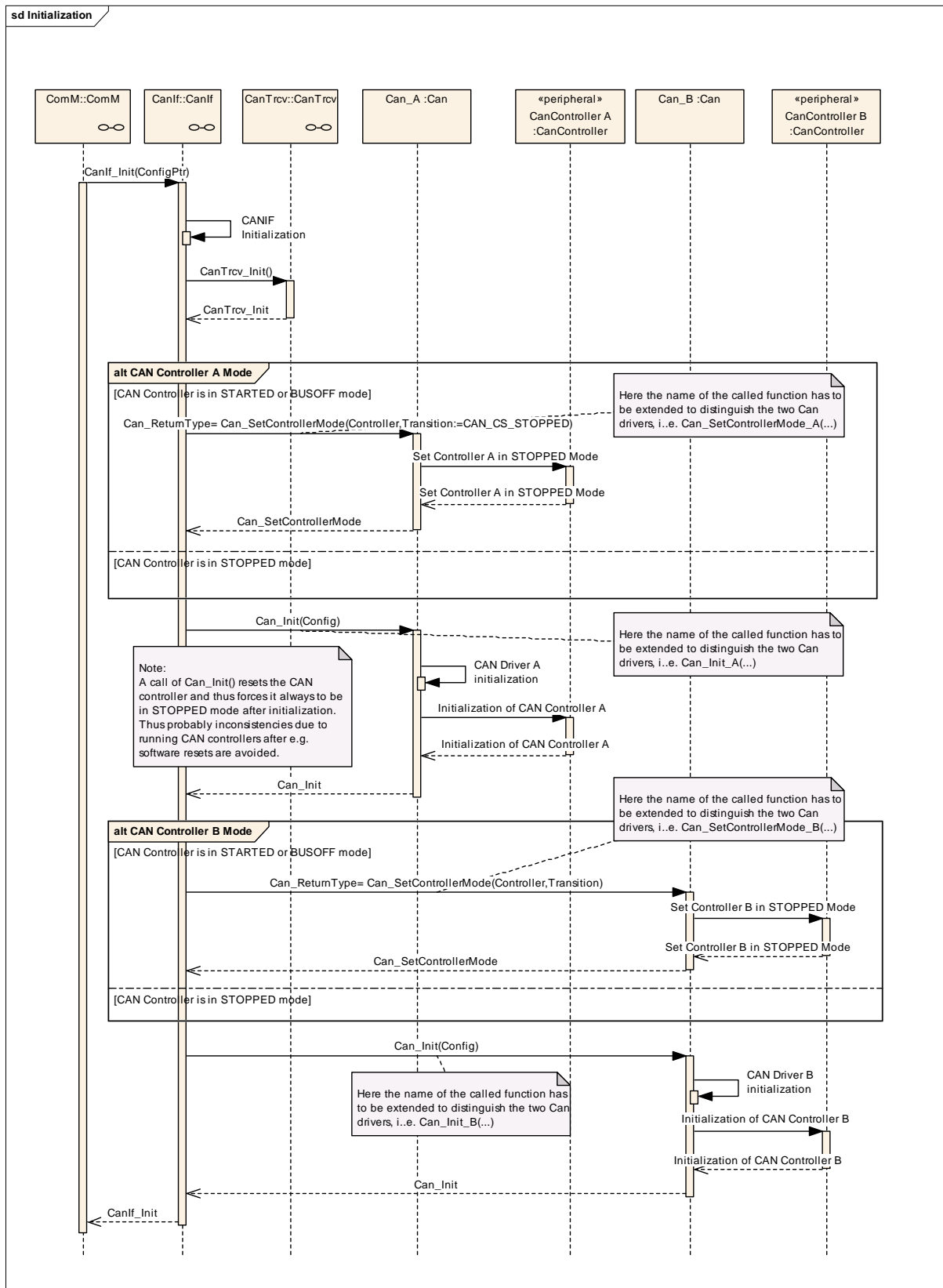
Figure 29 Initialization
