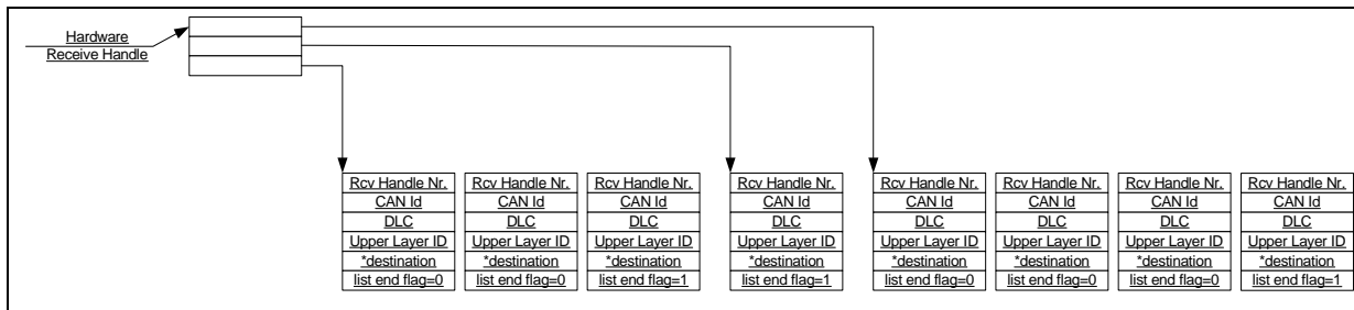
Figure 16 Software filtering example
