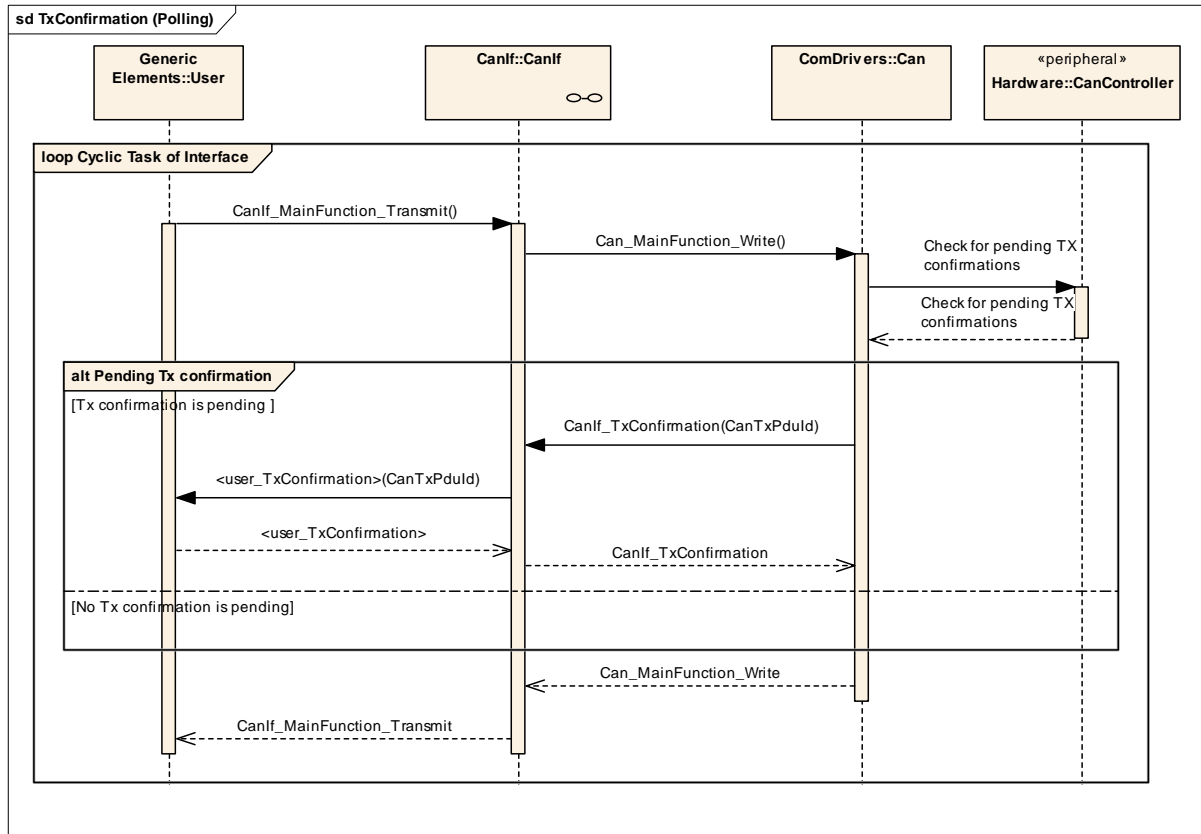
Figure 23 Transmit confirmation polling driven
