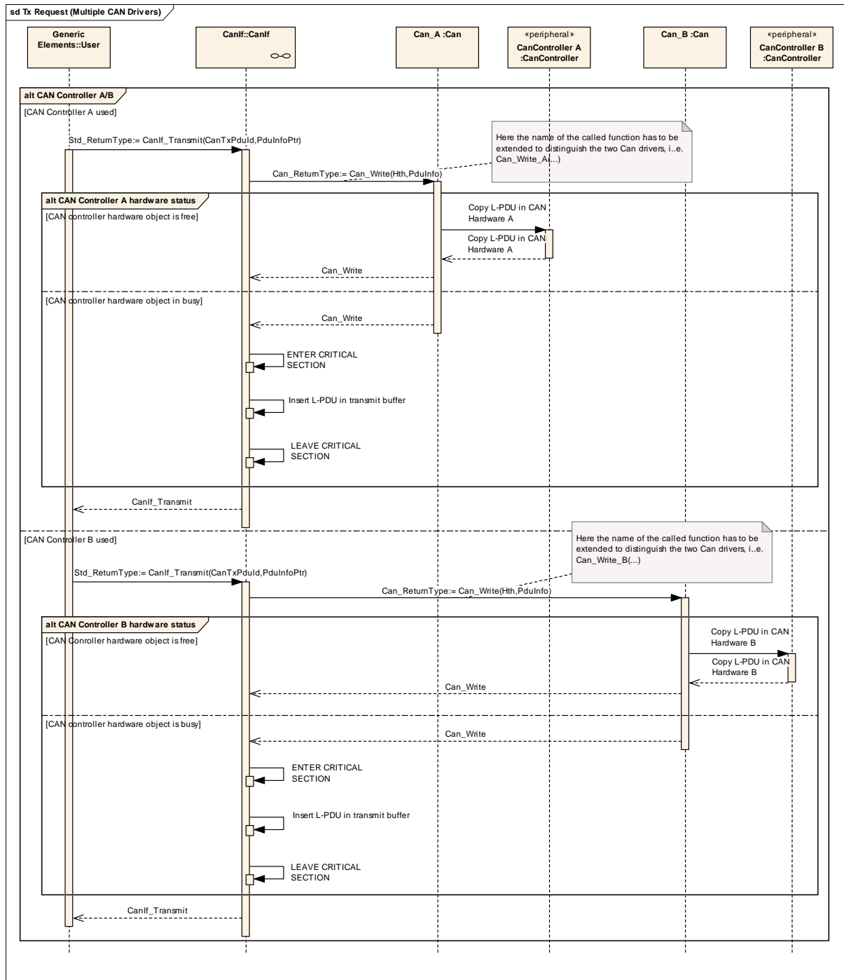
Figure 21 Transmission request with multiple CAN Drivers
