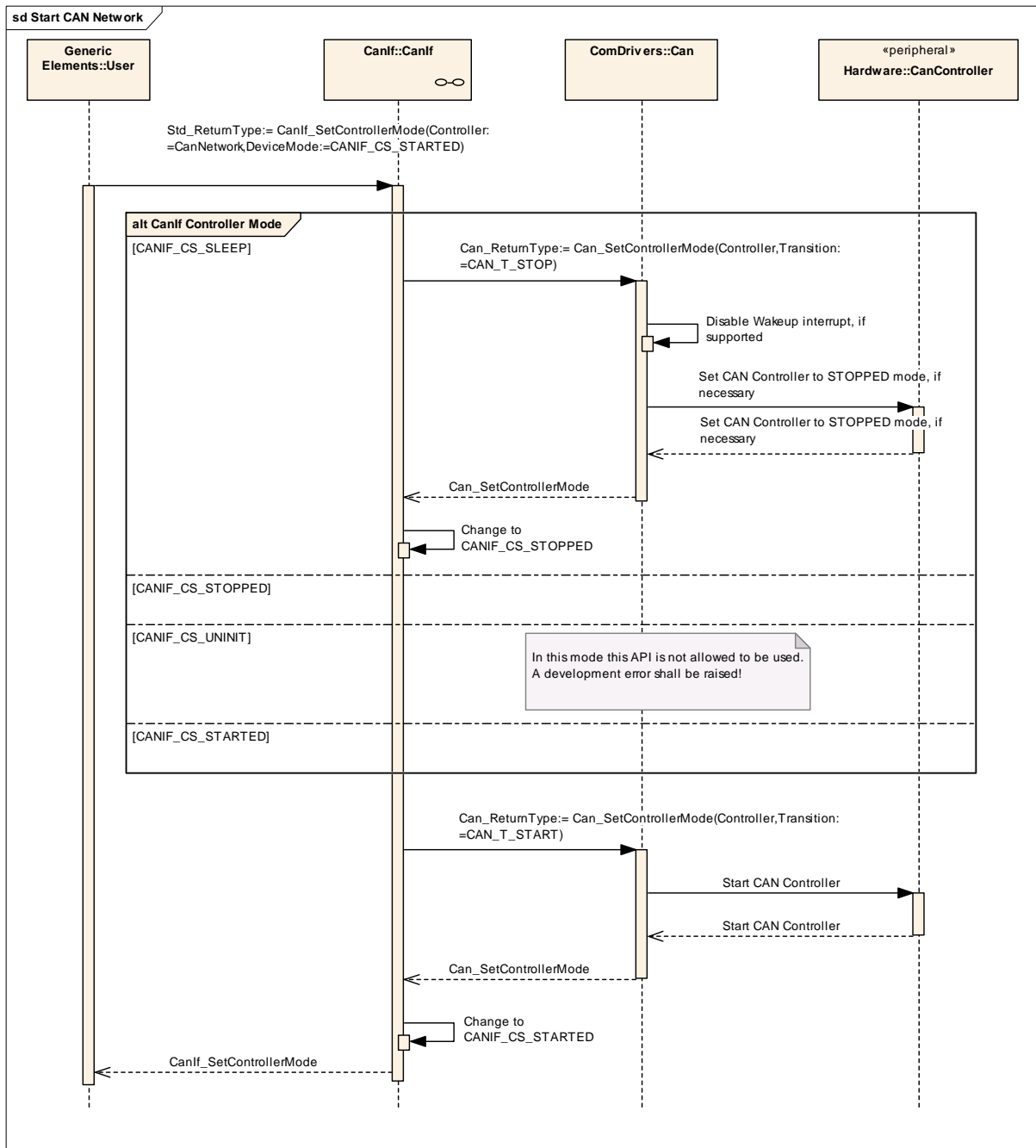
Figure 30 Start CAN network
