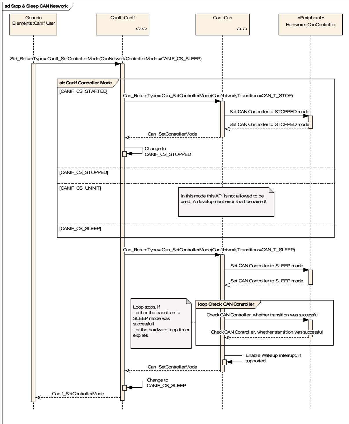
Figure 31 Stop CAN network
