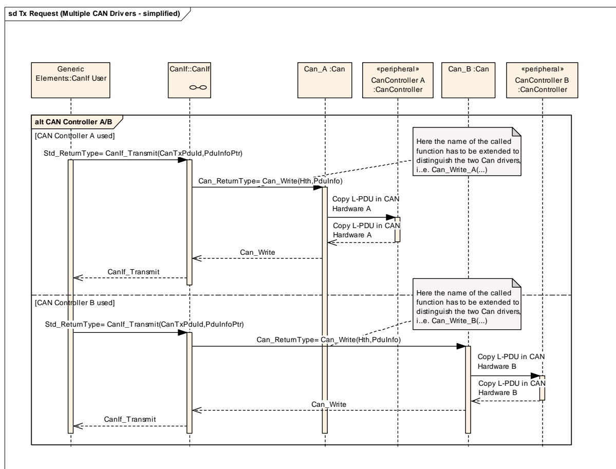
Figure 17 Transmission request with multiple CAN Drivers - simplified
