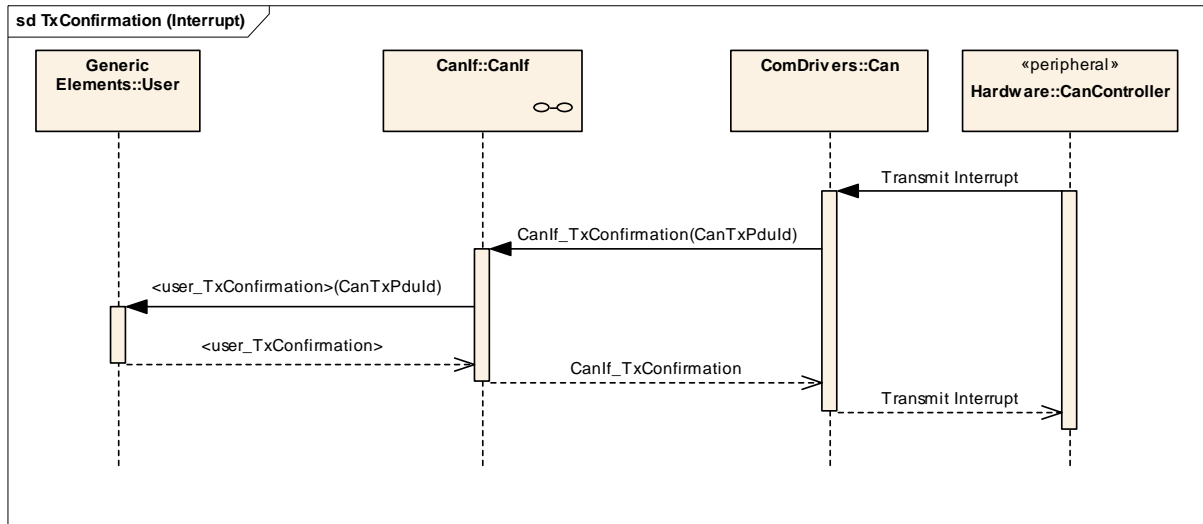
Figure 22 Transmit confirmation interrupt driven
