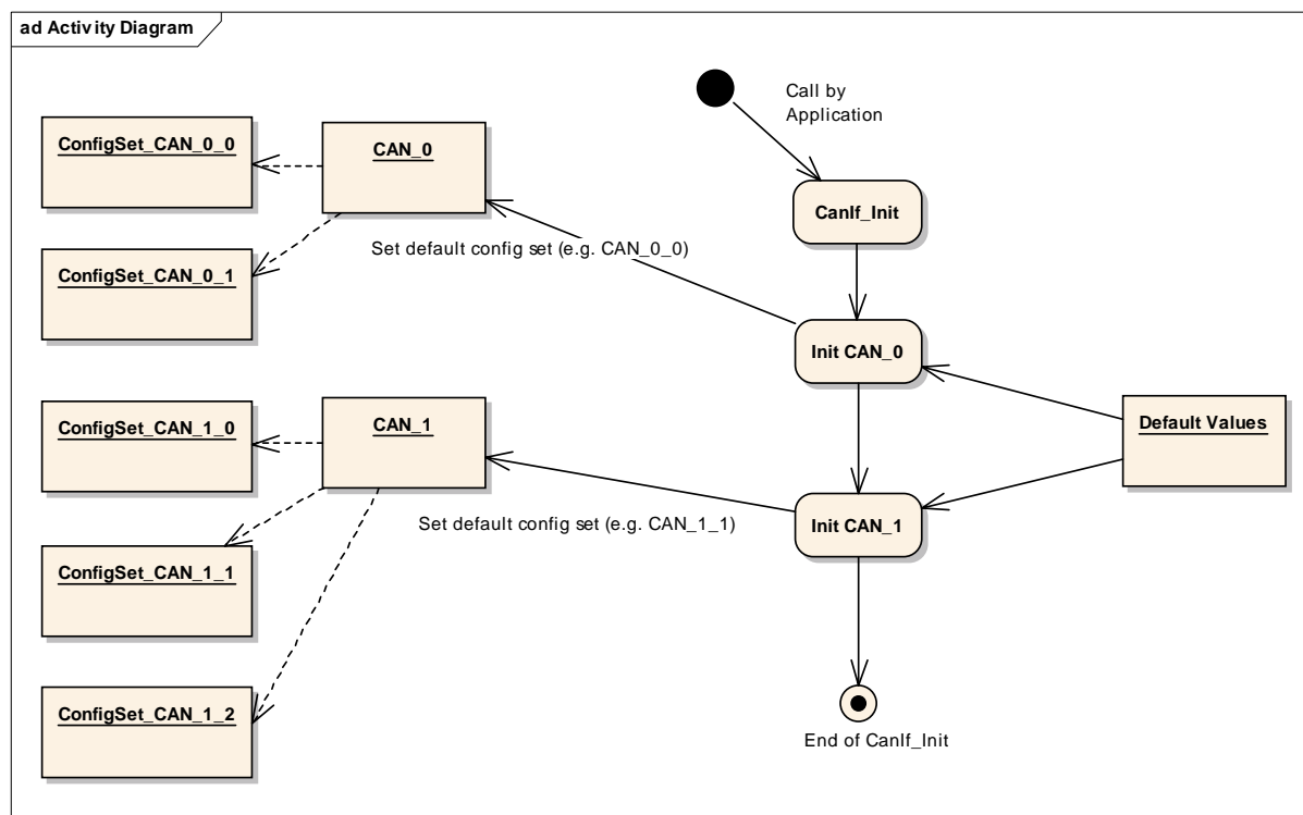
Figure 7 Initialization of CAN Interface and CAN Driver
