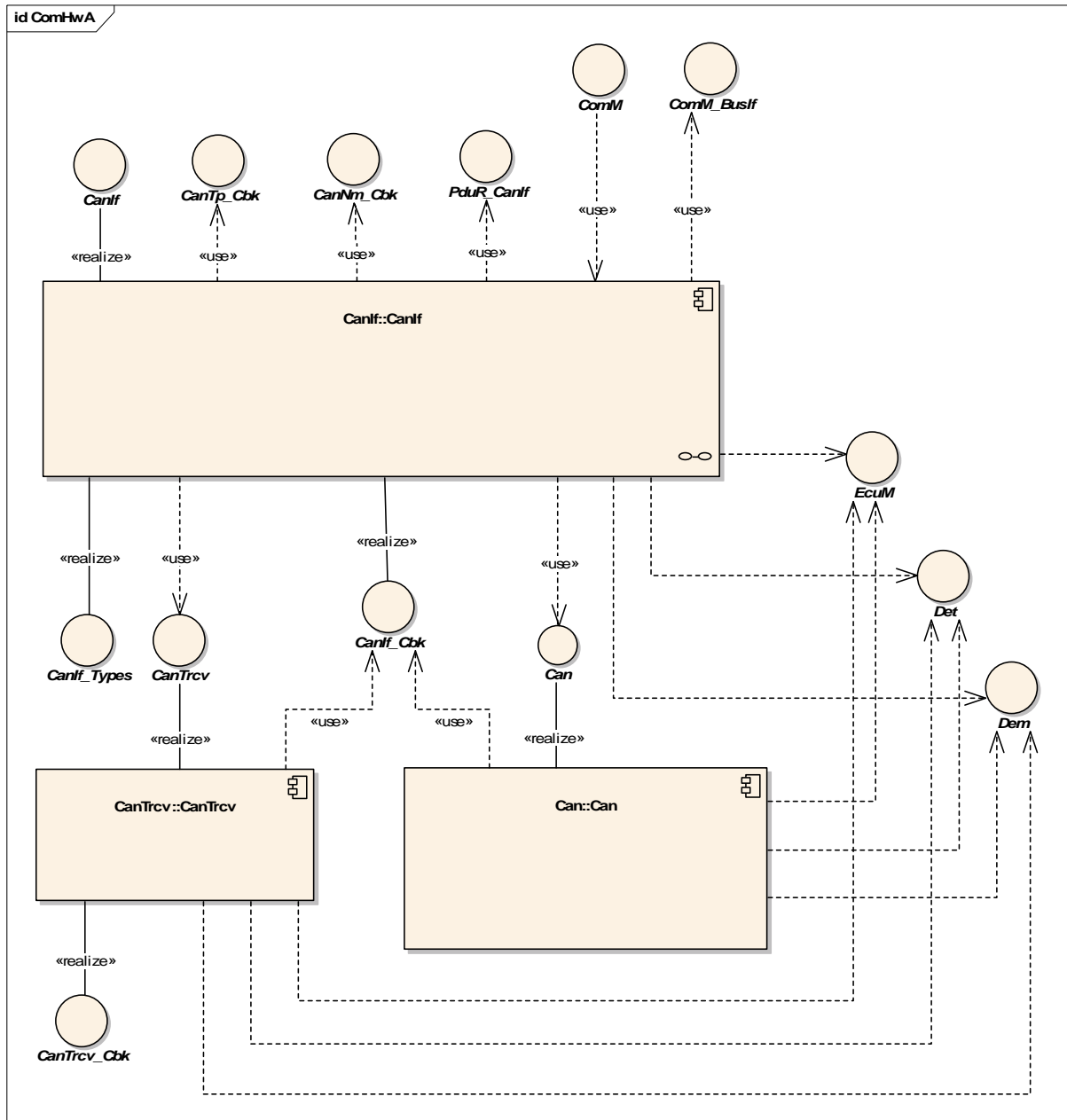
Figure 2 CANIF dependencies in AUTOSAR BSW)
