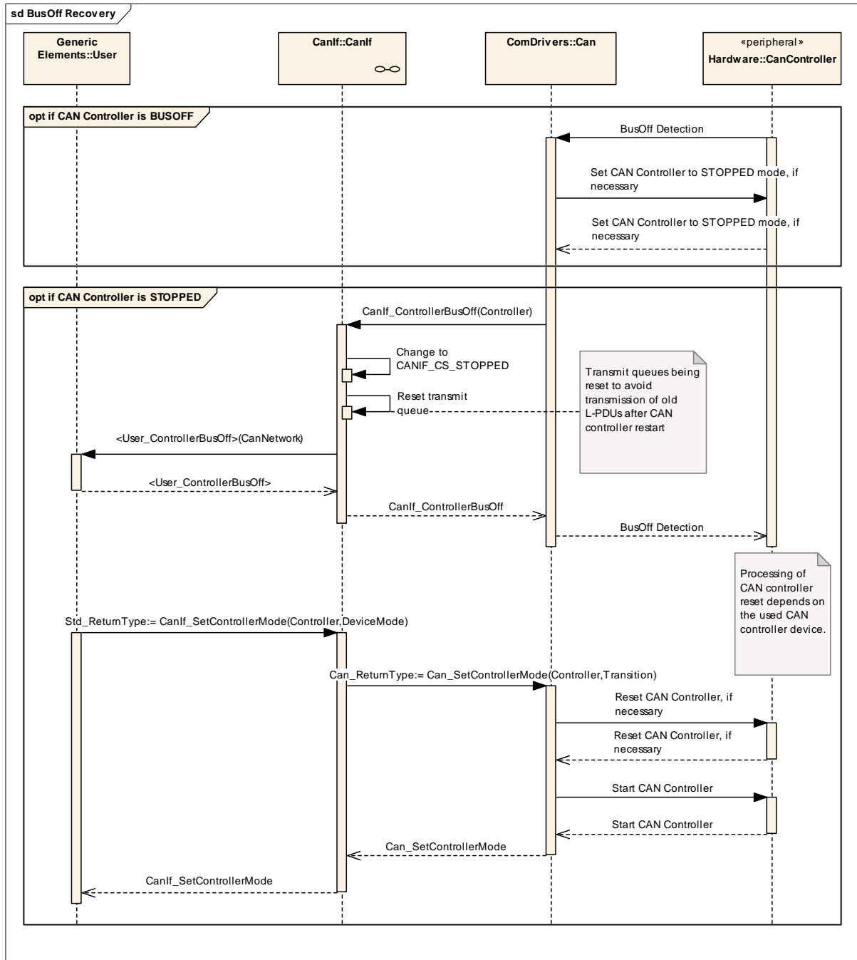
Figure 33 BusOff recovery
