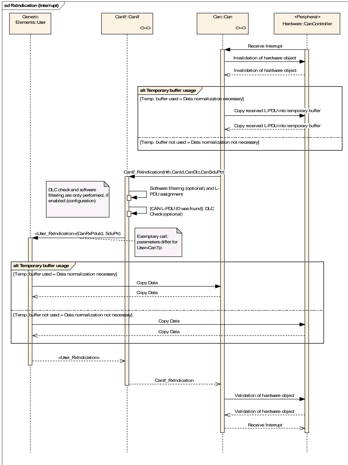
Figure 26 Receive indication interrupt driven
