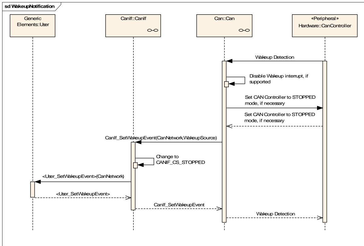
Figure 34 Wakeup notification
