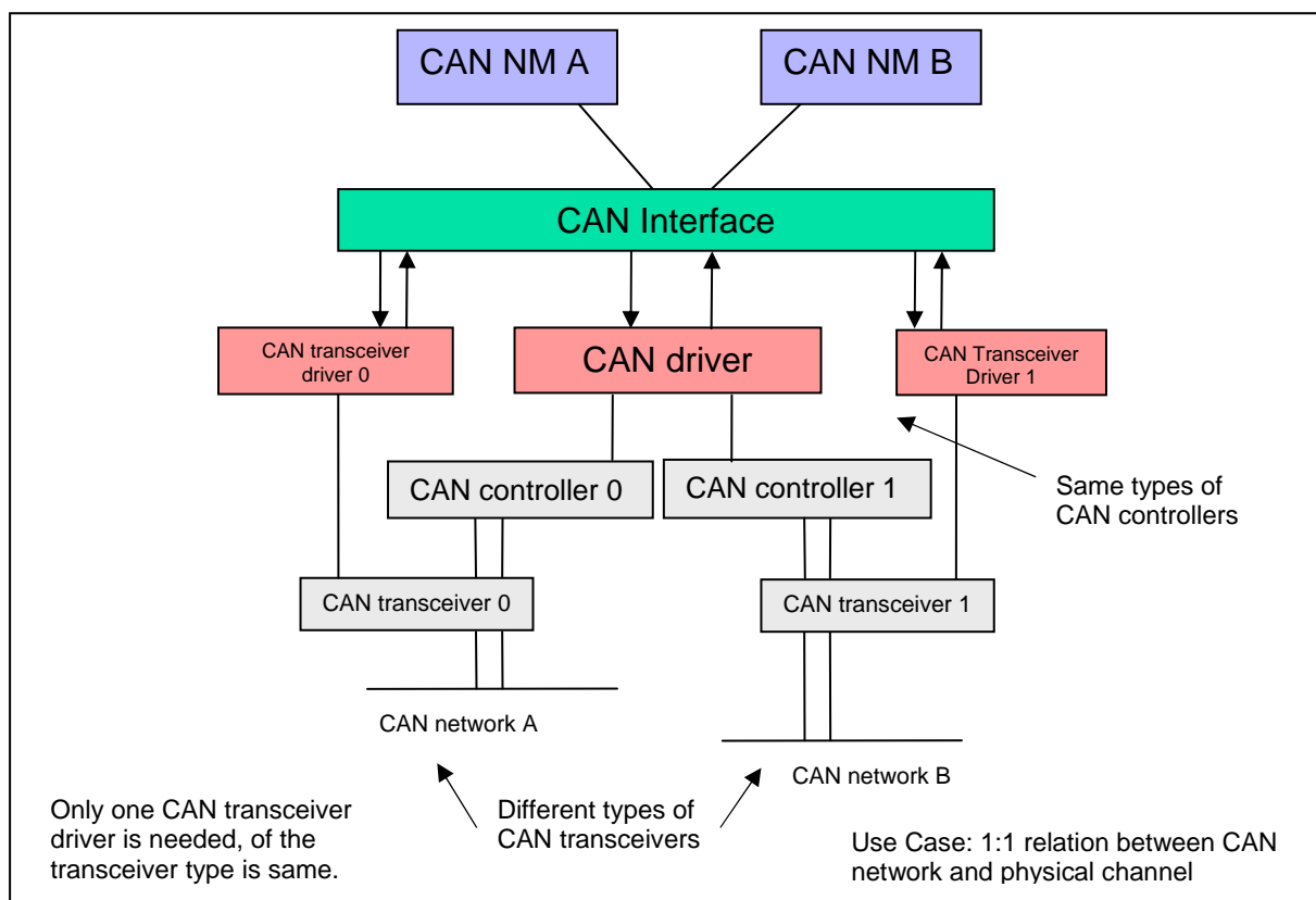
Figure 4: Network view definition example A
