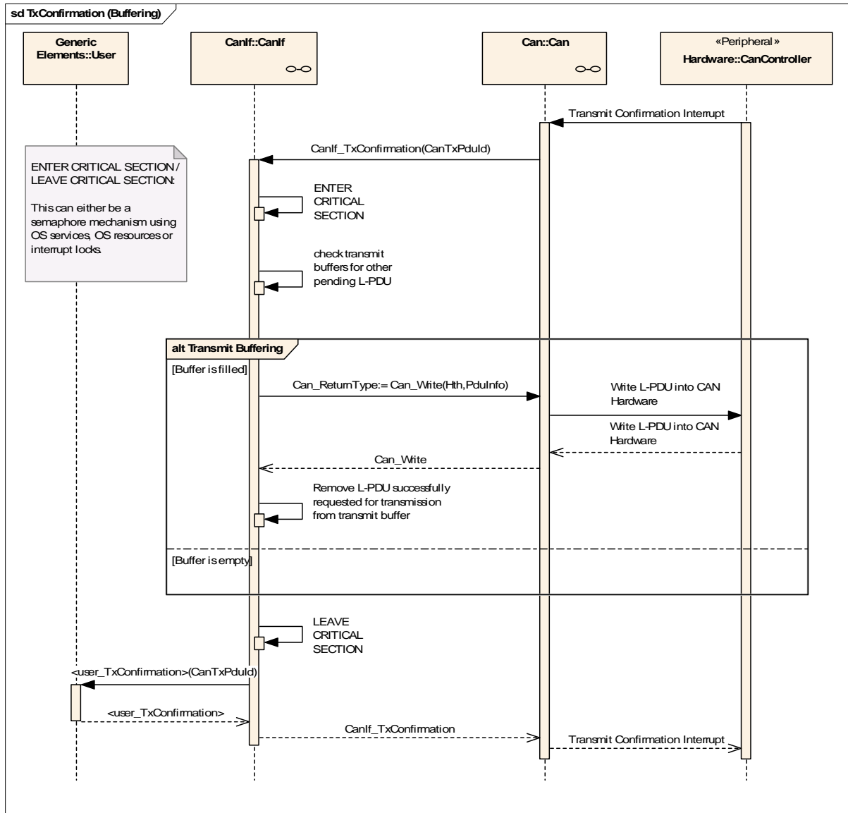
Figure 24 Transmit confirmation with buffering
