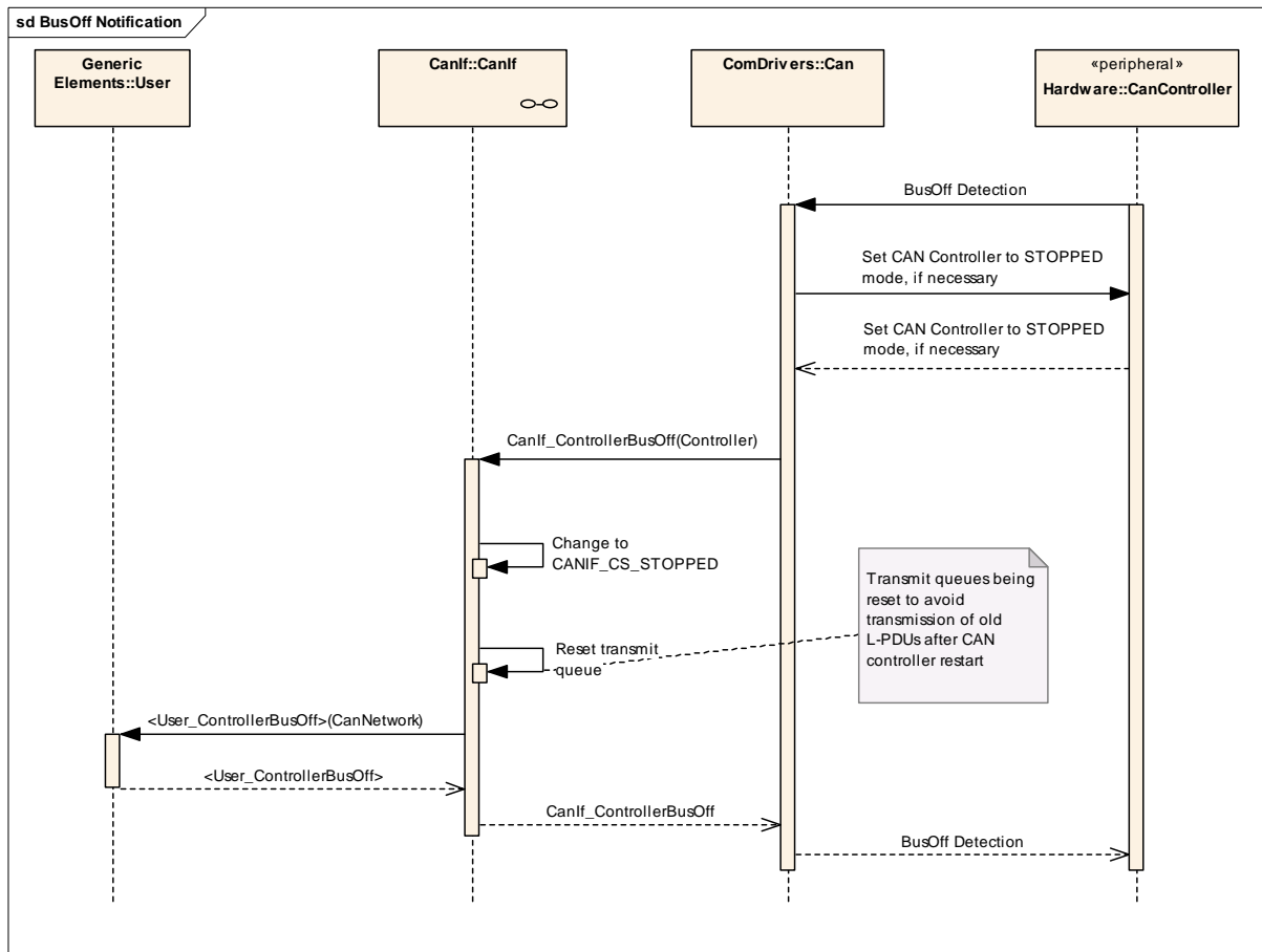
Figure 32 BusOff notification
