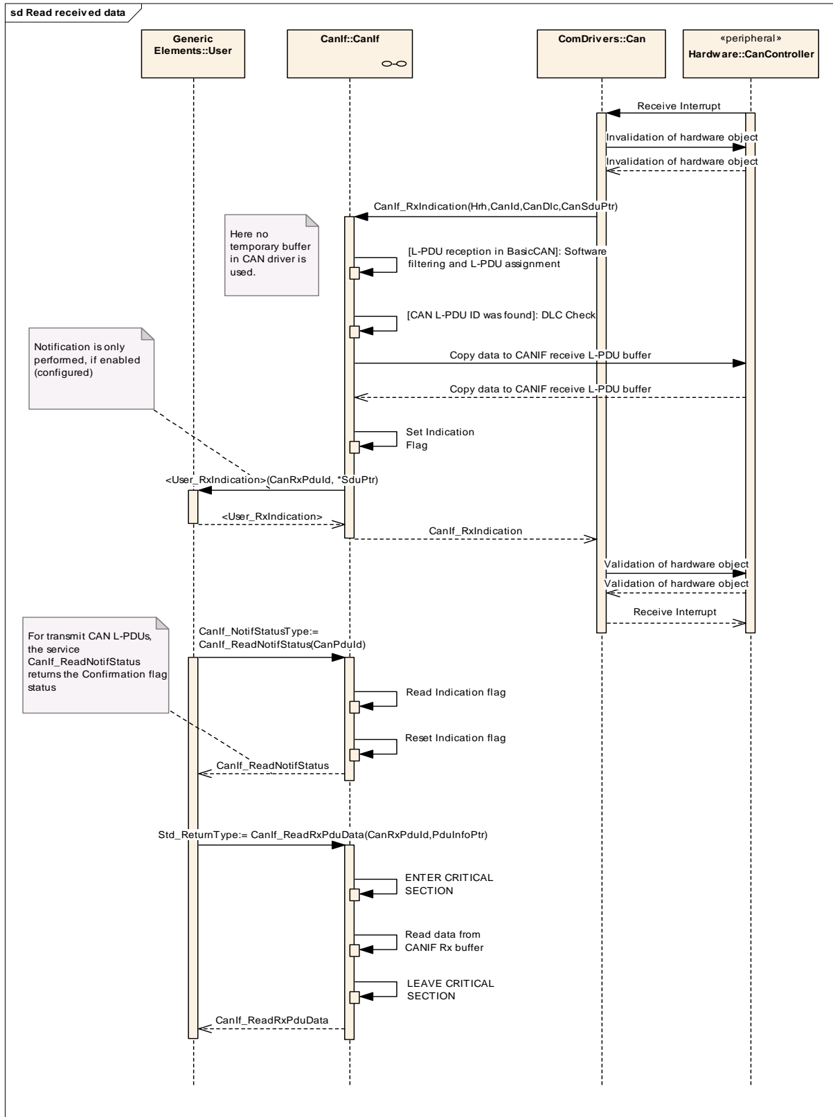
Figure 28 Read received data
