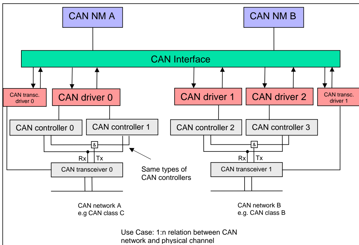
Figure 5: Network view definition example B
