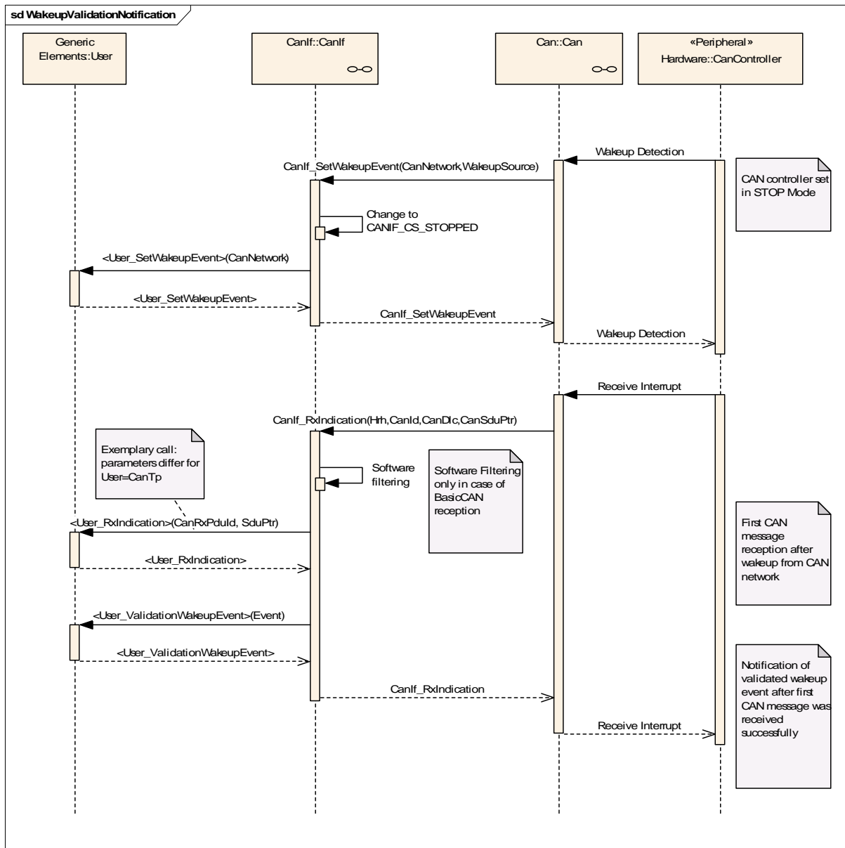
Figure 35 Wakeup notification with validation
