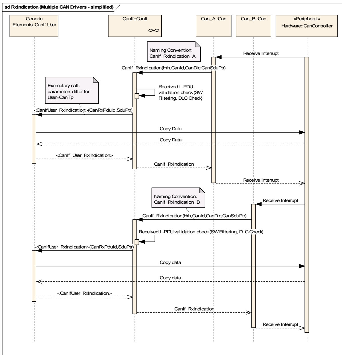
Figure 18 Receive interrupt with multiple CAN Drivers - simplified
