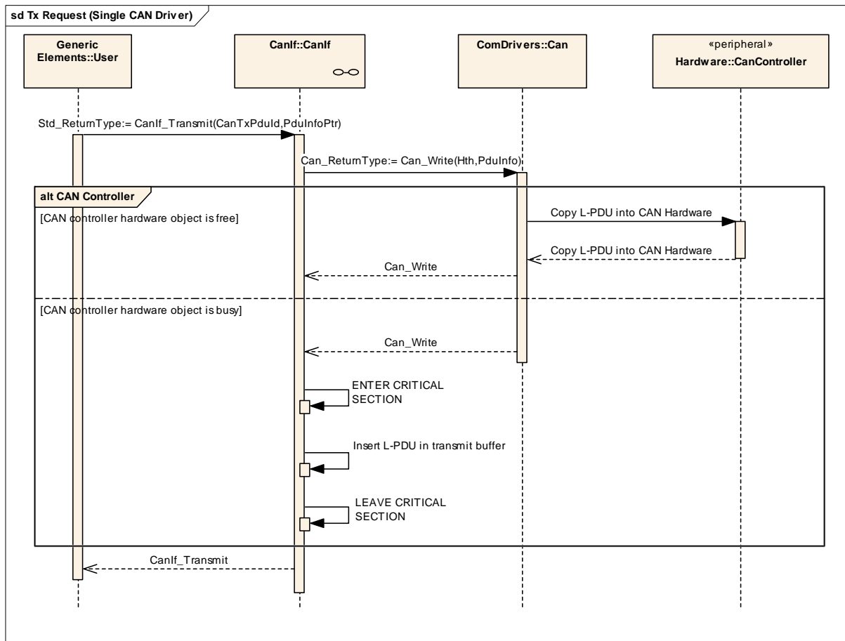
Figure 20 Transmission request with a single CAN Driver
