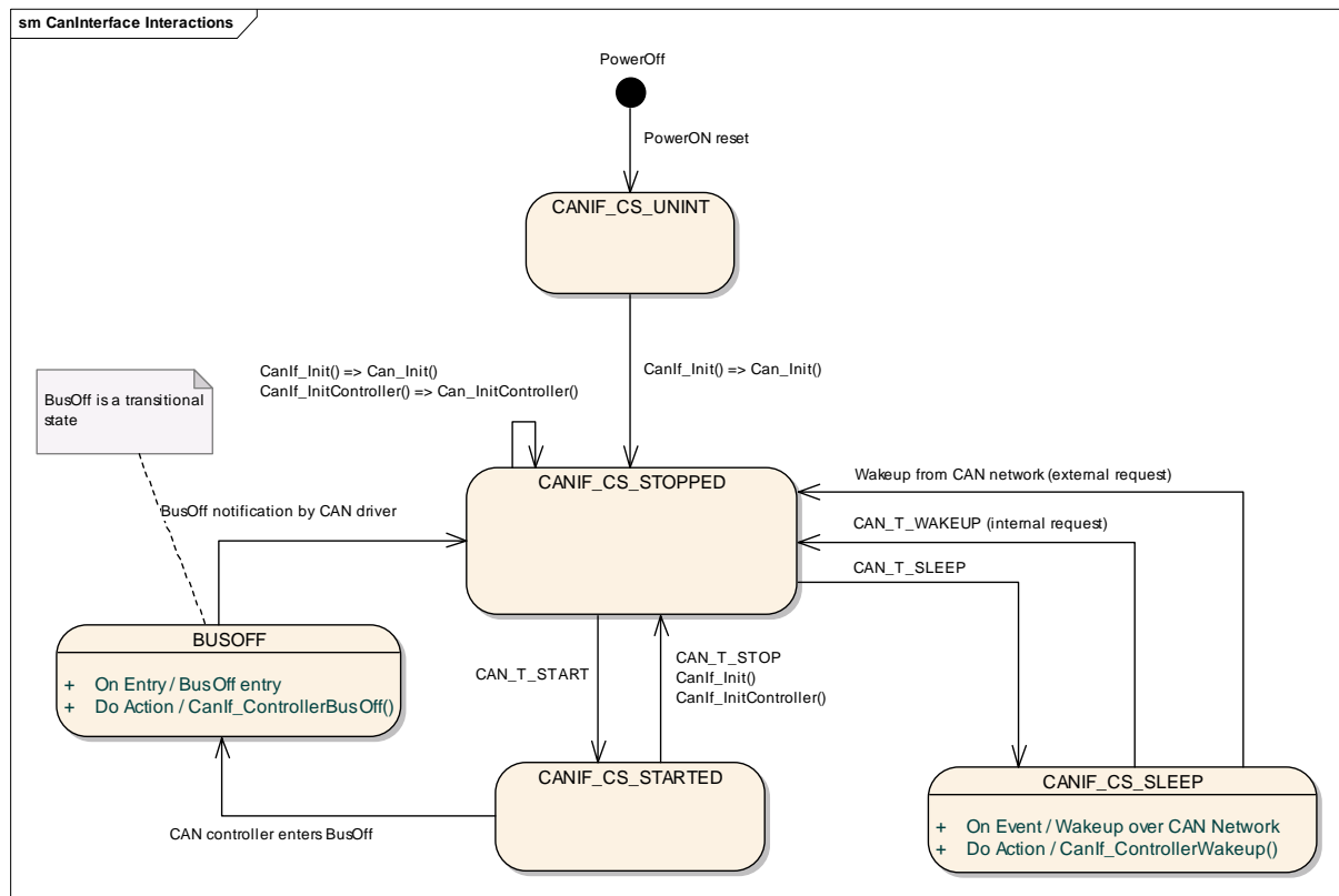
Figure 13 CAN Interface software states
