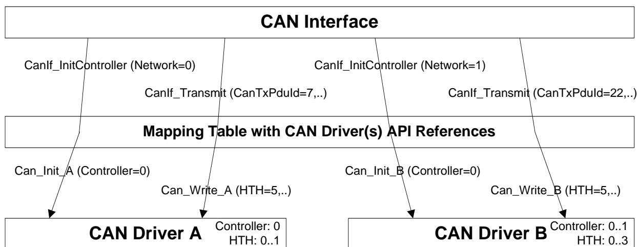
Figure 19 HTH Assignment with multiple CAN Drivers
