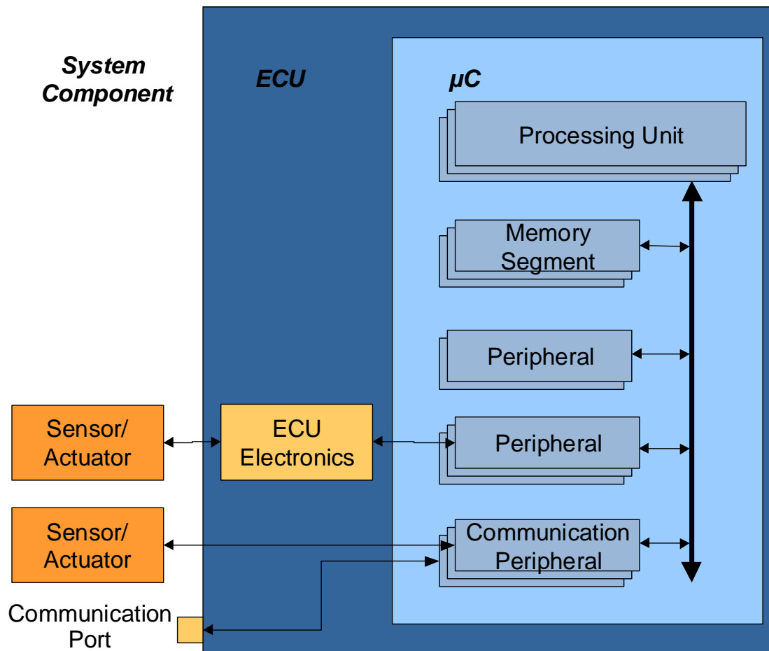
Figure 1-2: Overview ECU Template
