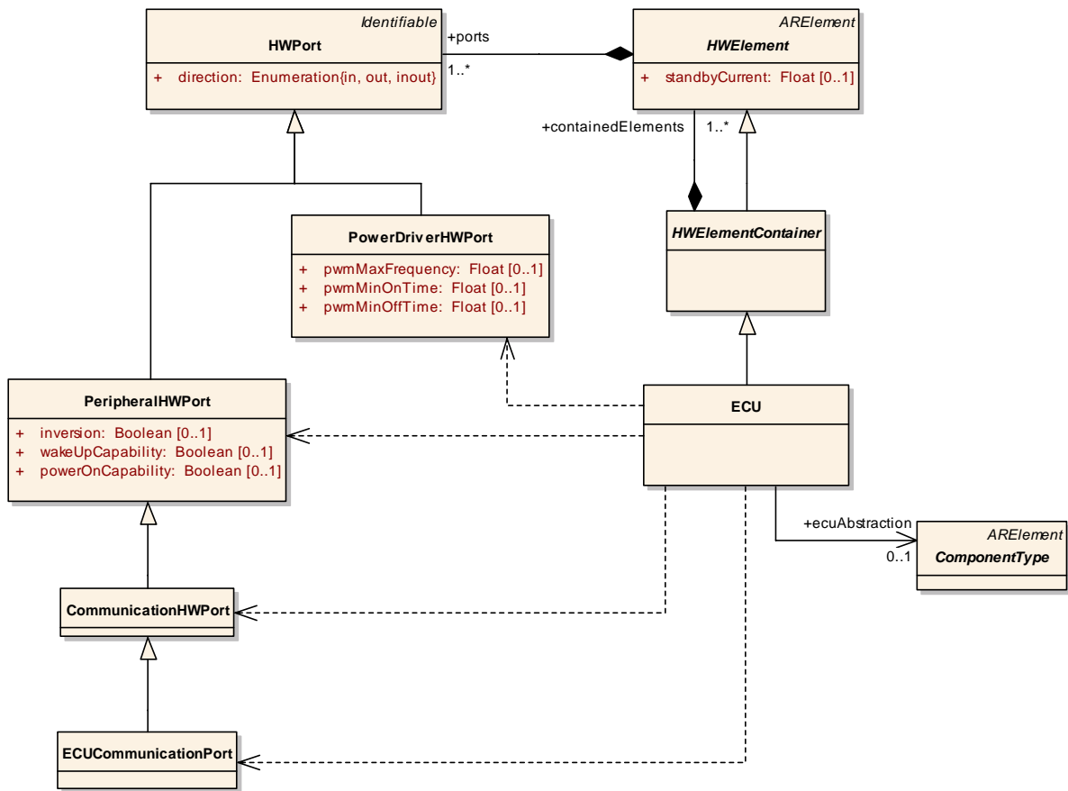
Figure 3-1: ECU Resource Overview
