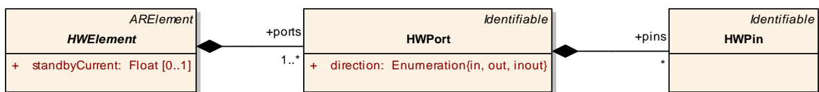
Figure 2-4: Definition of HW Port in the Meta-Model
