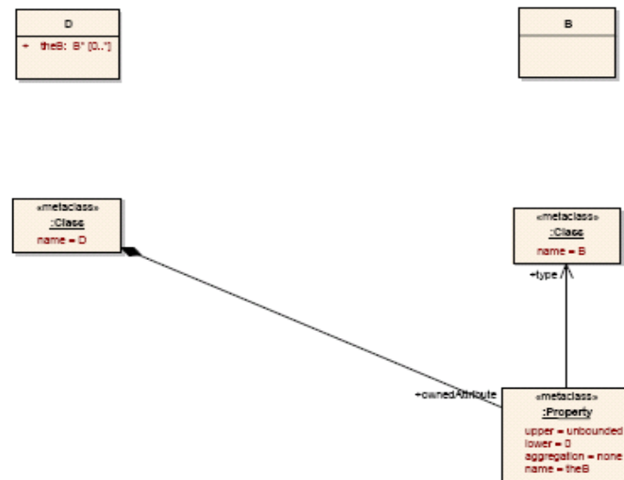
Figure 3-4: Representation of attribute (aggregation = none)
