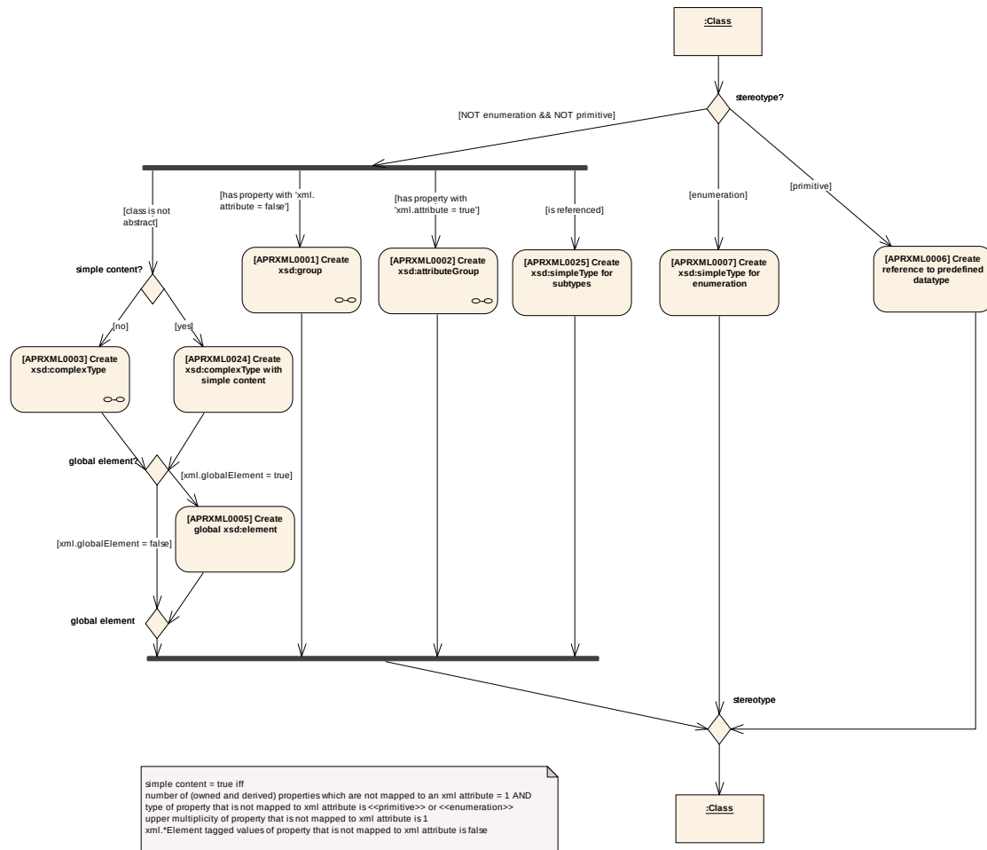
Figure 5-2: Class representation
