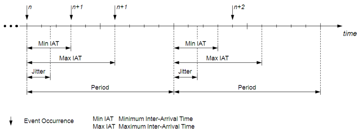
Figure 7.10: Parameters characterizing the Sporadic Event Triggering
