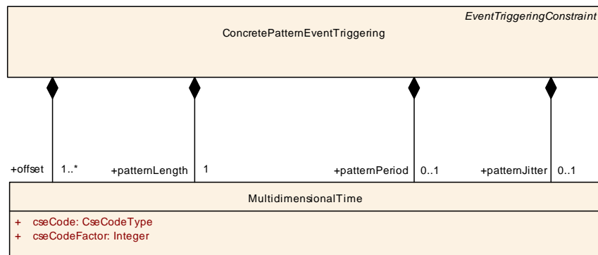
Figure 7.11: ConcretePatternEventTriggering
