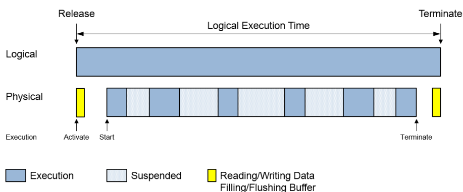
Figure 4.10: LET Approach
