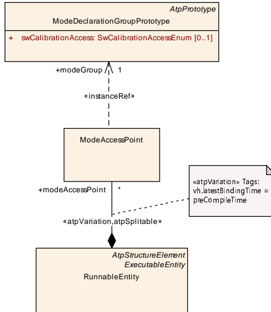
Figure 9.6: ModeAccessPoint
