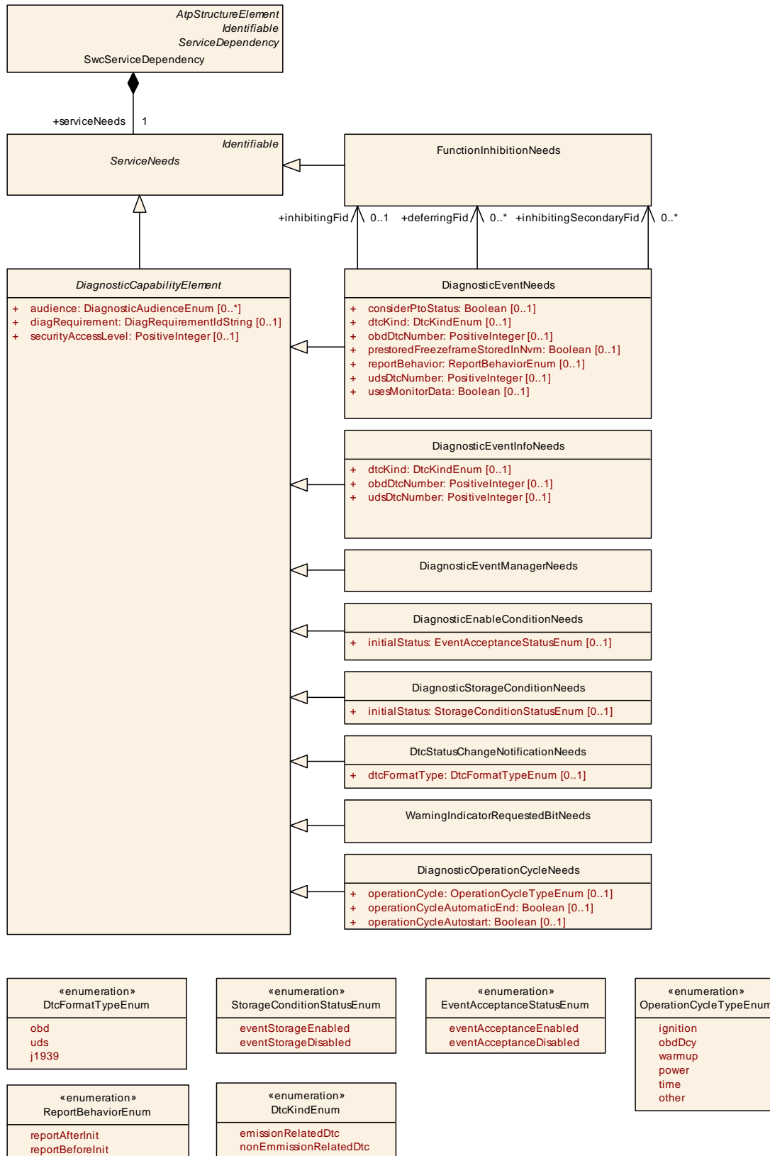
Figure 7.39: General diagnostic event-handling related ServiceNeeds
