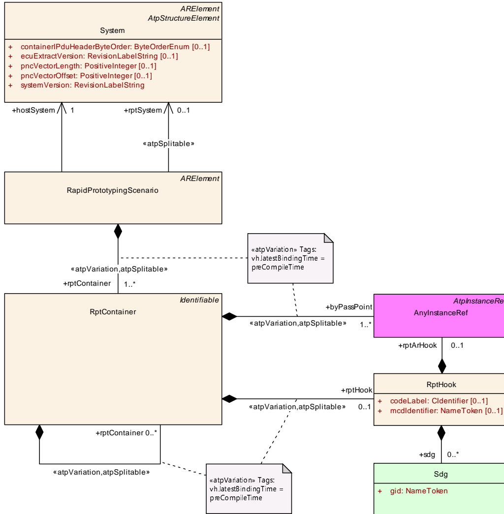
Figure 14.2: Rapid Prototyping Hooks
