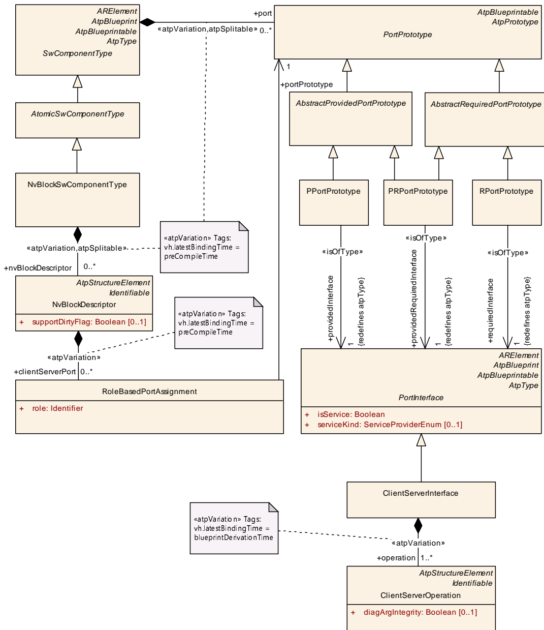
Figure 11.22: NvBlockNotification
