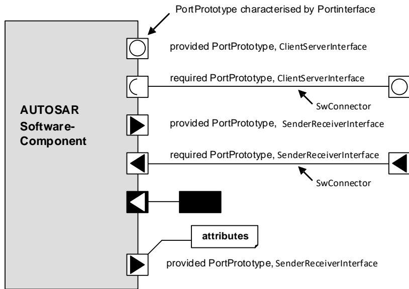
Figure 3.1: Graphical representation of software-components in AUTOSAR
