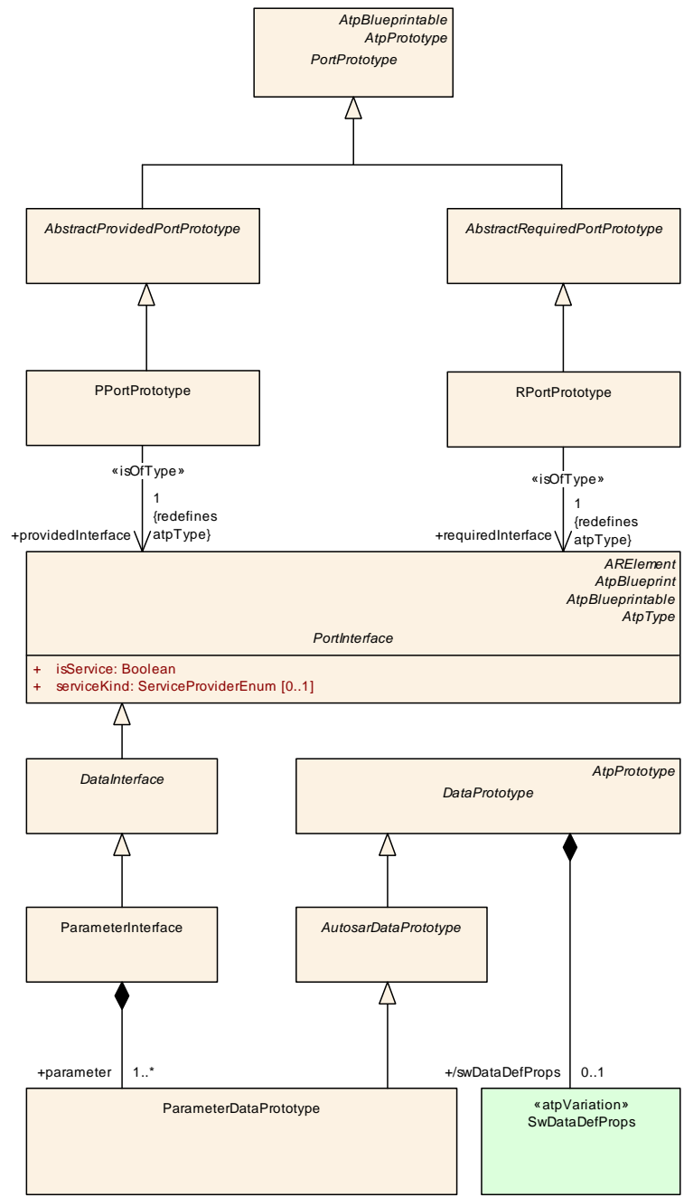
Figure 2.2: ParameterInterface
