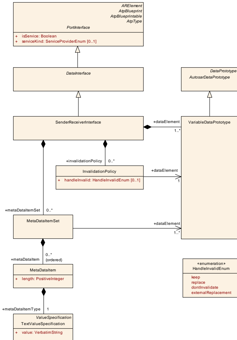
Figure 4.1: dataElements of a SenderReceiverInterface
