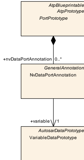
Figure 4.28: NvDataPortAnnotation
