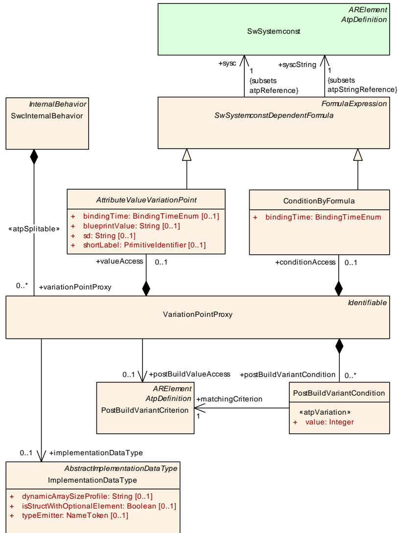
Figure 7.48: VariationPointProxy
