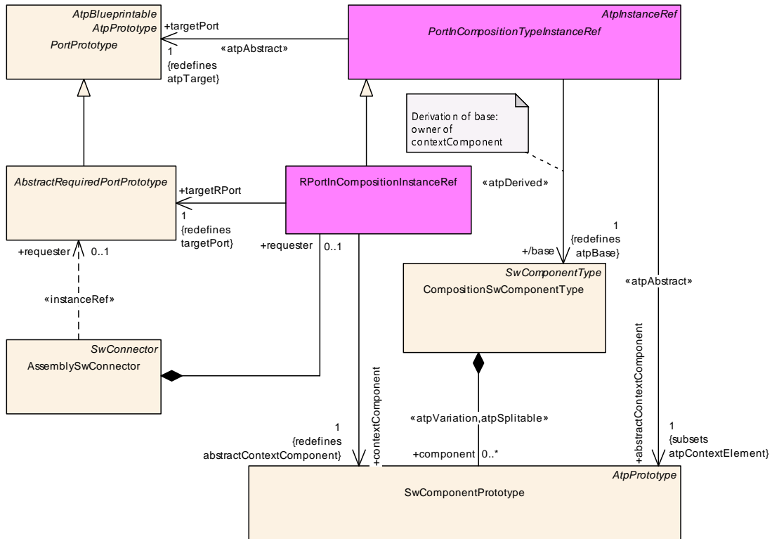
Figure D.16: Concrete modeling of references to RPortPrototype in the context of a CompositionSwComponentType
