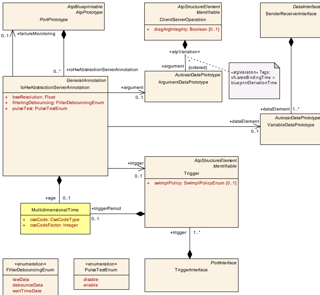
Figure 4.24: IoHwAbstractionServerAnnotation
