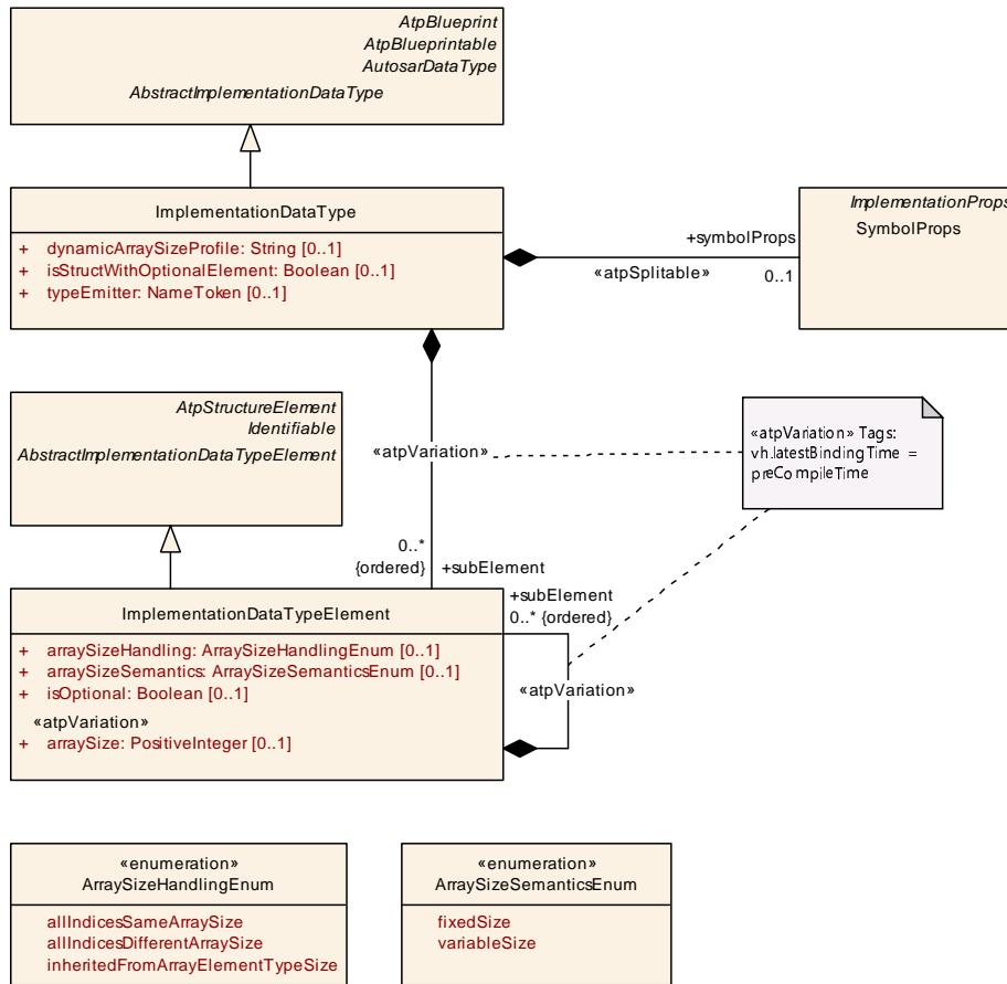
Figure 5.14: ImplementationDataType overview
