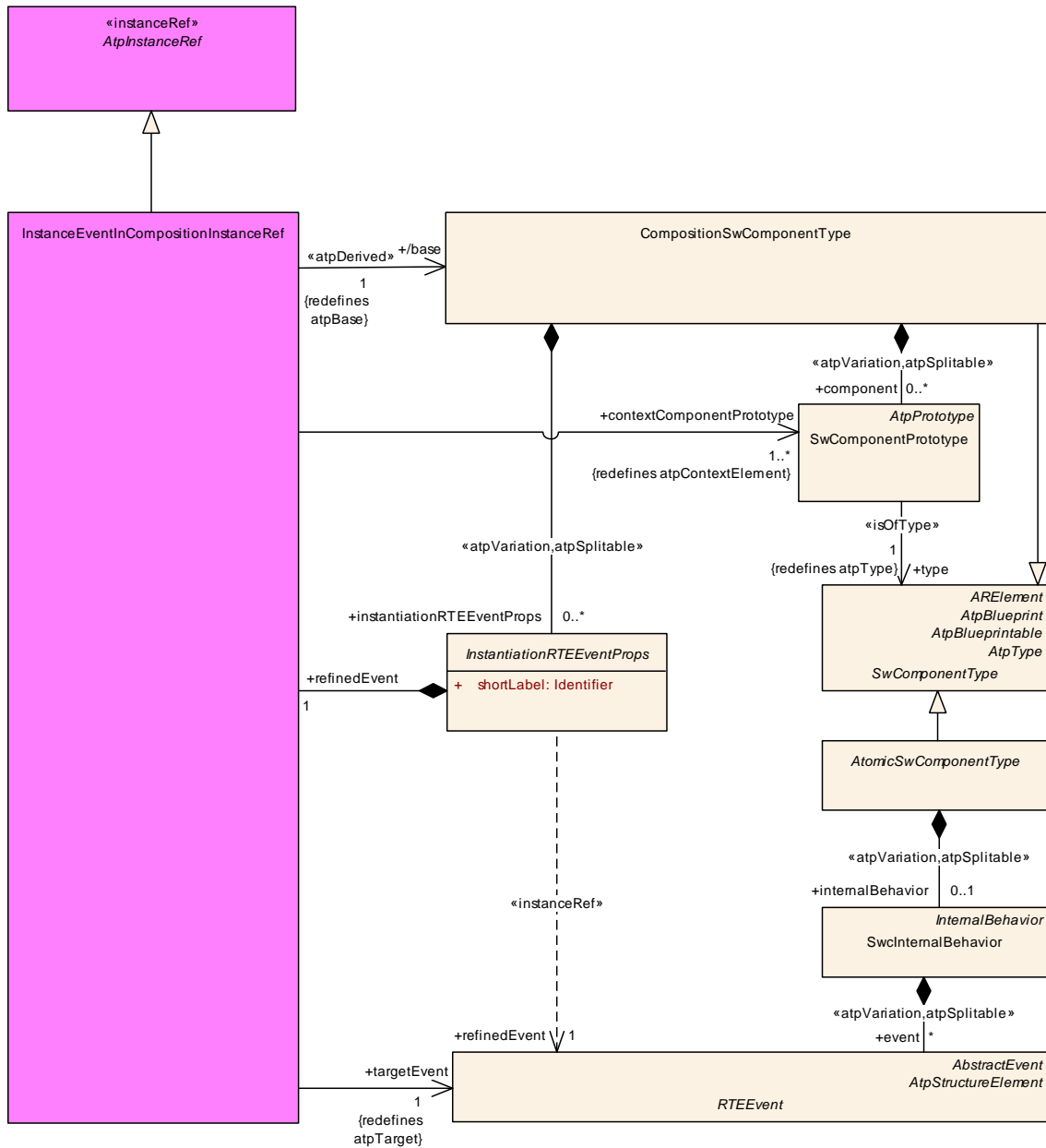
Figure D.22: Modeling of references to RTEEvent in the context of an InstantiationRTEEventProps from the point of view of a CompositionSwComponentType
