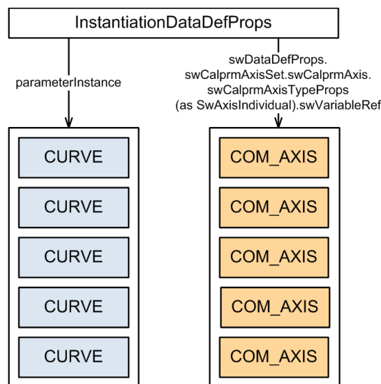
Figure 5.45: The n th CURVE in the array of CURVES relates to the n th COM_AXIS in the array of COM_AXIS s
