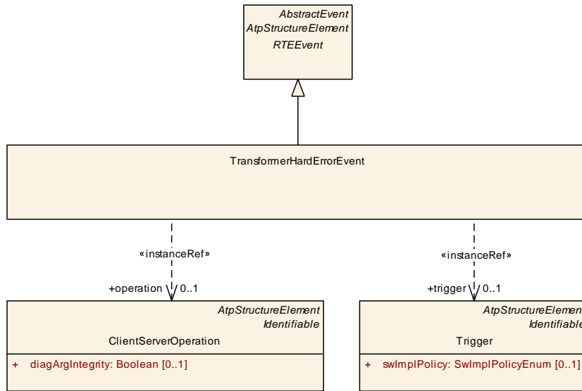
Figure 7.11: RTEEvent used in the context of data transformation
