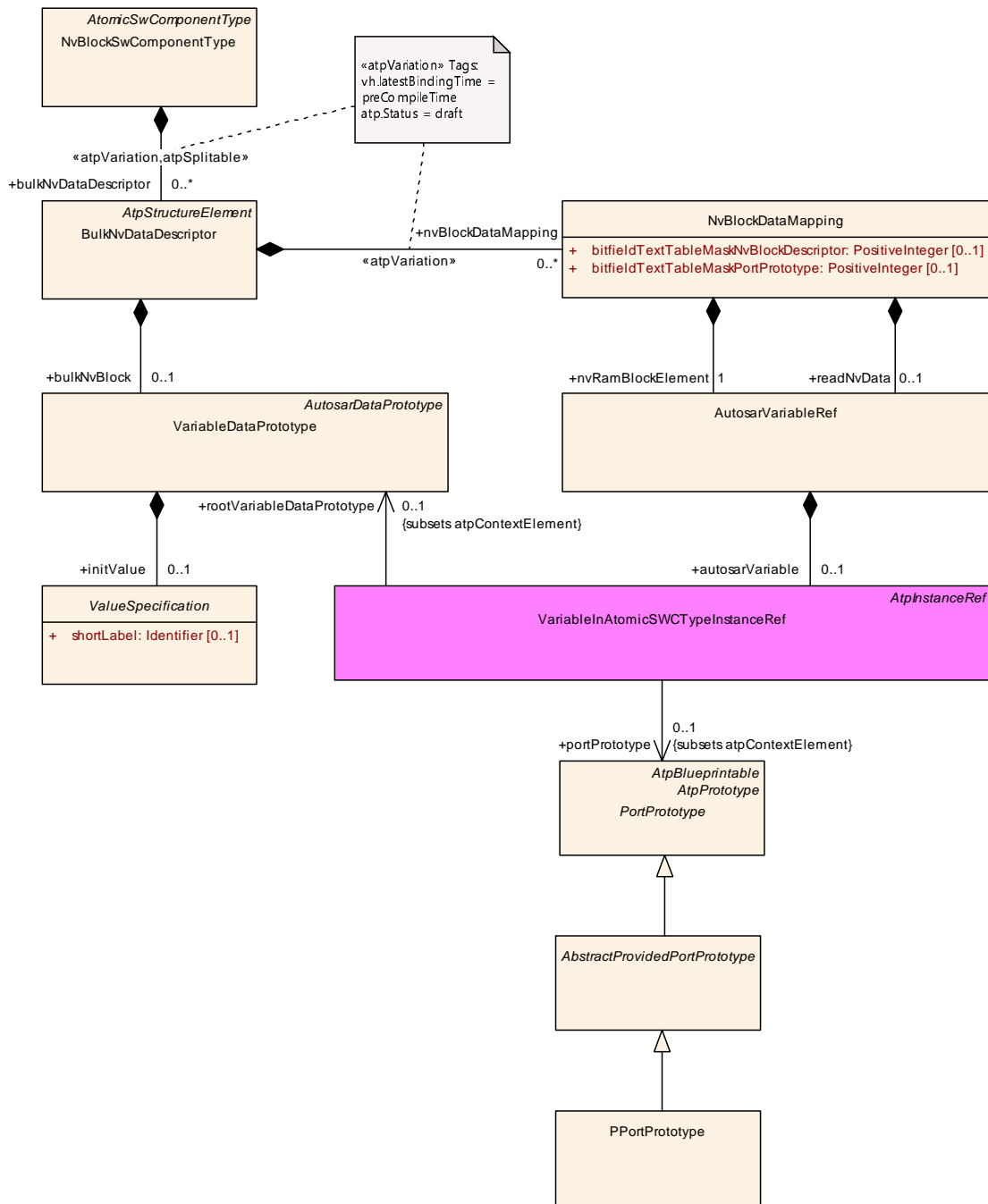
Figure 11.23: NvBlockSwComponentType and BulkNvDataDescriptor
