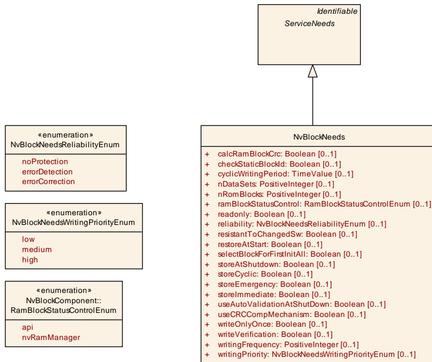
Figure 11.16: NvBlockNeeds
