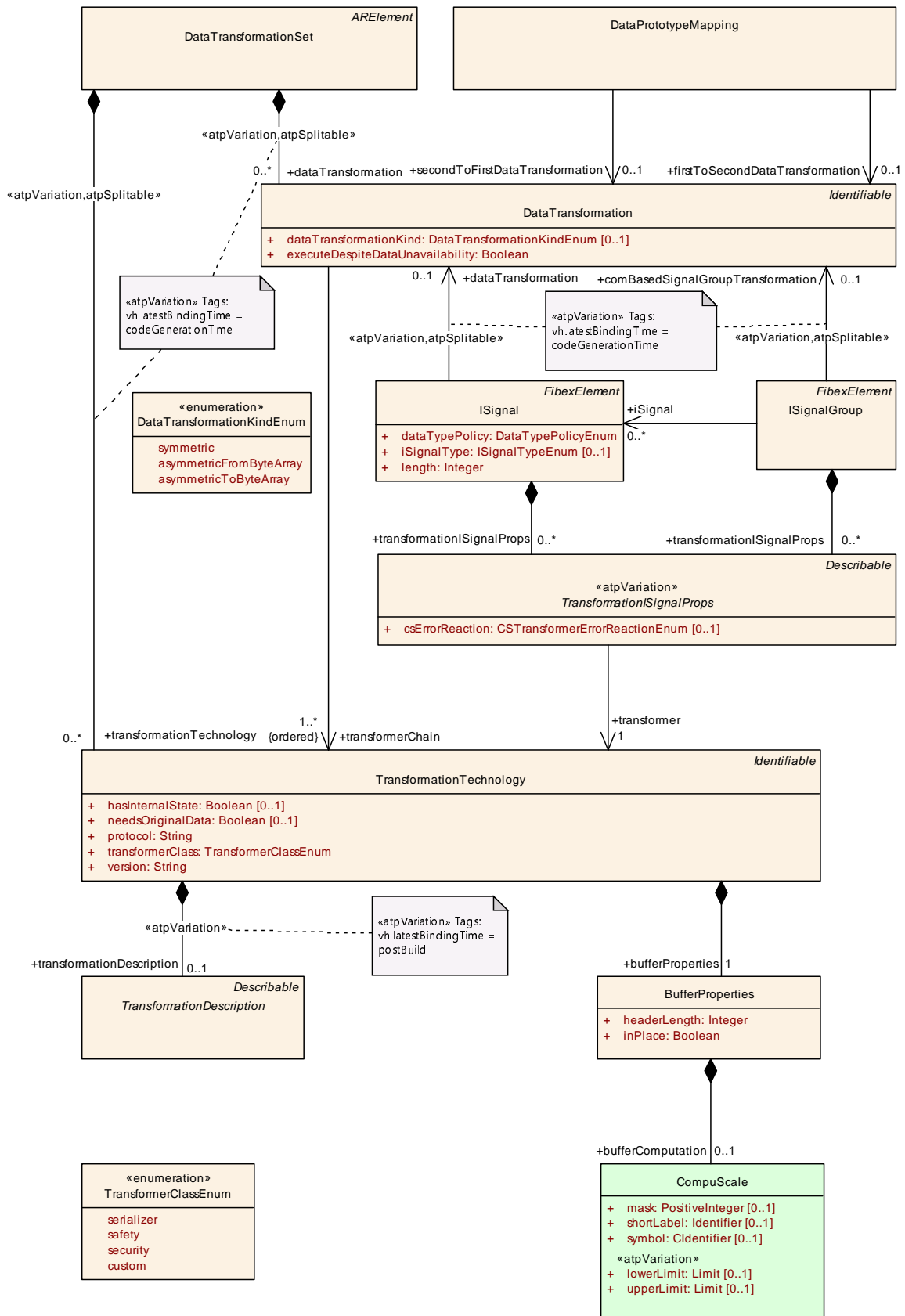
Figure 4.44: Big picture of data transformation in the AUTOSAR meta-model
