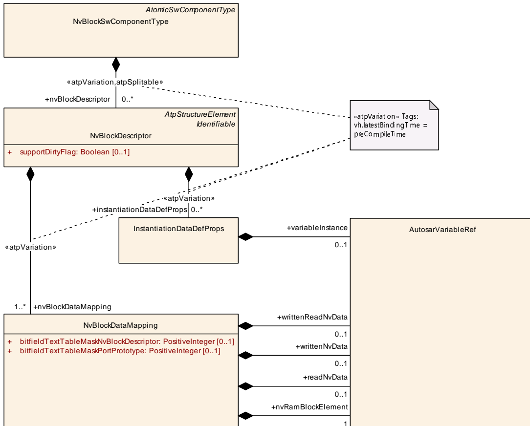
Figure 11.20: Attributes of NvBlockDataMapping
