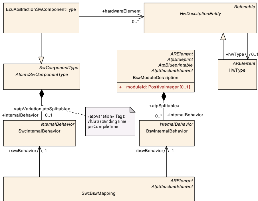
Figure 10.7: EcuAbstractionSwComponentType
