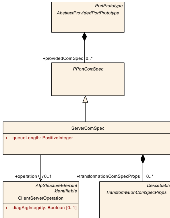
Figure 4.36: Communication attributes of PPortPrototype with respect to client-server communication.
