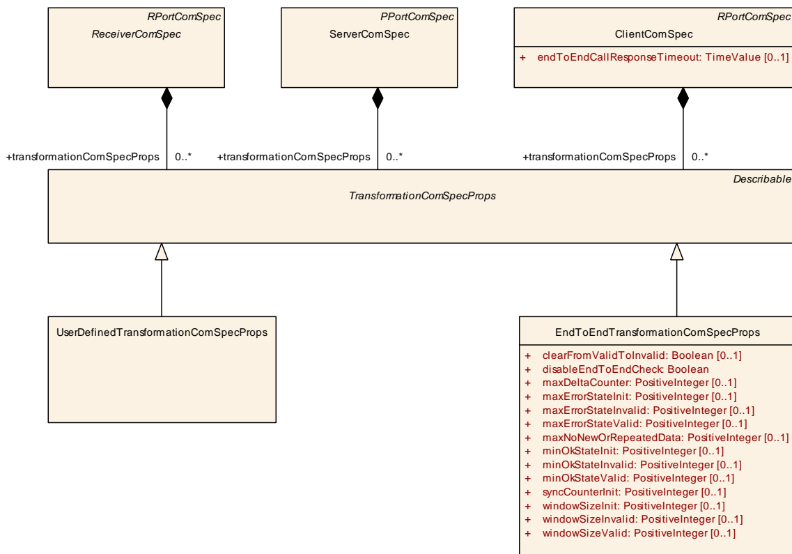
Figure 4.43: Specification of data transformation properties within ReceiverComSpec, ServerComSpec, and ClientComSpec
