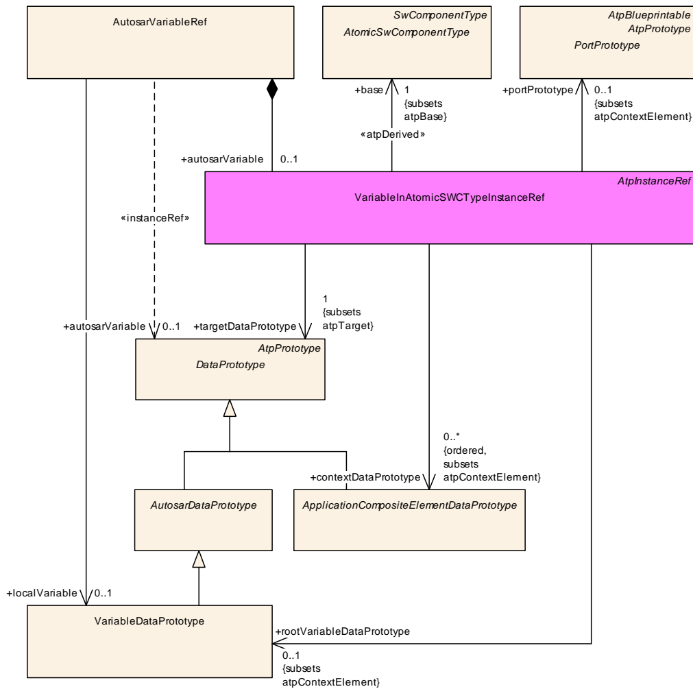
Figure 5.25: Implementation of the InstanceRef for AutosarVariableRef
