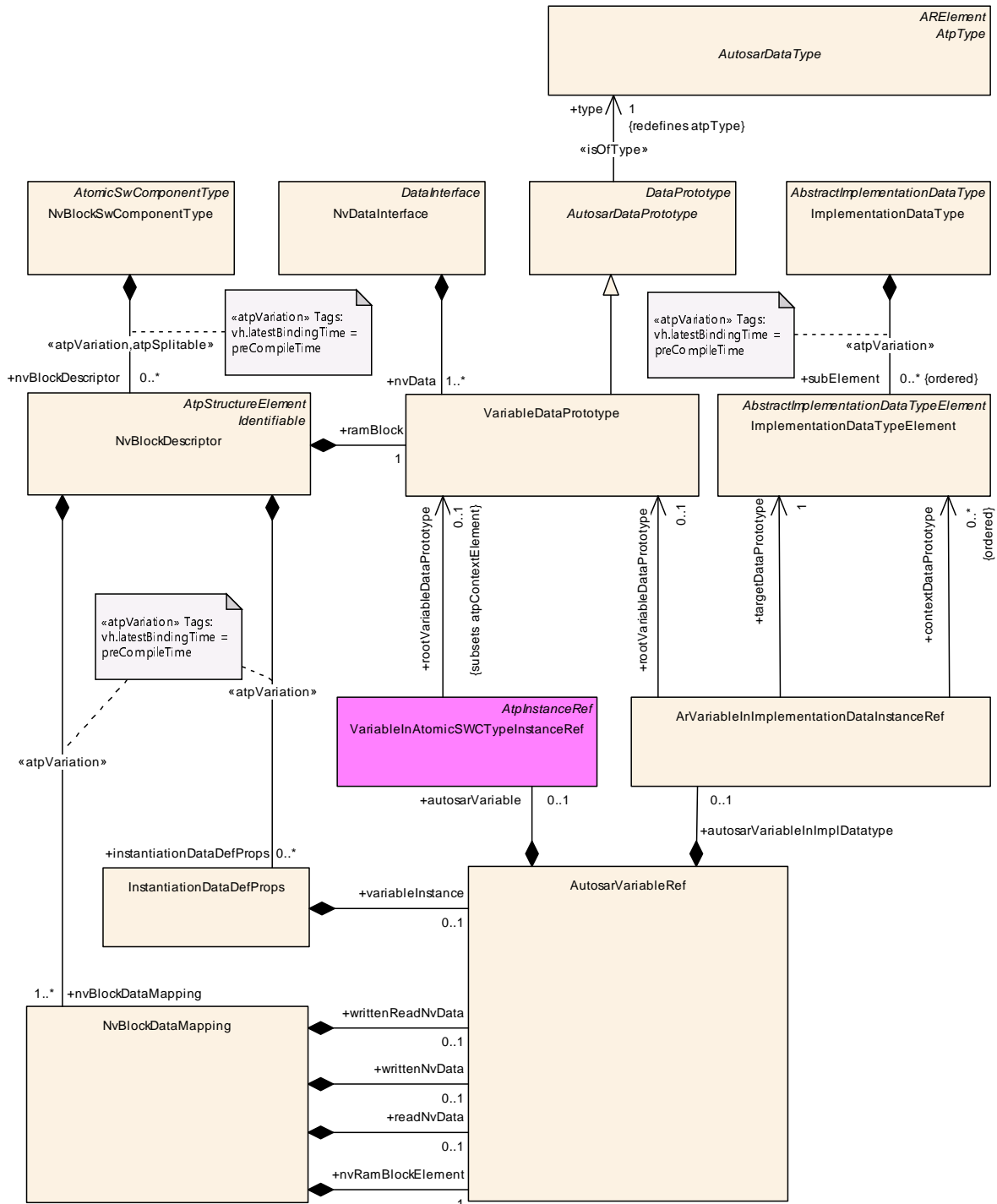
Figure 11.19: NvBlockDataMapping and InstantiationDataDefProps
