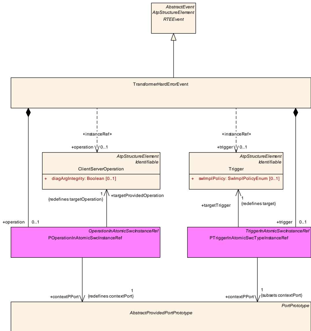
Figure D.31: Modeling of transformer error response
