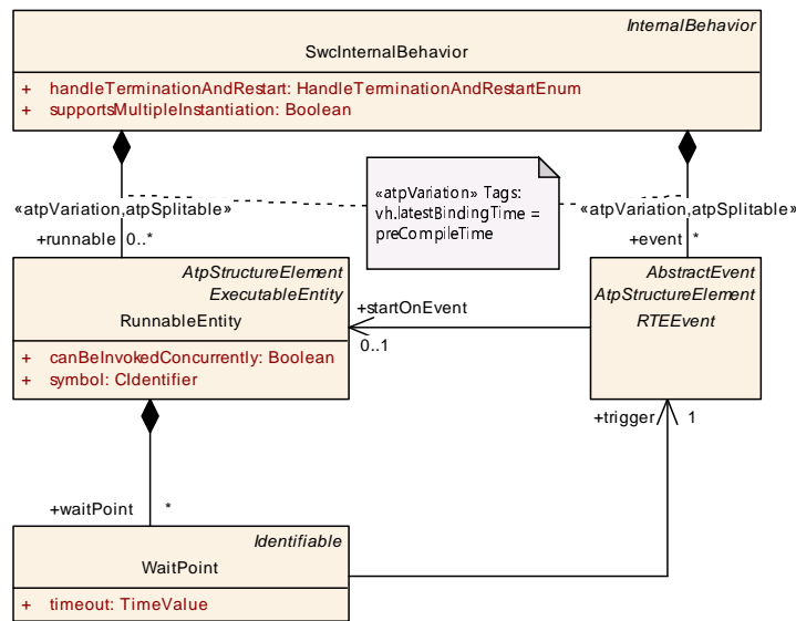
Figure 7.13: Description of the interaction between an RTEEvent and RunnableEntities
