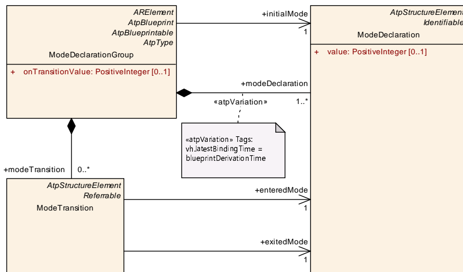
Figure 9.2: ModeTransition
