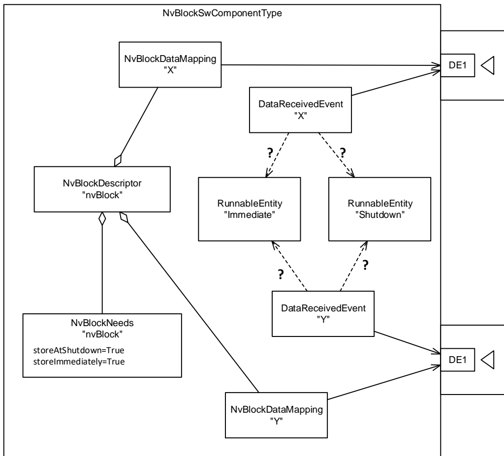
Figure 11.13: Existence of several event-based writing strategies for the same NvBlockDescriptor
