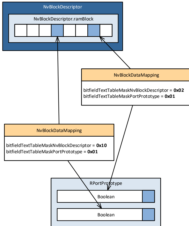
Figure 11.21: Visualization of the approach to map bitfields inside an NvBlockSwComponentType
