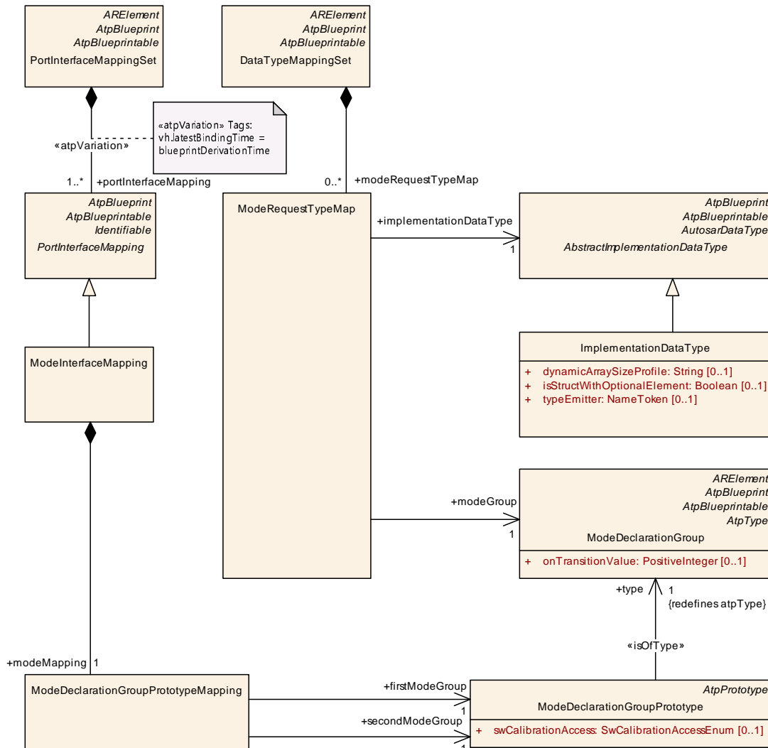
Figure 4.6: Mapping of modes to data types
