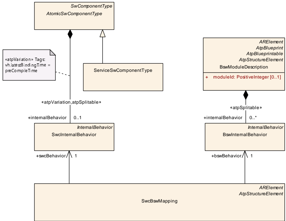
Figure 11.2: ServiceSwComponentType
