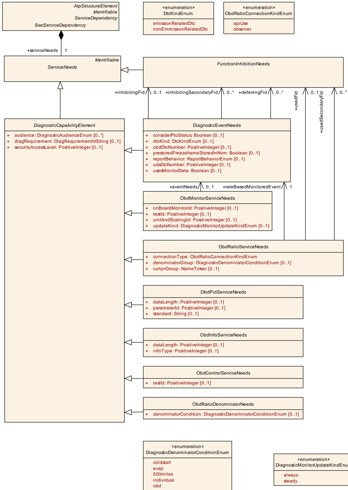
Figure 7.40: ServiceNeeds: Diagnostic-related ServiceNeeds with emphasis on OBD
