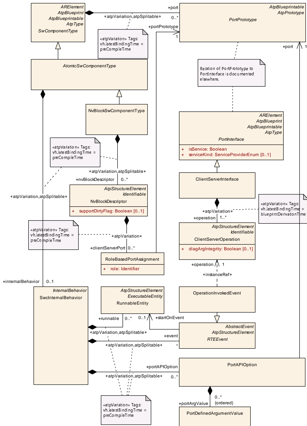
Figure 11.24: NvBlockSwComponentType and SwcInternalBehavior
