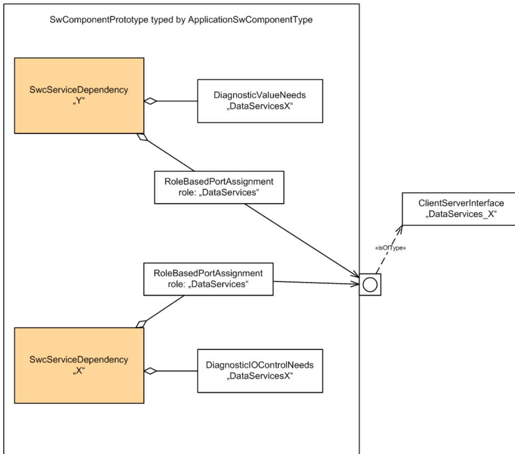
Figure 7.47: Two SwcServiceDependencies referencing one PortPrototype
