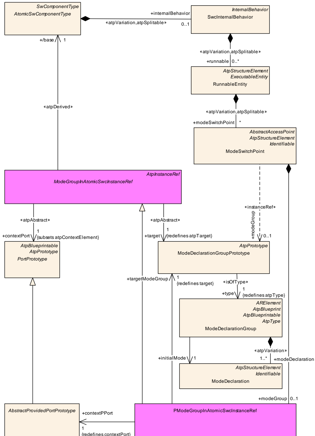
Figure D.23: Modeling of references to provided ModeDeclarationGroupPrototype in the context of an AtomicSwComponentType
