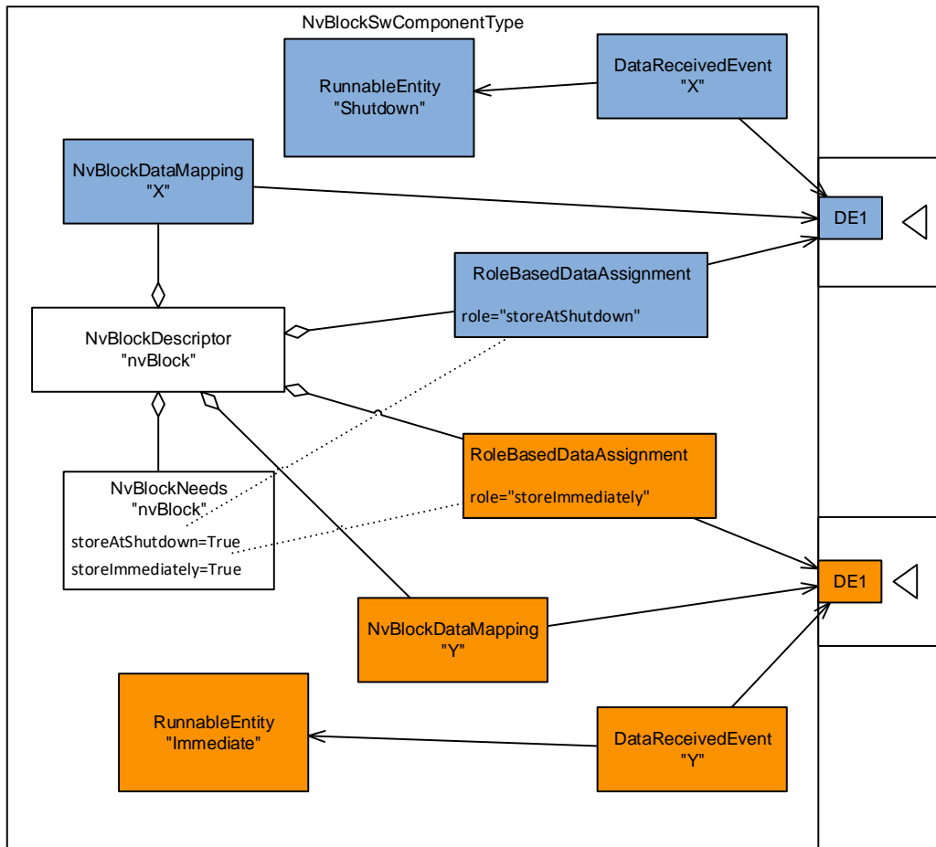
Figure 11.15: Solution for the existence of several event-based writing strategies for the same NvBlockDescriptor
