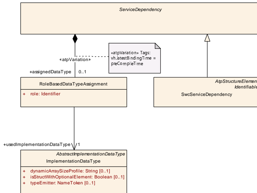
Figure 7.46: Details of RoleBasedDataTypeAssignment for local data
