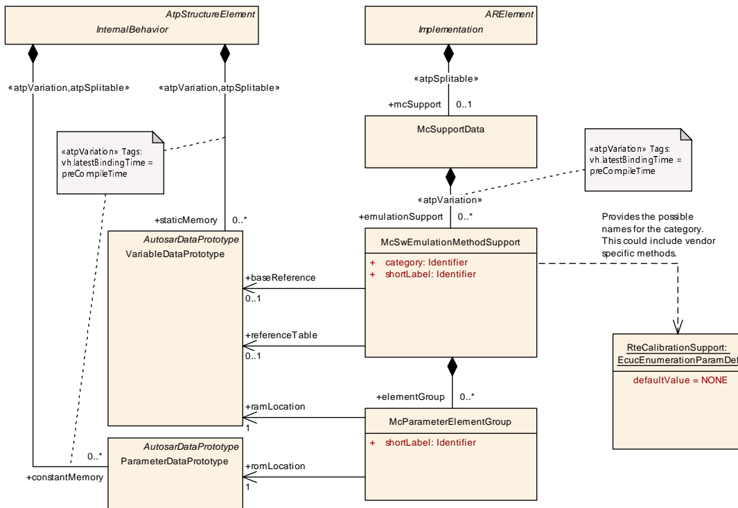
Figure 10.3: Describing the Software Emulation Method for Calibration Data
