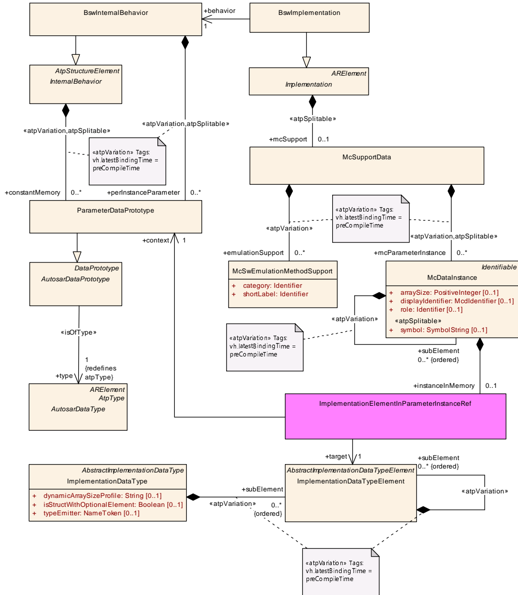
Figure 10.4: Reference to the Implemented Data needed for Emulation
