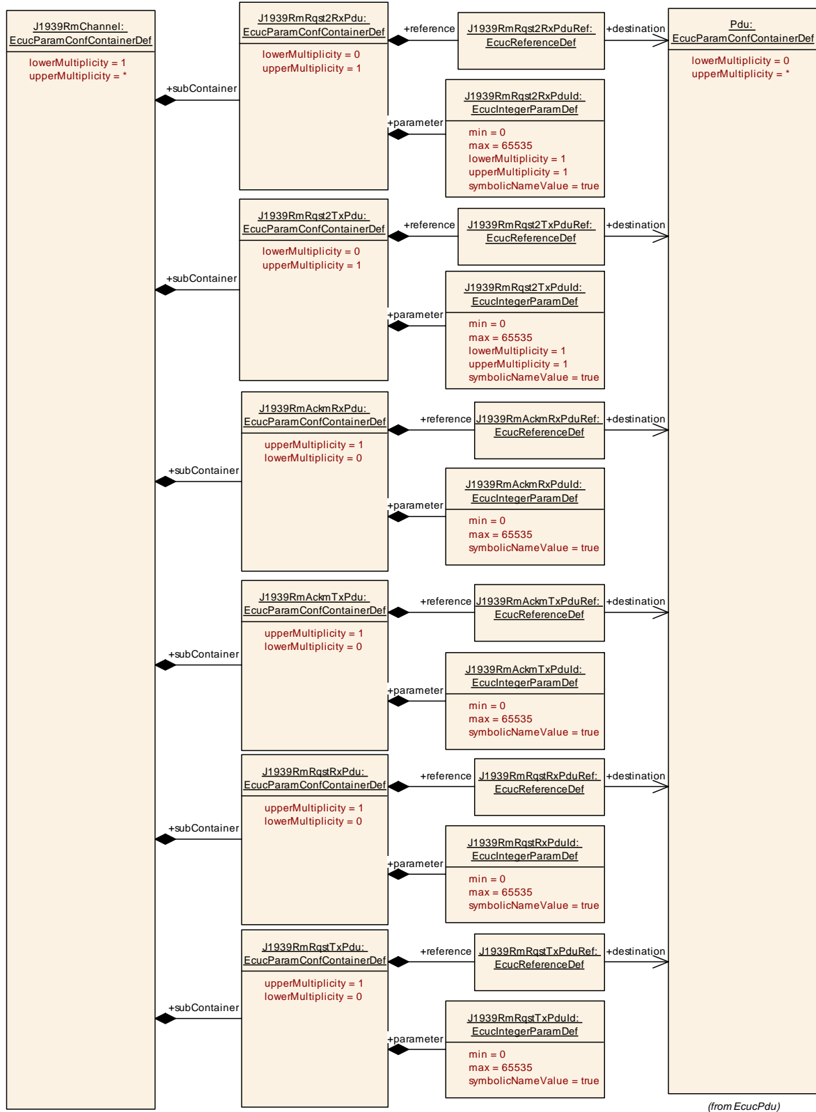
Figure 11: Configuration container J1939RmChannel with PDUs
