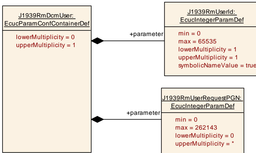
Figure 15: Configuration container J1939RmDcmUser
