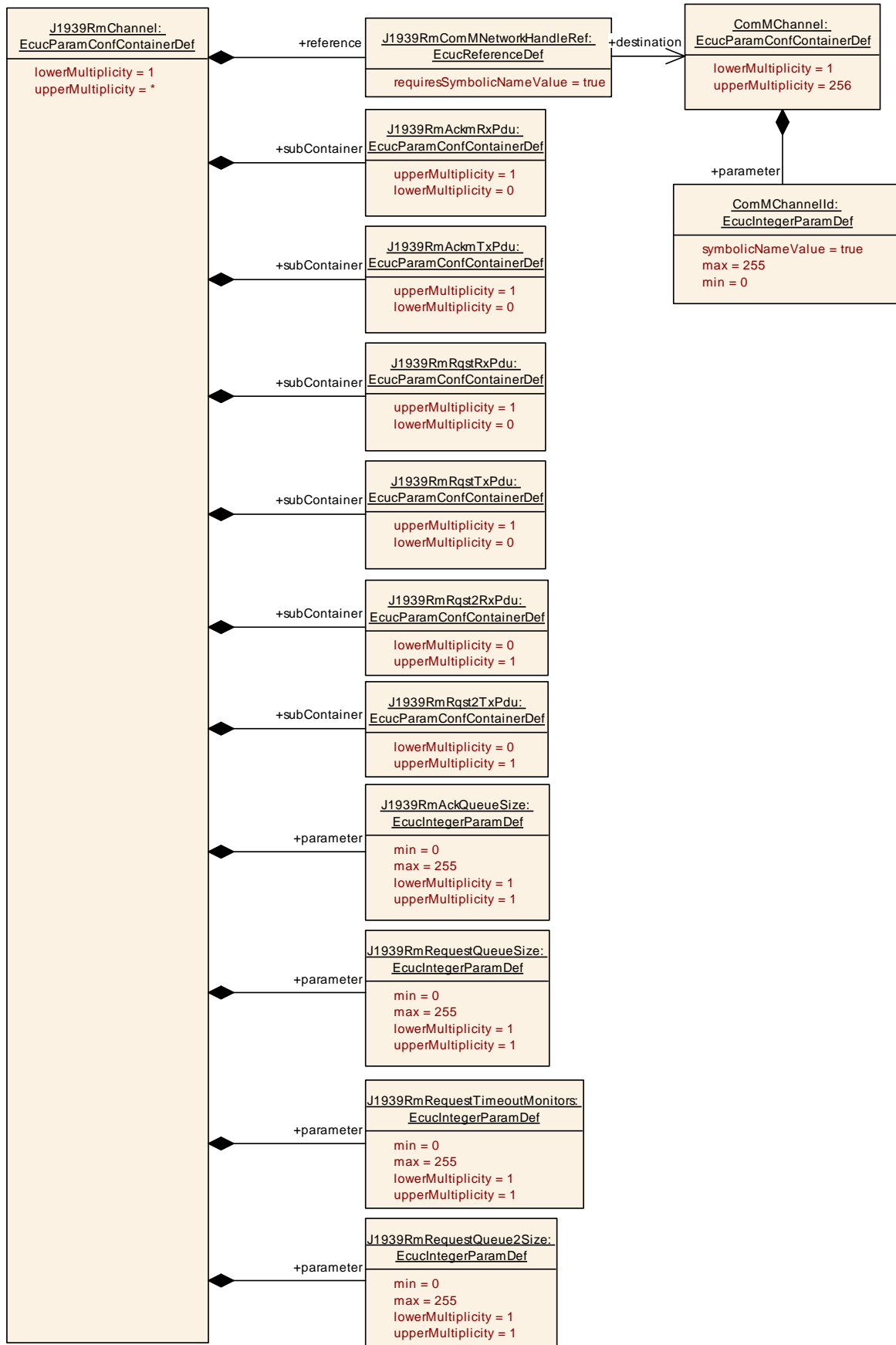
Figure 10: Configuration container J1939RmChannel
