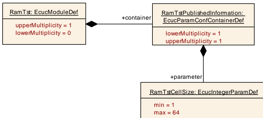
Figure 20: RamTstPublishedInformation
