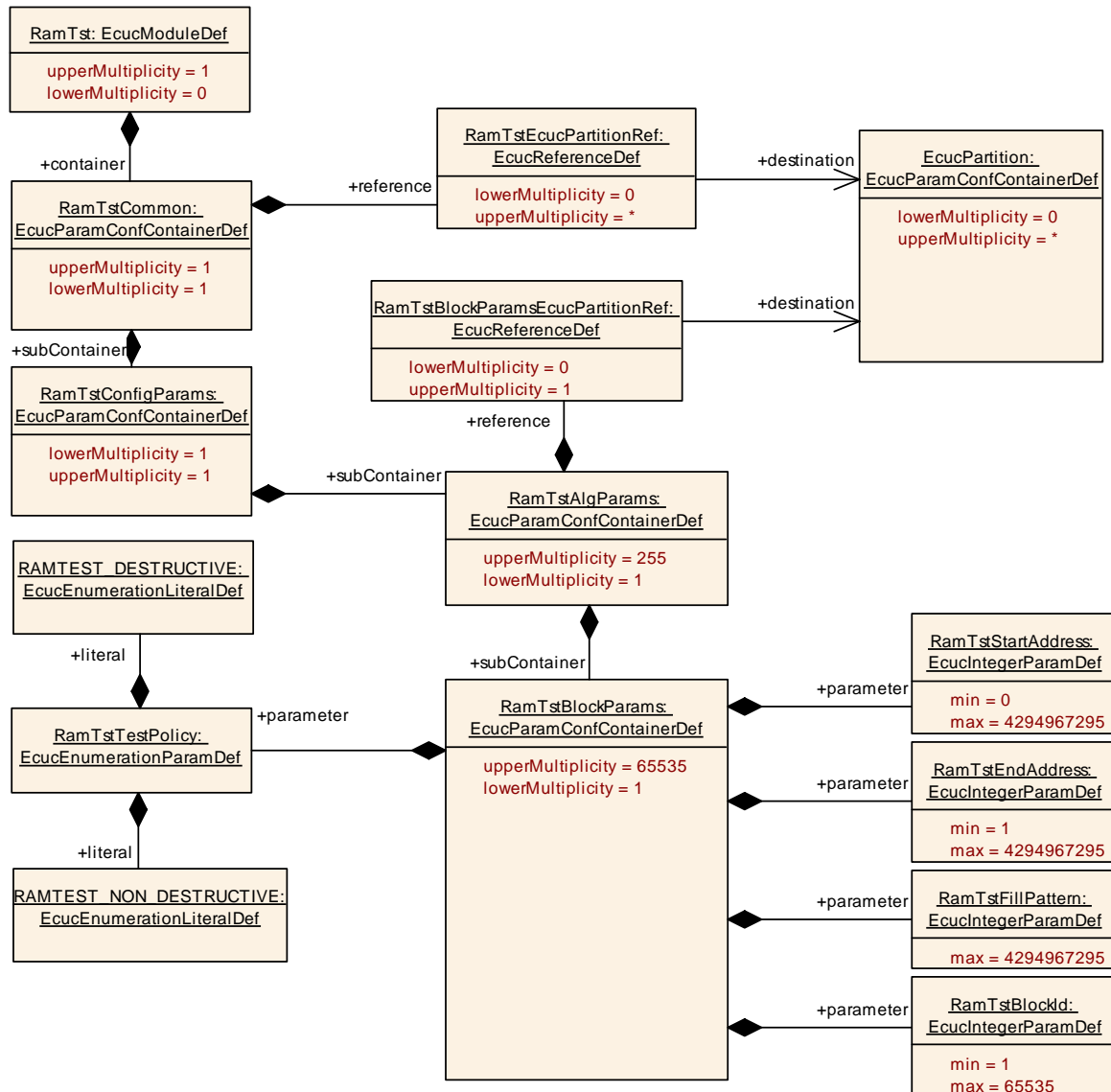
Figure 19: RamTstBlockParams
