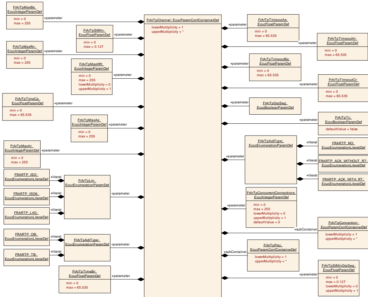
Figure 23: FrArTpChannel configuration
