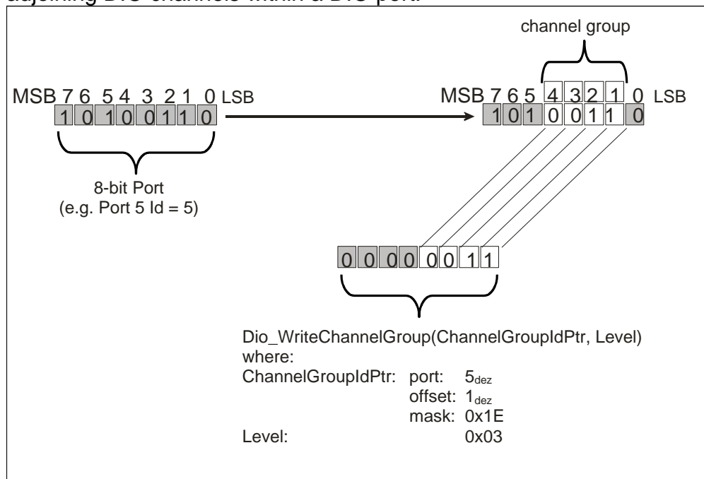
Figure 2: Schematic description of a ChannelGroup
