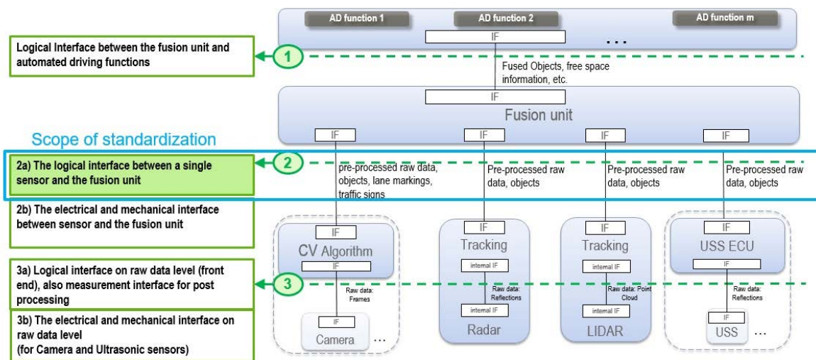
Figure 4.1: Scope of Sensor Interface Standardization
