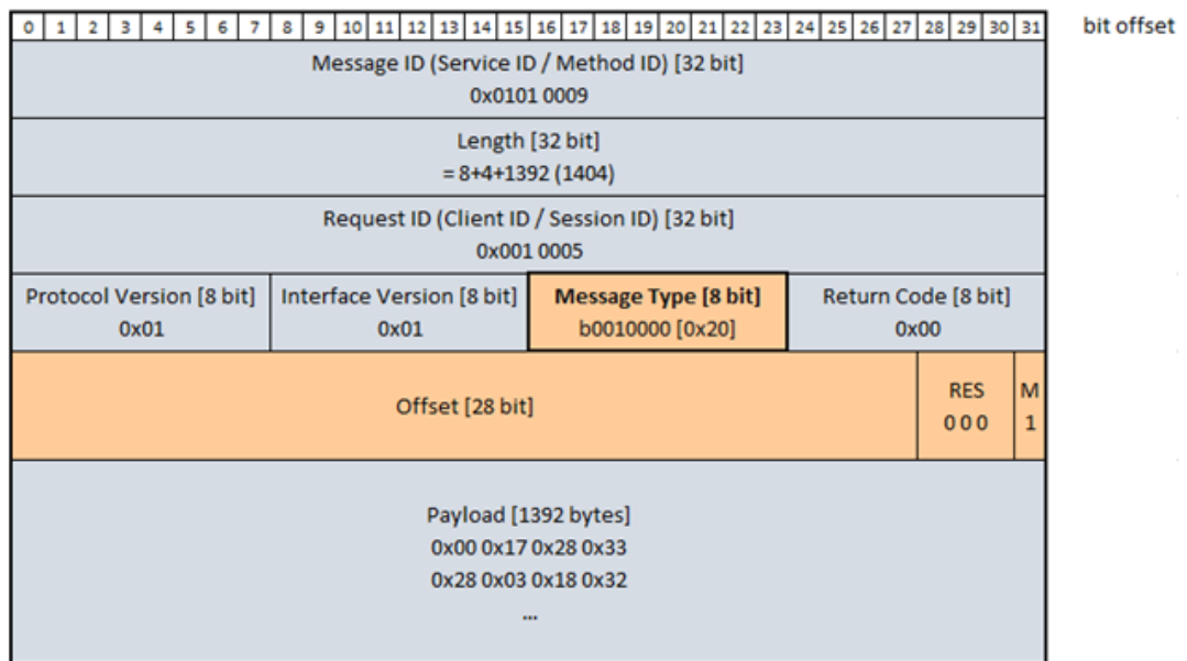
Figure 4.19: Example: Header of the SOME/IP segments
