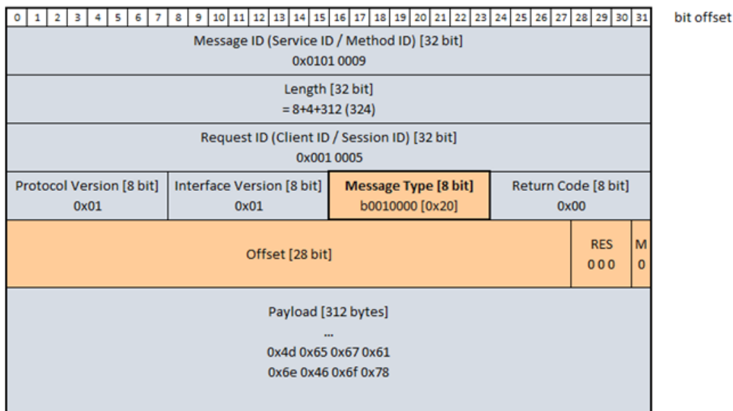
Figure 4.20: Example: Header of the last SOME/IP segment
