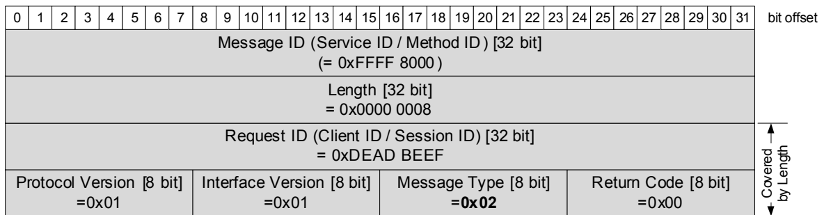
Figure 4.15: SOME/IP Magic Cookie Message for SOME/IP
