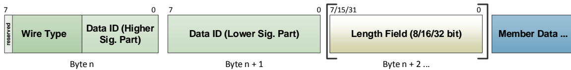
Figure 4.6: Tag Layout
