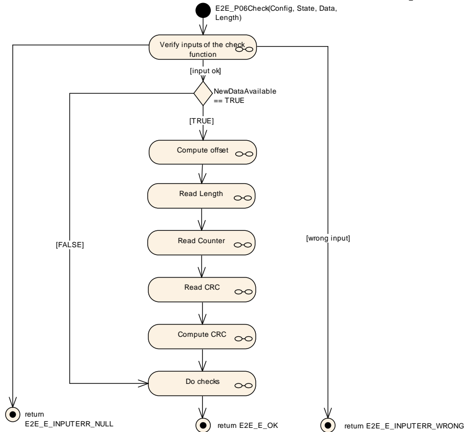
Figure 6.53: E2E Profile 6 Check
