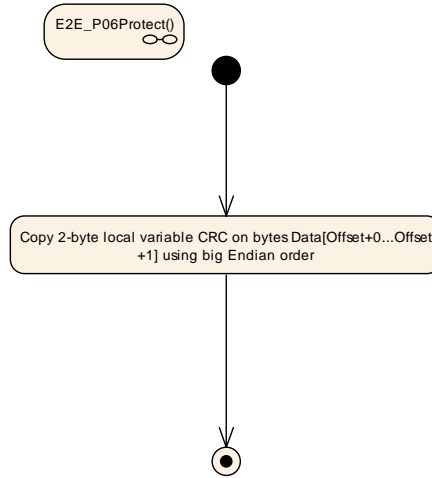
Figure 6.51: E2E Profile 6 Protect step "Write CRC"
