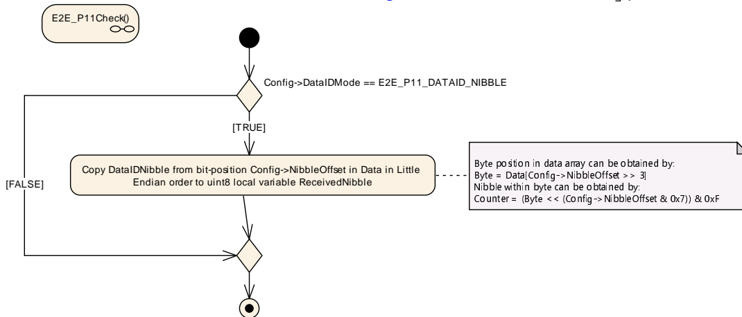
Figure 6.87: E2E Profile 11 Check step "Read DataIDNibble"
