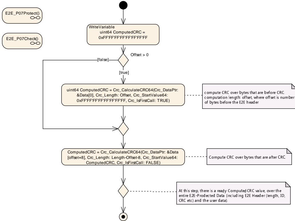
Figure 6.66: E2E Profile 7 Protect and Check step "ComputeCRC"
