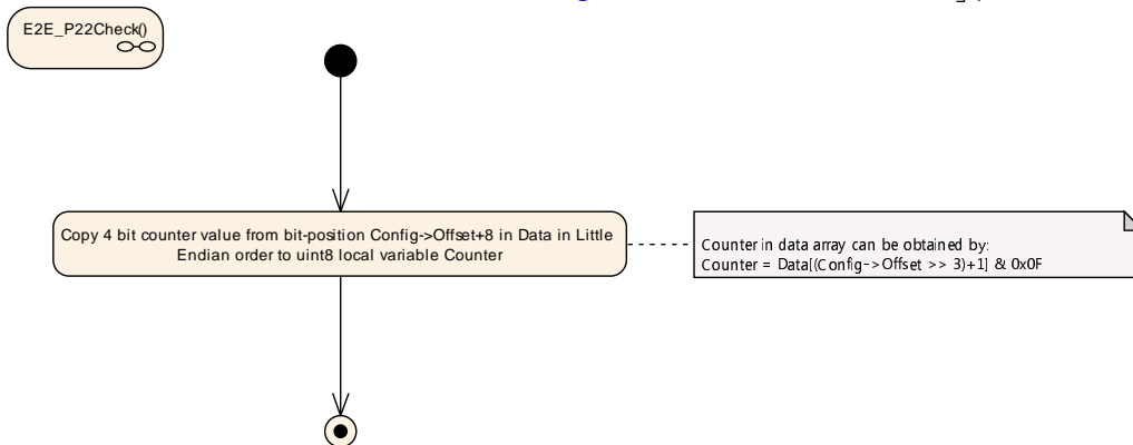
Figure 6.100: E2E Profile 22 Check step "Read Counter"
