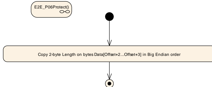
Figure 6.48: E2E Profile 6 Protect step "Write Length"
