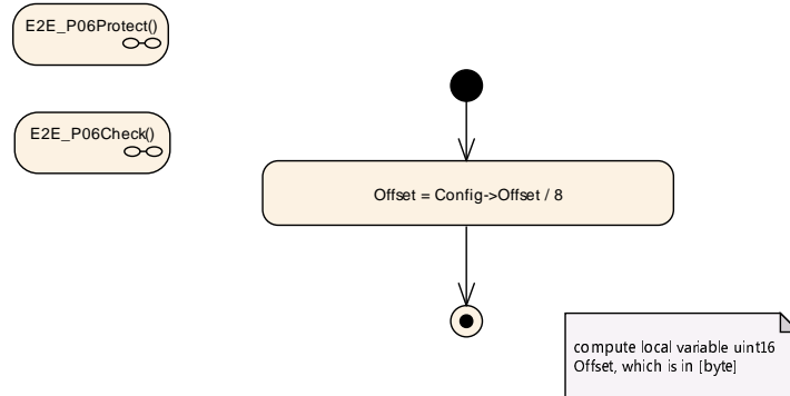
Figure 6.47: E2E Profile 6 Protect step "Compute offset"
