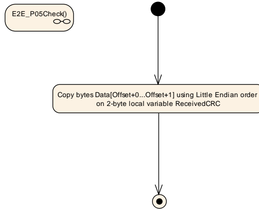
Figure 6.42: E2E Profile 5 Check step "Read CRC"
