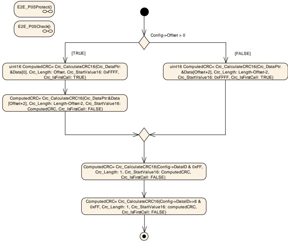
Figure 6.36: E2E Profile 5 Protect and Check step "Compute CRC"
