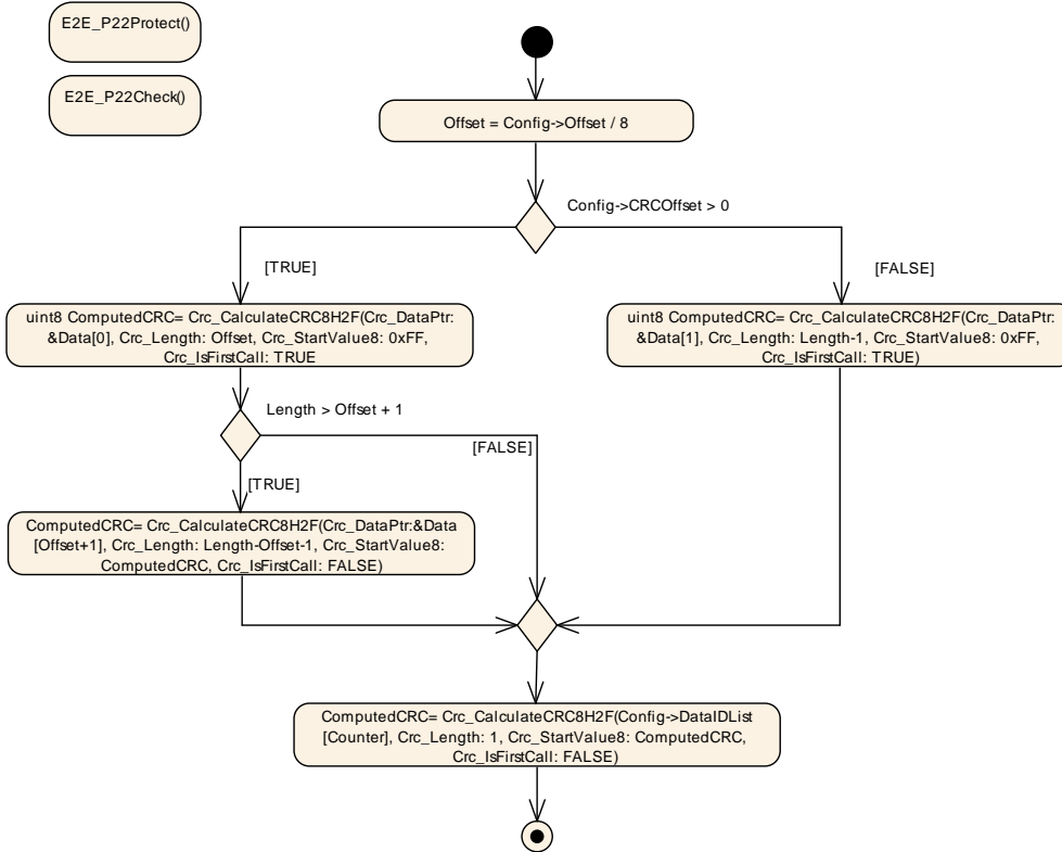
Figure 6.95: E2E Profile 22 Protect and Check step "Compute CRC"
