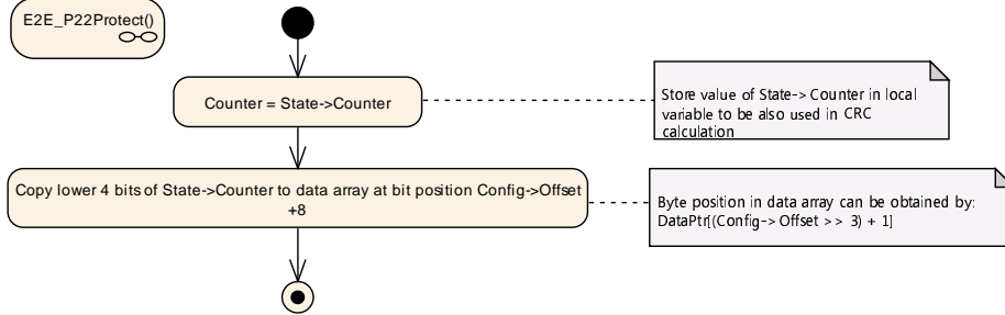
Figure 6.94: E2E Profile 22 Protect step "Write Counter"
