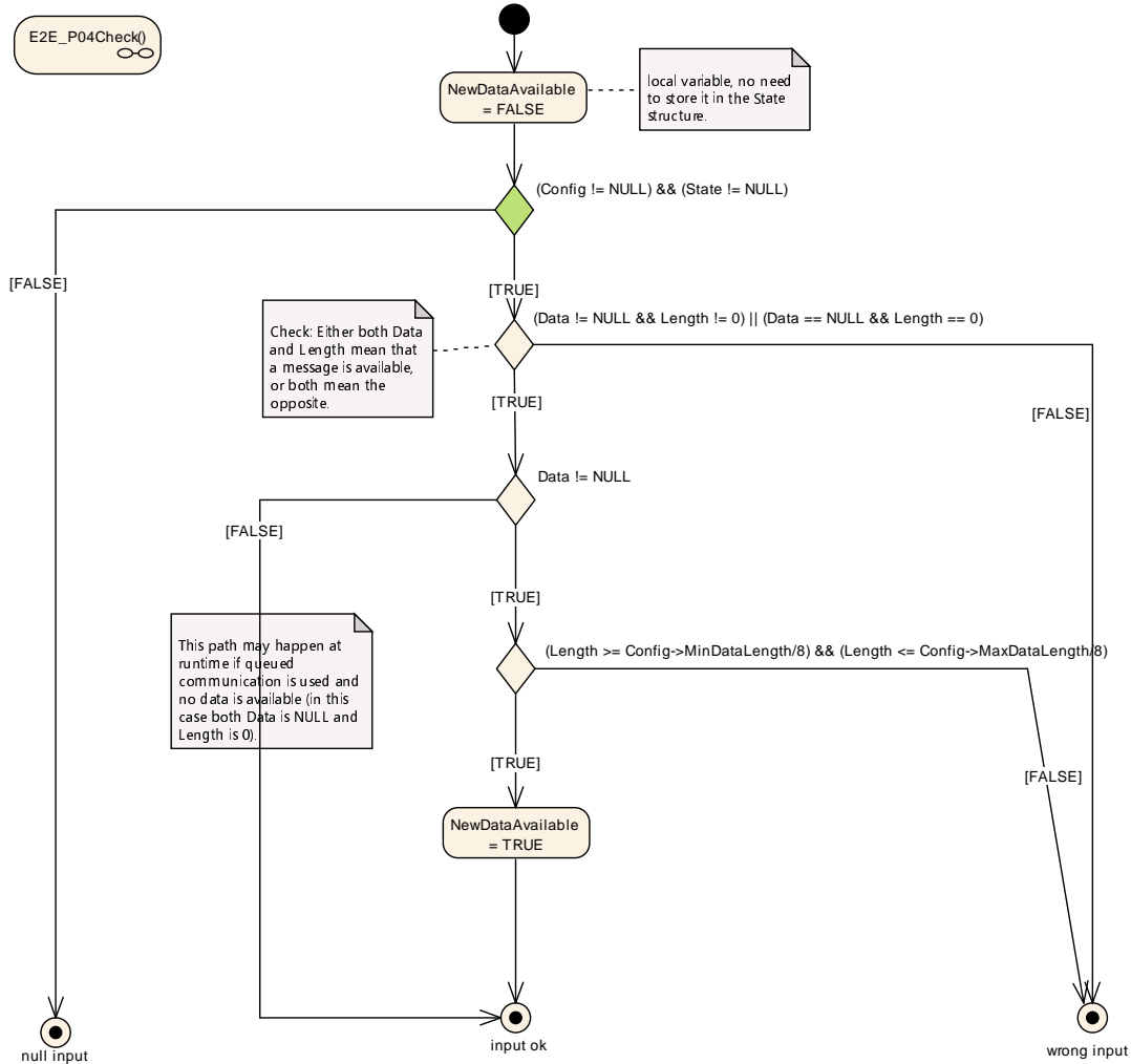
Figure 6.25: E2E Profile Check step 'Verify inputs of the check function'
