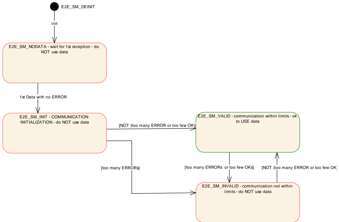
Figure 6.103: E2E state machine overview
