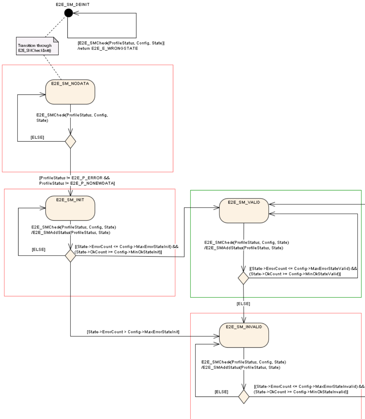
Figure 6.104: E2E state machine check
