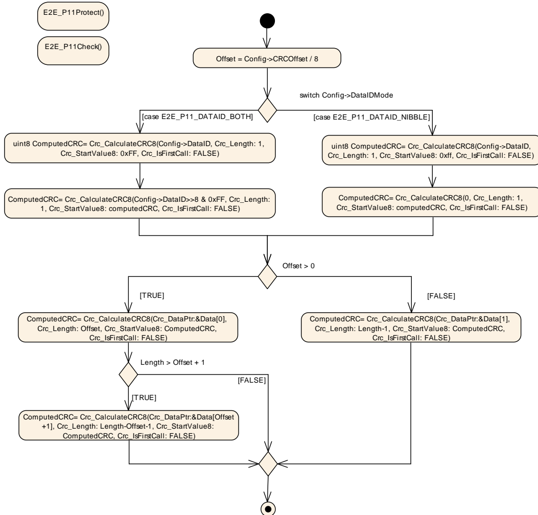
Figure 6.82: E2E Profile 11 Protect and Check step "Compute CRC"
