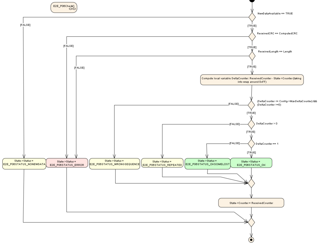
Figure 6.58: E2E Profile 6 Check step "Do Checks"
