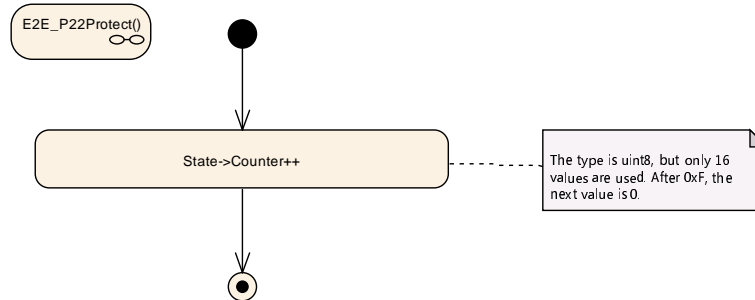
Figure 6.97: E2E Profile 22 Protect step "Increment Counter"
