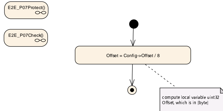
Figure 6.62: E2E Profile 7 Protect step "Compute offset"
