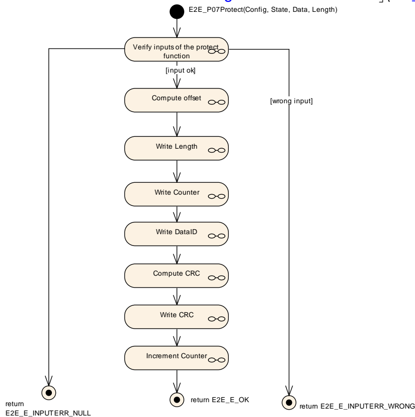
Figure 6.60: E2E Profile 7 Protect
