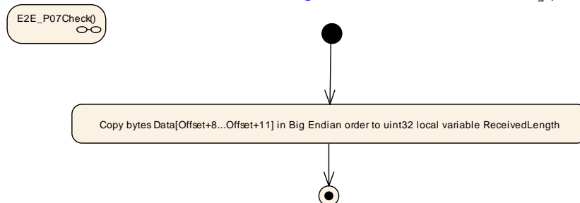
Figure 6.71: E2E Profile 7 Check step "Read Length"
