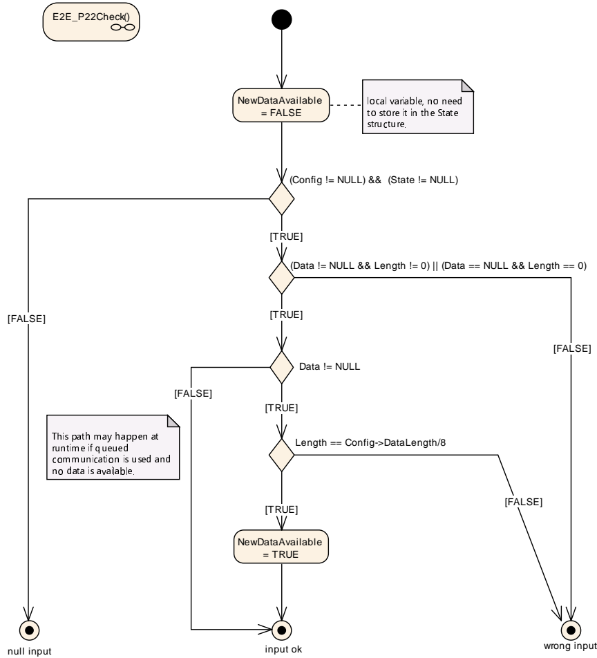
Figure 6.99: E2E Profile 22 Check step "Verify inputs of the check function"
