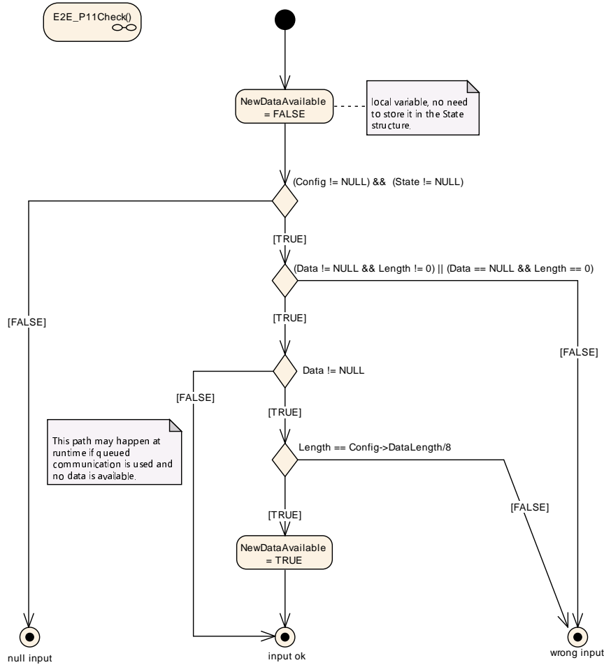
Figure 6.86: E2E Profile 11 Check step "Verify inputs of the check function"
