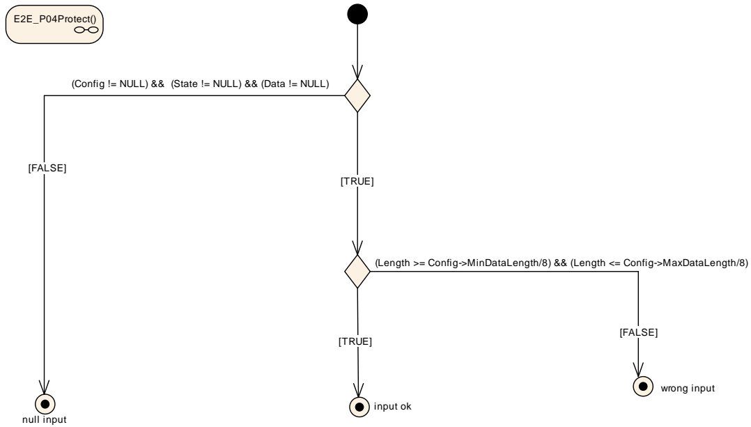
Figure 6.16: E2E Profile 4 Protect step "Verify inputs of the protect function"
