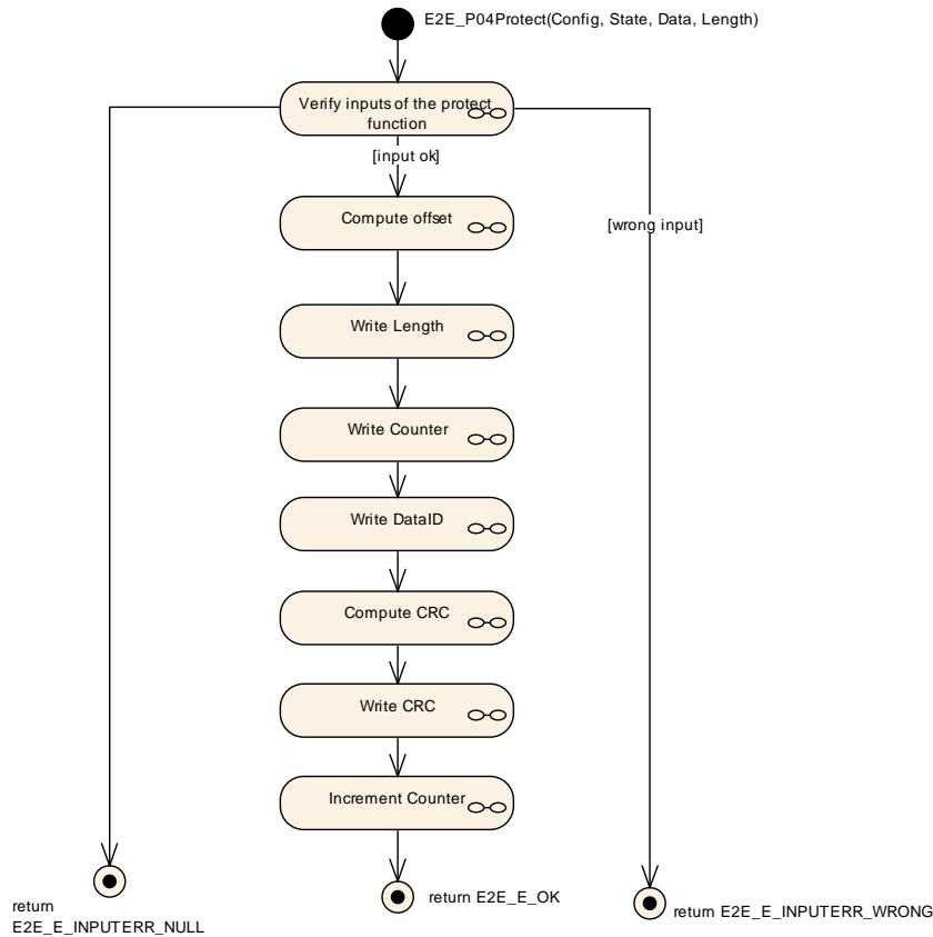
Figure 6.15: E2E Profile 4 Protect
