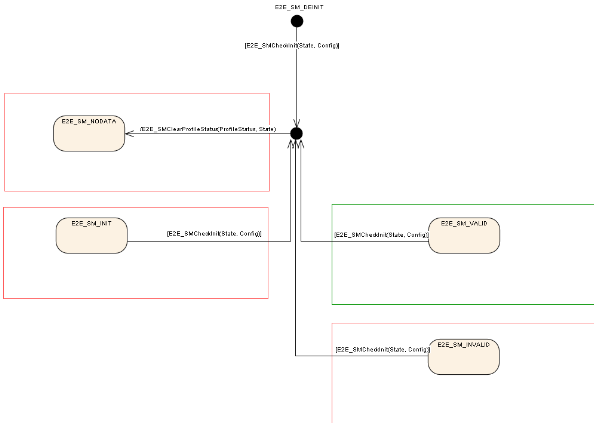
Figure 6.106: E2E state machine step E2E_SMCheckInit
