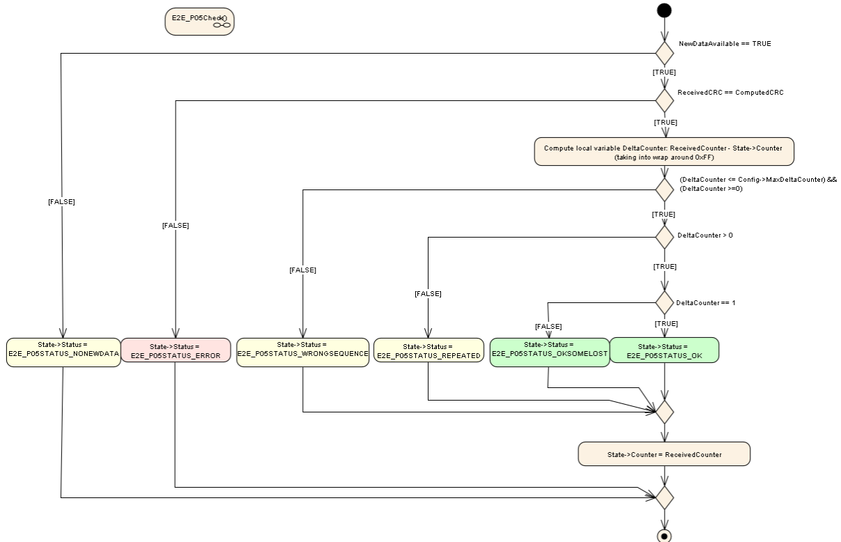
Figure 6.43: E2E Profile 5 Check step "Do Checks"
