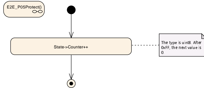
Figure 6.38: E2E Profile 5 Protect step "Increment Counter"
