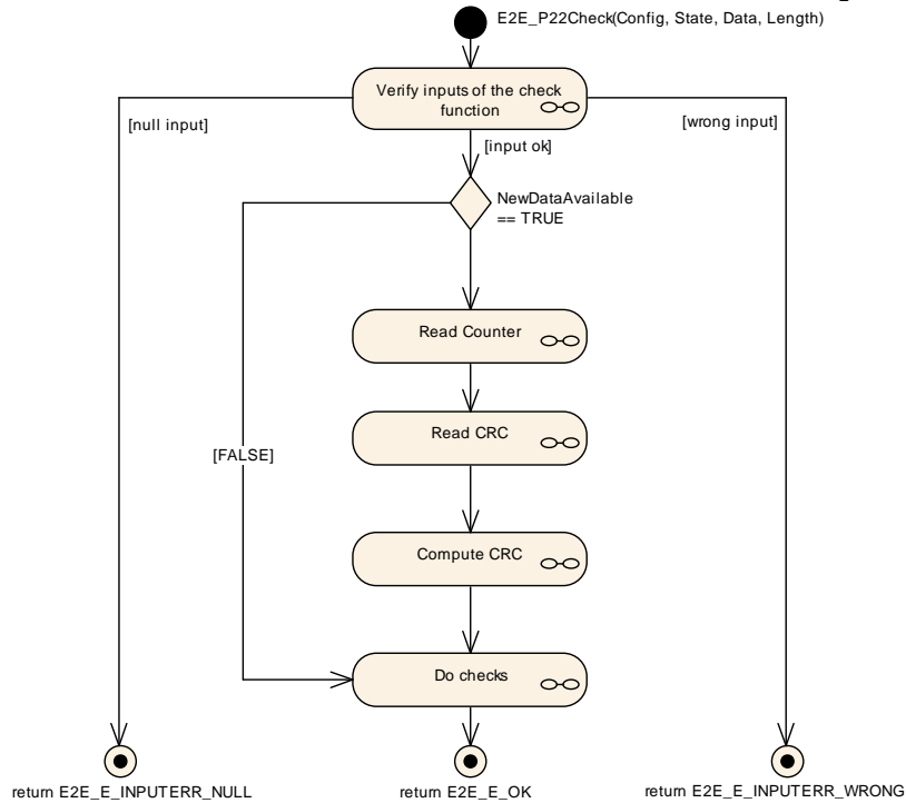
Figure 6.98: E2E Profile 22 Check
