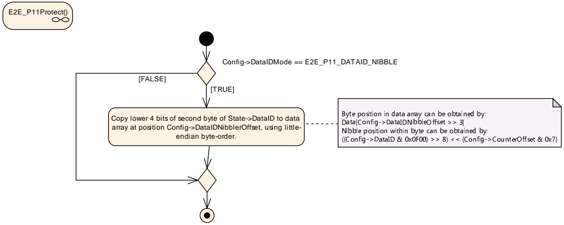
Figure 6.80: E2E Profile 11 Protect step "Write DataIDNibble"
