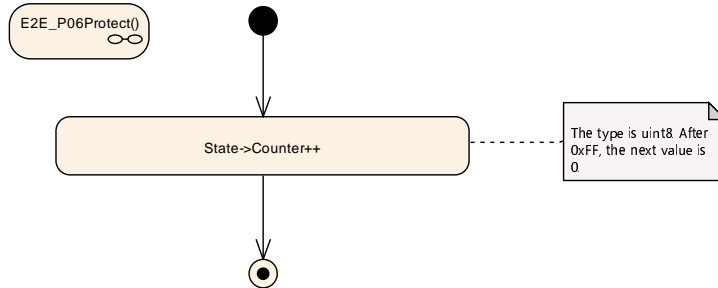
Figure 6.52: E2E Profile 6 Protect step "Increment Counter"
