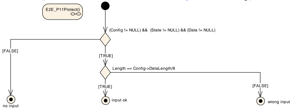
Figure 6.79: E2E Profile 11 Protect step "Verify inputs of the protect function"
