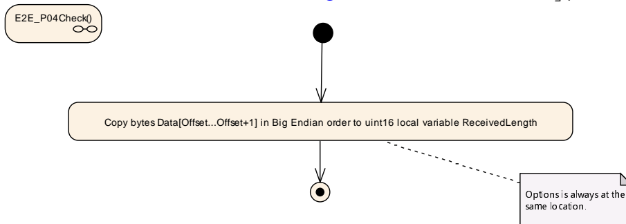
Figure 6.26: E2E Profile Check step "Read Length"
