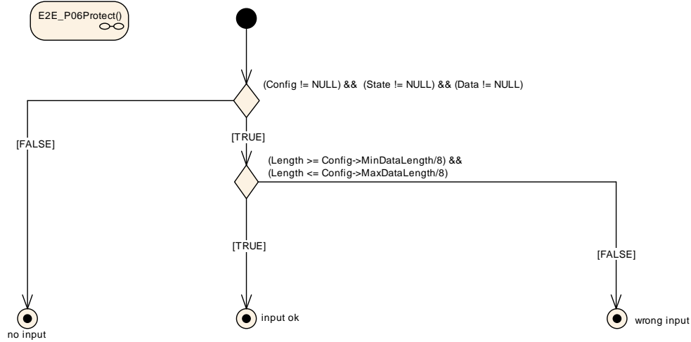
Figure 6.46: E2E Profile 6 Protect step "Verify inputs of the protect function"
