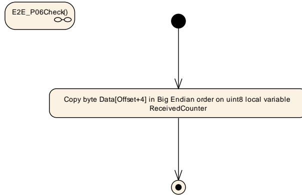
Figure 6.56: E2E Profile 6 Check step "Read Counter"
