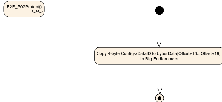
Figure 6.65: E2E Profile 7 Protect step "Write Data ID"
