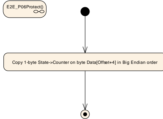
Figure 6.49: E2E Profile 6 Protect step "Write Counter"
