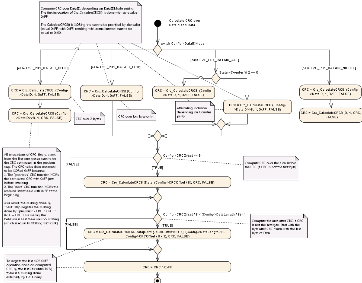
Figure 6.6: Subdiagram „Calculate CRC over Data ID and Data”, used by E2E_P01Protect() and E2E_P01Check()
