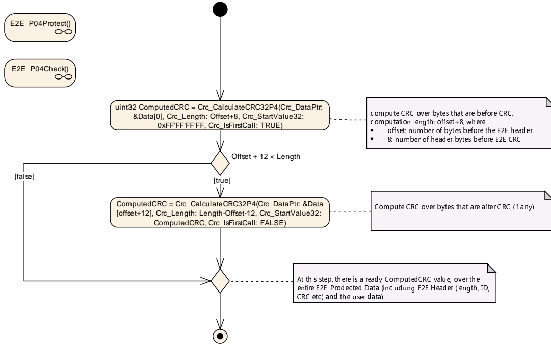
Figure 6.21: E2E Profile 4 Protect and Check step "Compute CRC"
