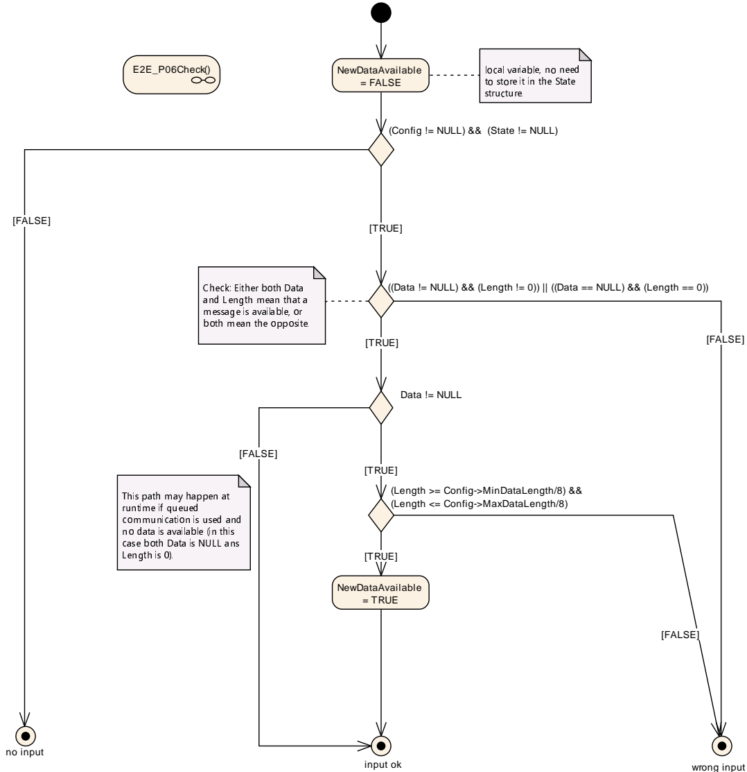
Figure 6.54: E2E Profile 6 Check step "Verify Inputs"
