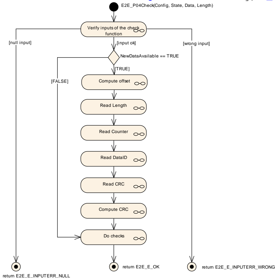
Figure 6.24: E2E Profile Check
