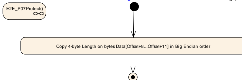
Figure 6.63: E2E Profile 7 Protect step "Write Length"
