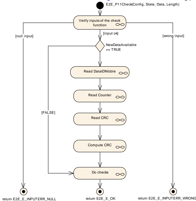
Figure 6.85: E2E Profile 11 Check
