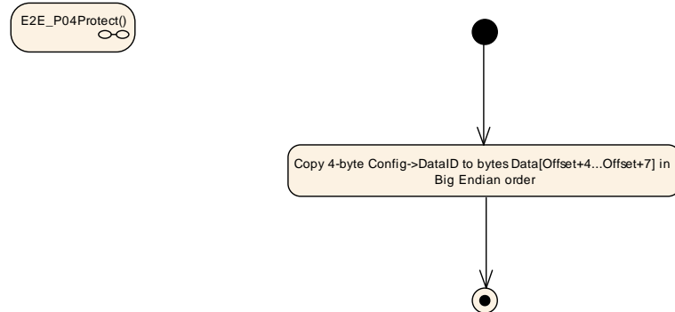
Figure 6.20: E2E Profile 4 Protect step "Write DataID"
