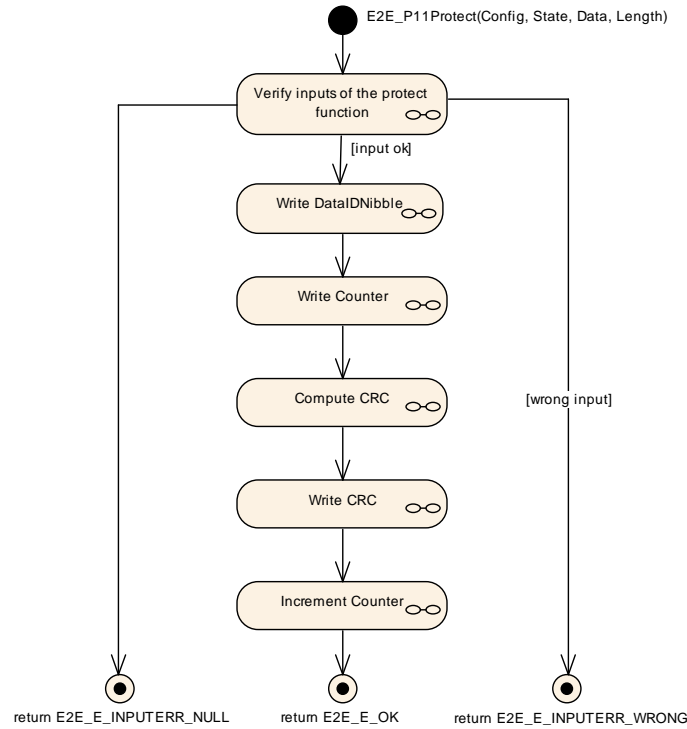
Figure 6.78: E2E Profile 11 Protect
