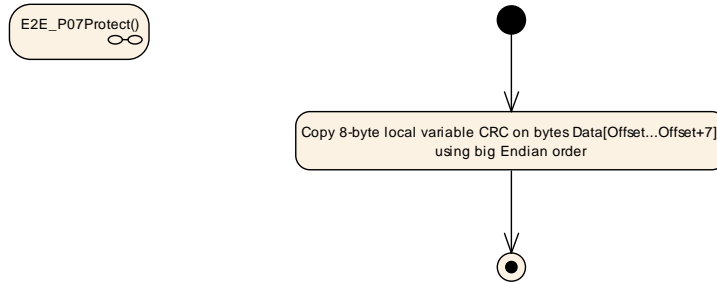
Figure 6.67: E2E Profile 7 Protect step "Write CRC"
