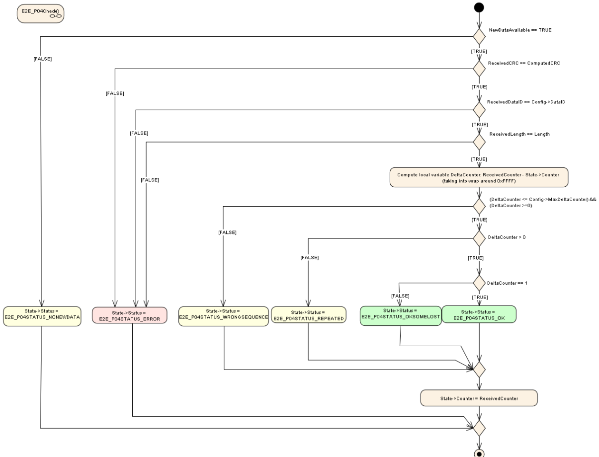
Figure 6.30: E2E Profile 4 Check step "Do Checks"
