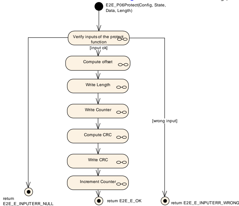
Figure 6.45: E2E Profile 6 Protect
