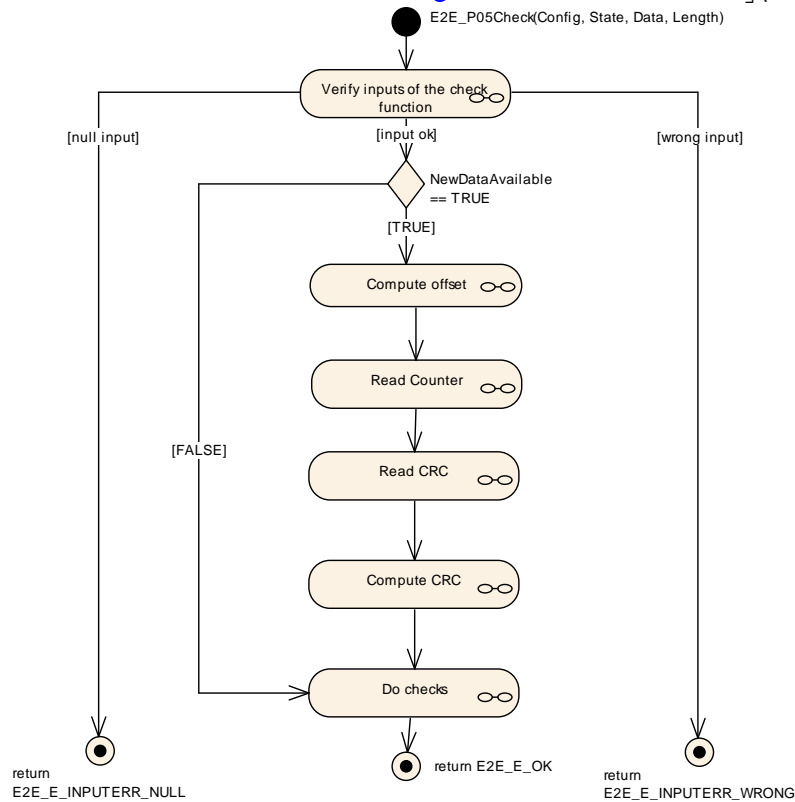
Figure 6.39: E2E Profile 5 Check
