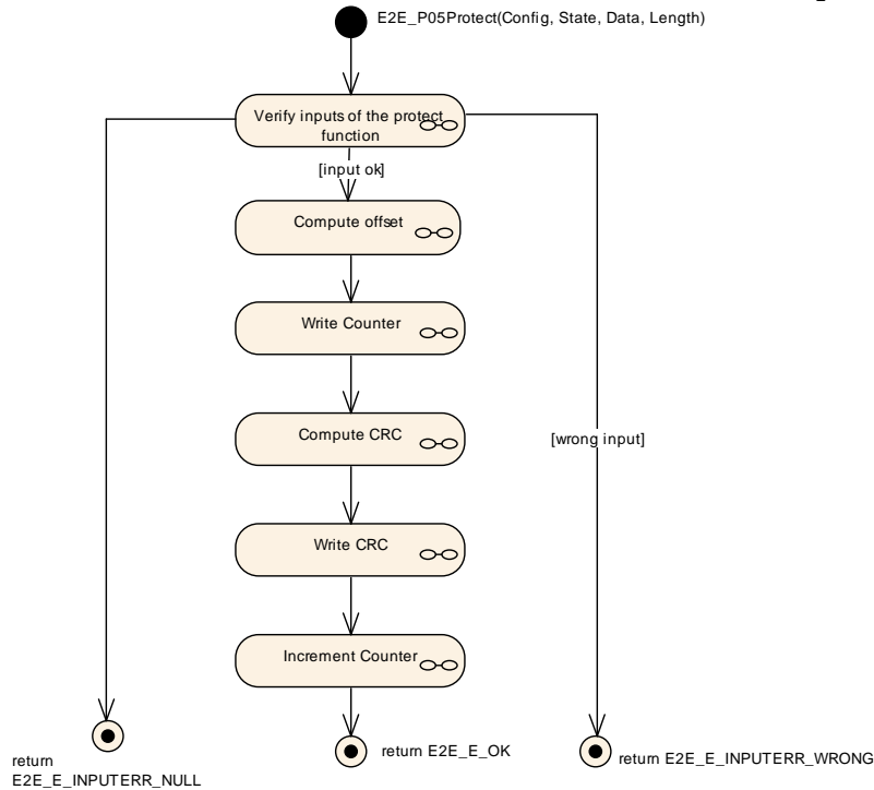
Figure 6.32: E2E Profile 5 Protect
