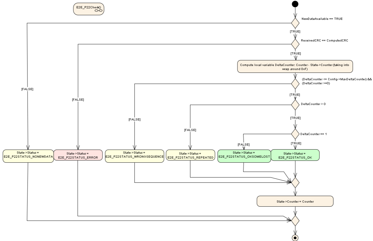
Figure 6.102: E2E Profile 22 Check step "Do Checks"
