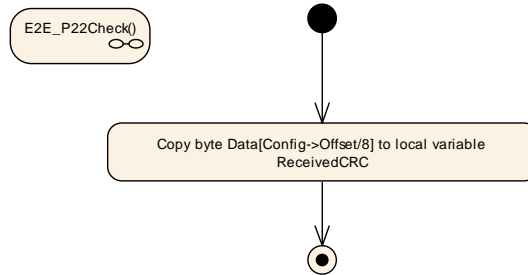
Figure 6.101: E2E Profile 22 Check step "Read CRC"
