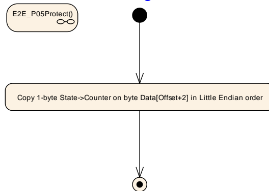
Figure 6.35: E2E Profile 5 Protect step "Write Counter"
