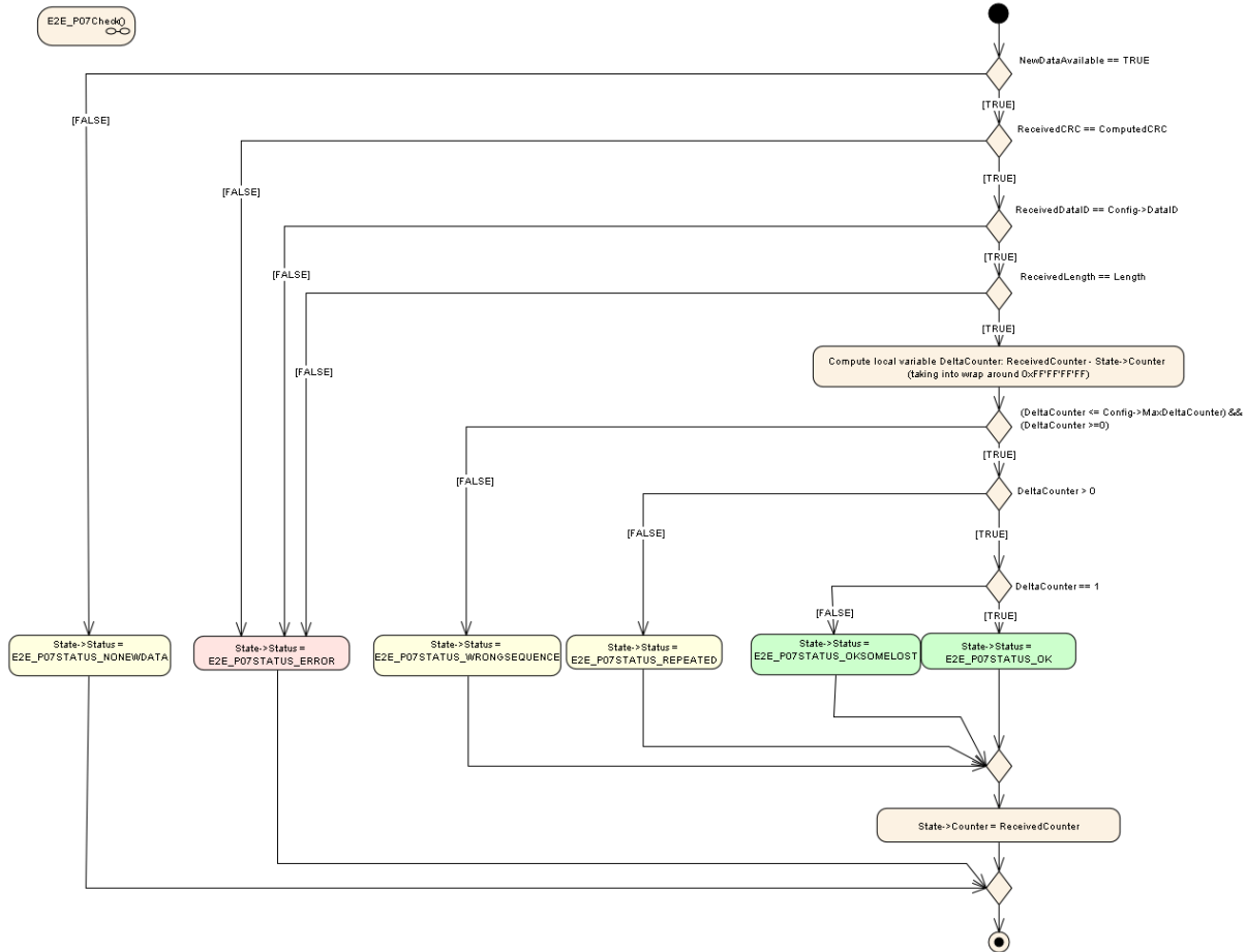
Figure 6.75: E2E Profile 7 Check step "Do Checks"
