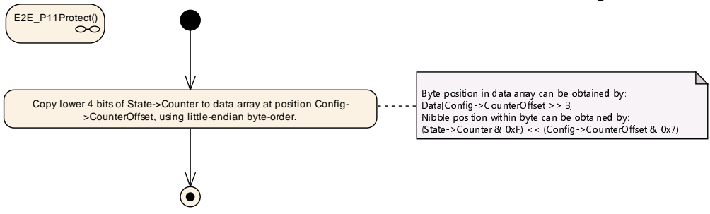
Figure 6.81: E2E Profile 11 Protect step "Write Counter"
