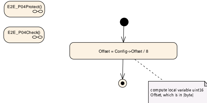
Figure 6.17: E2E Profile 4 Protect step "Compute offset"
