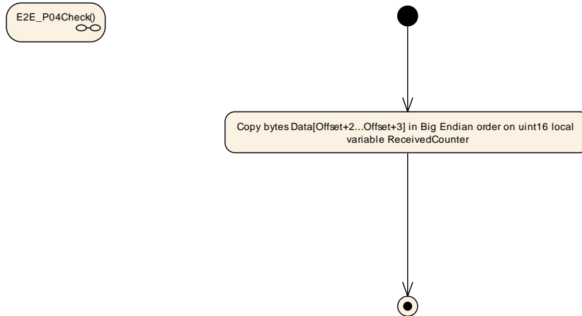
Figure 6.27: E2E Profile Check step "Read Counter"
