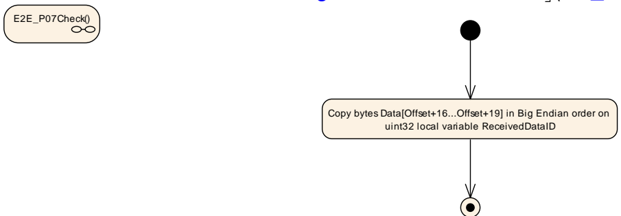
Figure 6.73: E2E Profile 7 Check step "Read DataID"
