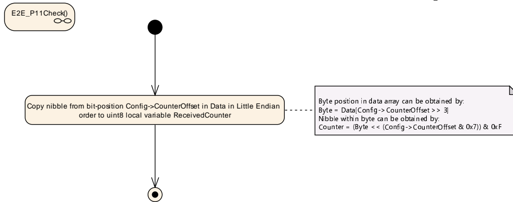
Figure 6.88: E2E Profile 11 Check step "Read Counter"
