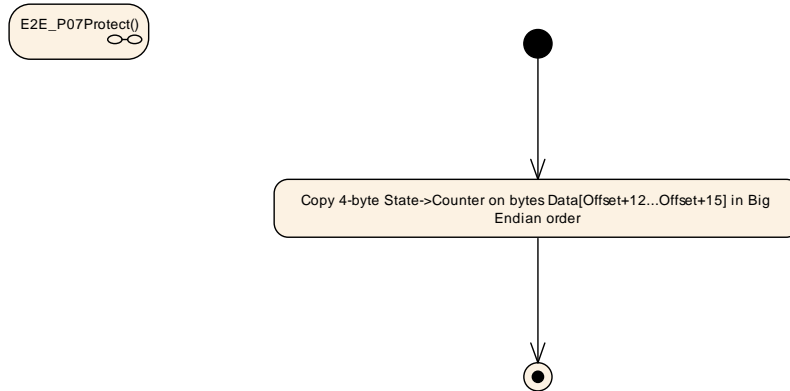
Figure 6.64: E2E Profile 7 Protect step "Write Counter"
