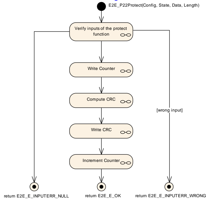
Figure 6.92: E2E Profile 22 Protect
