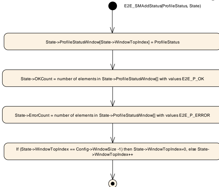
Figure 6.105: E2E state machine step E2E_SMAddStatus
