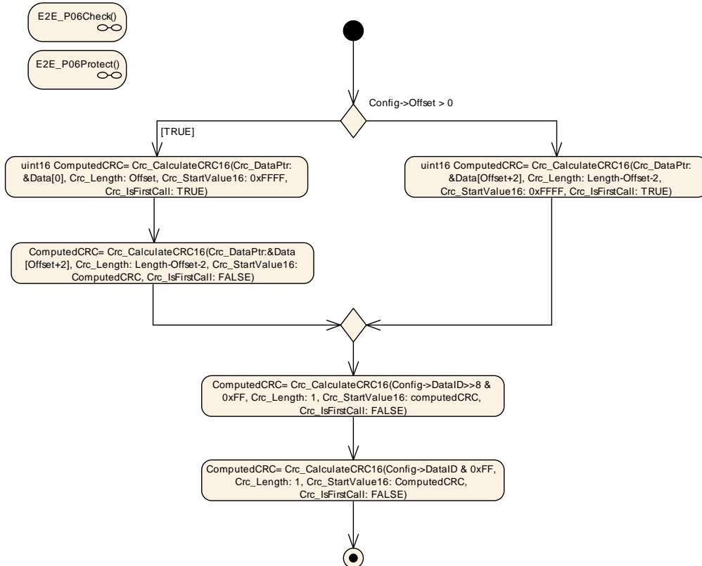
Figure 6.50: E2E Profile 6 Protect and Check step "Compute CRC"
