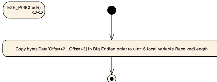
Figure 6.55: E2E Profile 6 Check step "Read Length"
