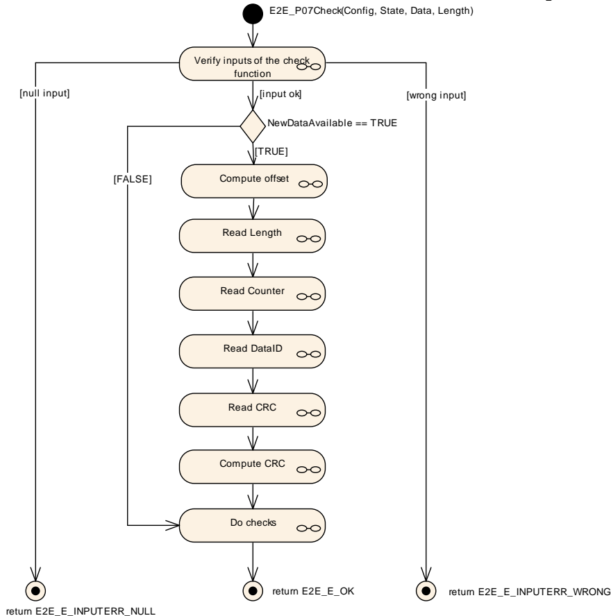
Figure 6.69: E2E Profile 7 Check
