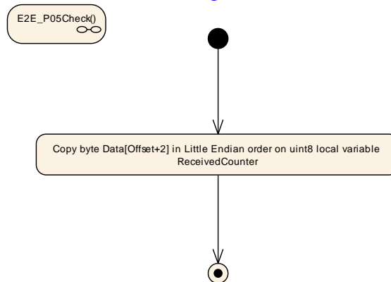
Figure 6.41: E2E Profile 5 Check step "Read Counter"
