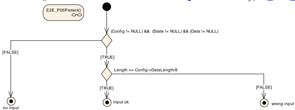
Figure 6.33: E2E Profile 5 Protect step "Verify inputs of the protect function"
