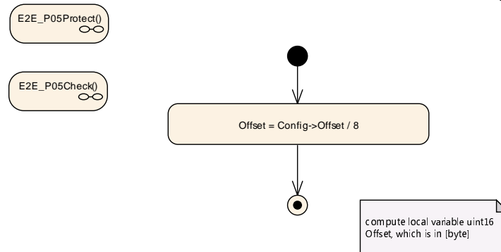
Figure 6.34: E2E Profile 5 Protect step "Compute offset"
