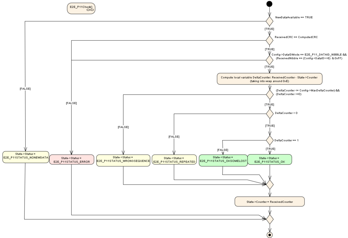
Figure 6.90: E2E Profile 11 Check step "Do Checks"
