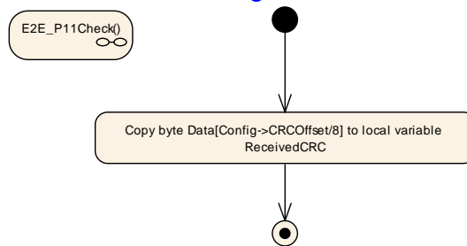
Figure 6.89: E2E Profile 11 Check step "Read CRC"
