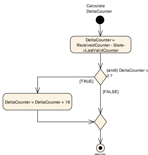
Figure 6.13: Calculate Delta Counter
