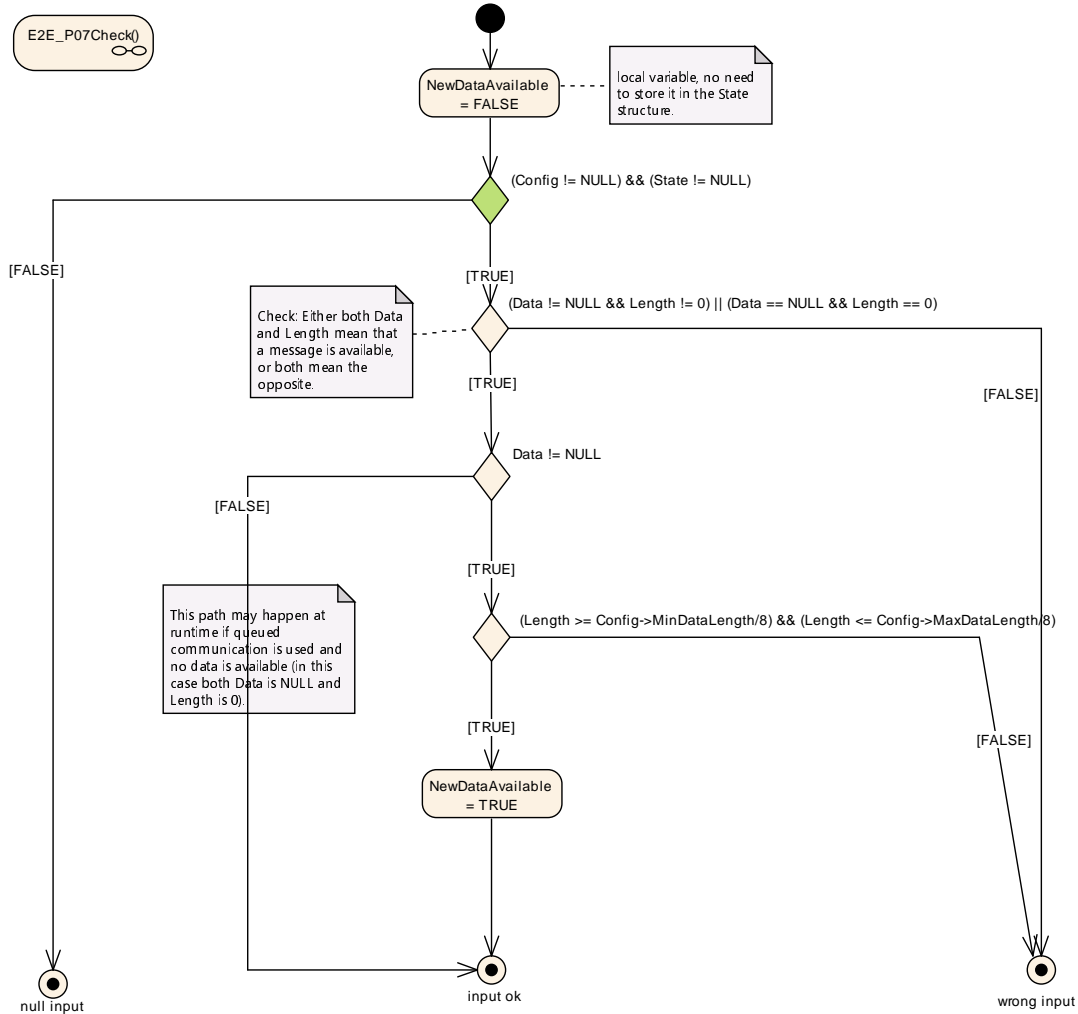
Figure 6.70: E2E Profile 7 Check step "Verify inputs of the check function"
