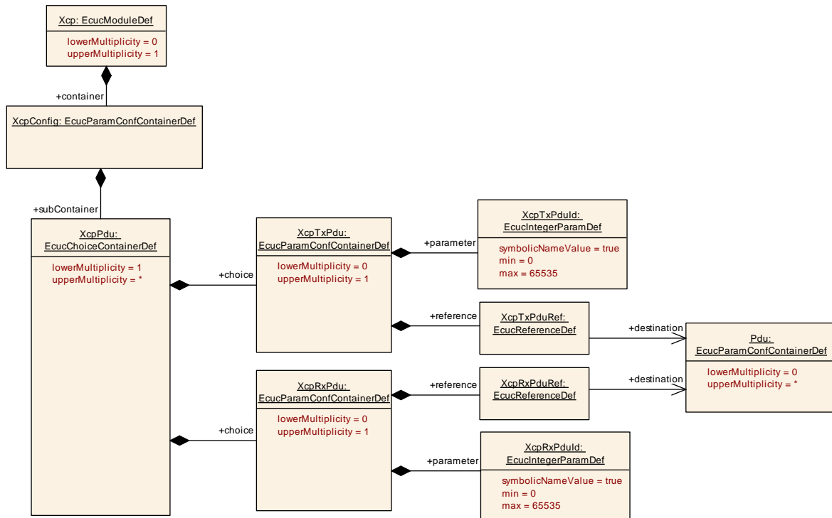
Figure 10: Diagram XcpPdu
