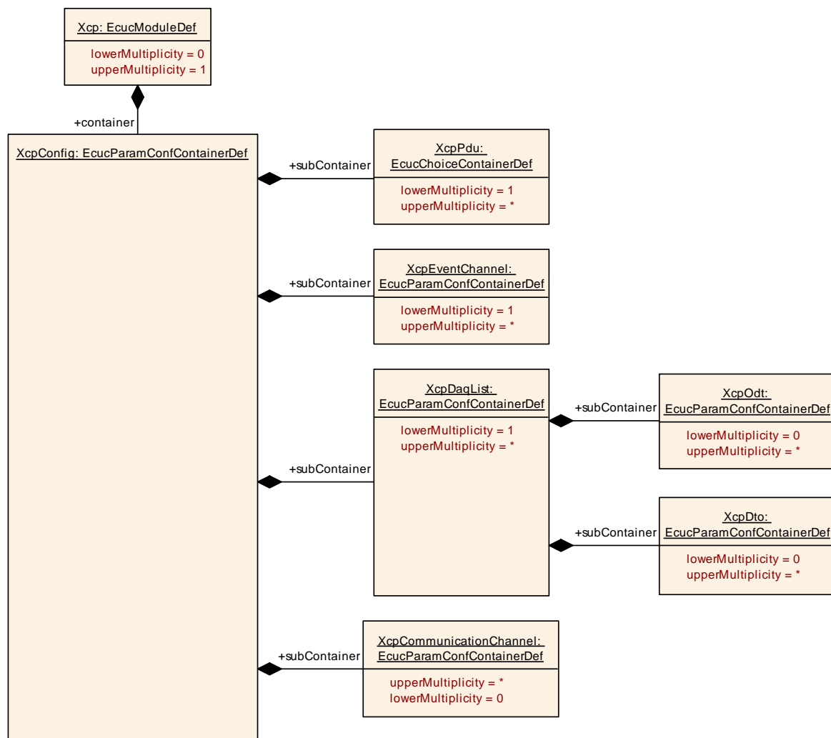
Figure 8: Diagram XcpConfig
