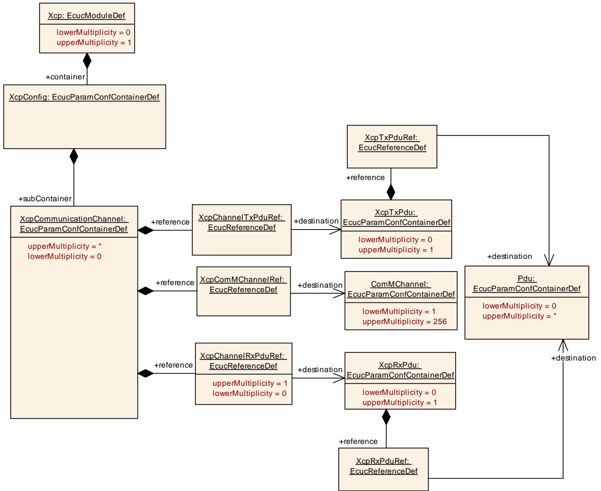
Figure 11: Diagram XcpCommunicationChannel
