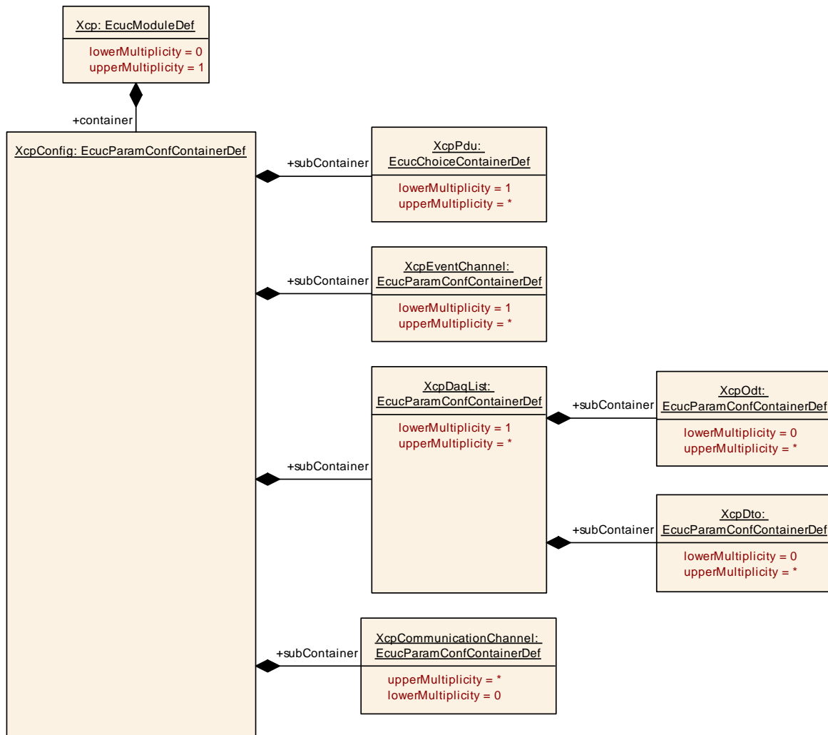
Figure 8: Diagram XcpConfig
