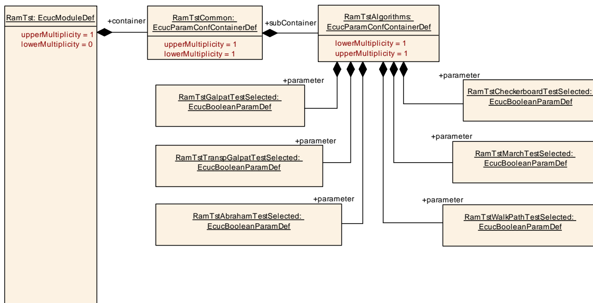
Figure 16: RamTstAlgorithms
