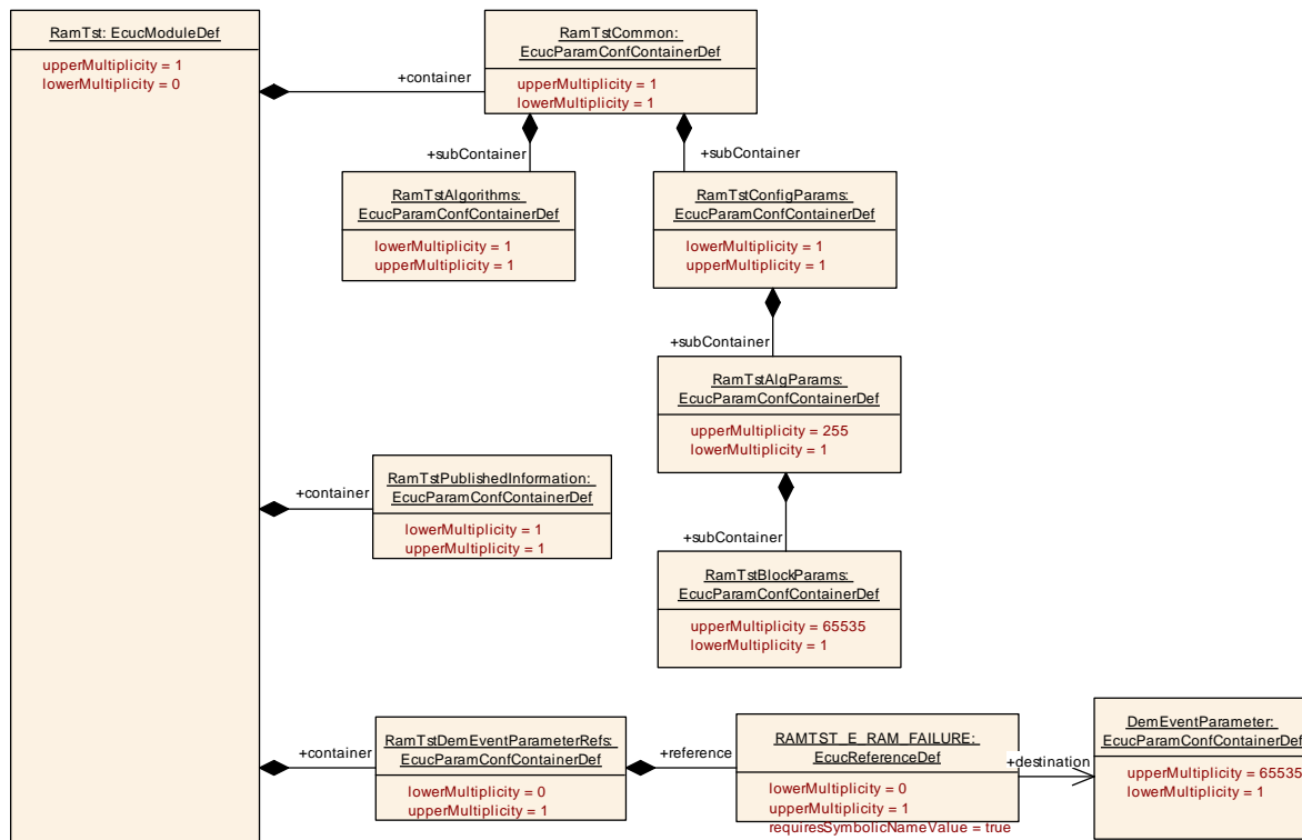
Figure 14: RAM Test Configuration Overview
