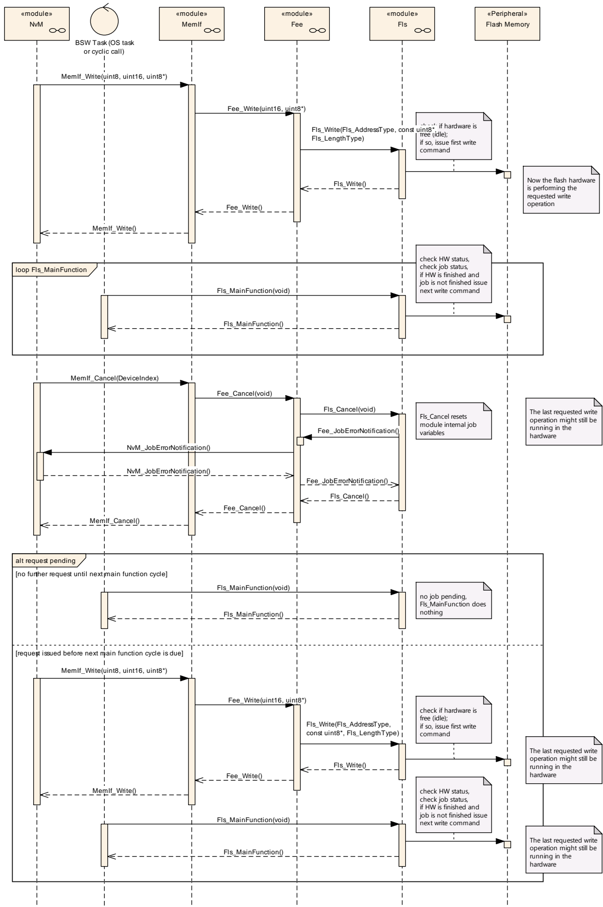
Figure 6: Sequence diagram „Fee_Cancel“
