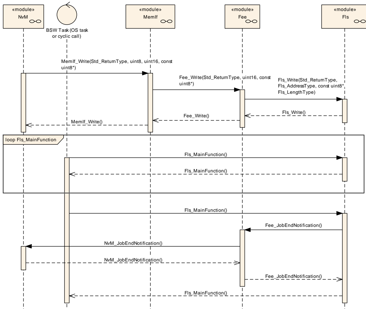
Figure 5: Sequence diagram “Fee_Write”
