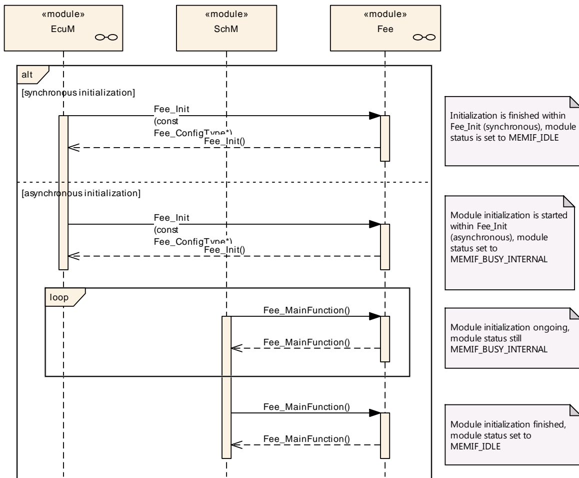
Figure 4: Sequence diagram of “ Fee_Init ” service
