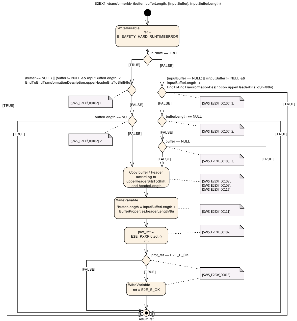
Figure 7-1: E2EXf_<transformerId>function overview
