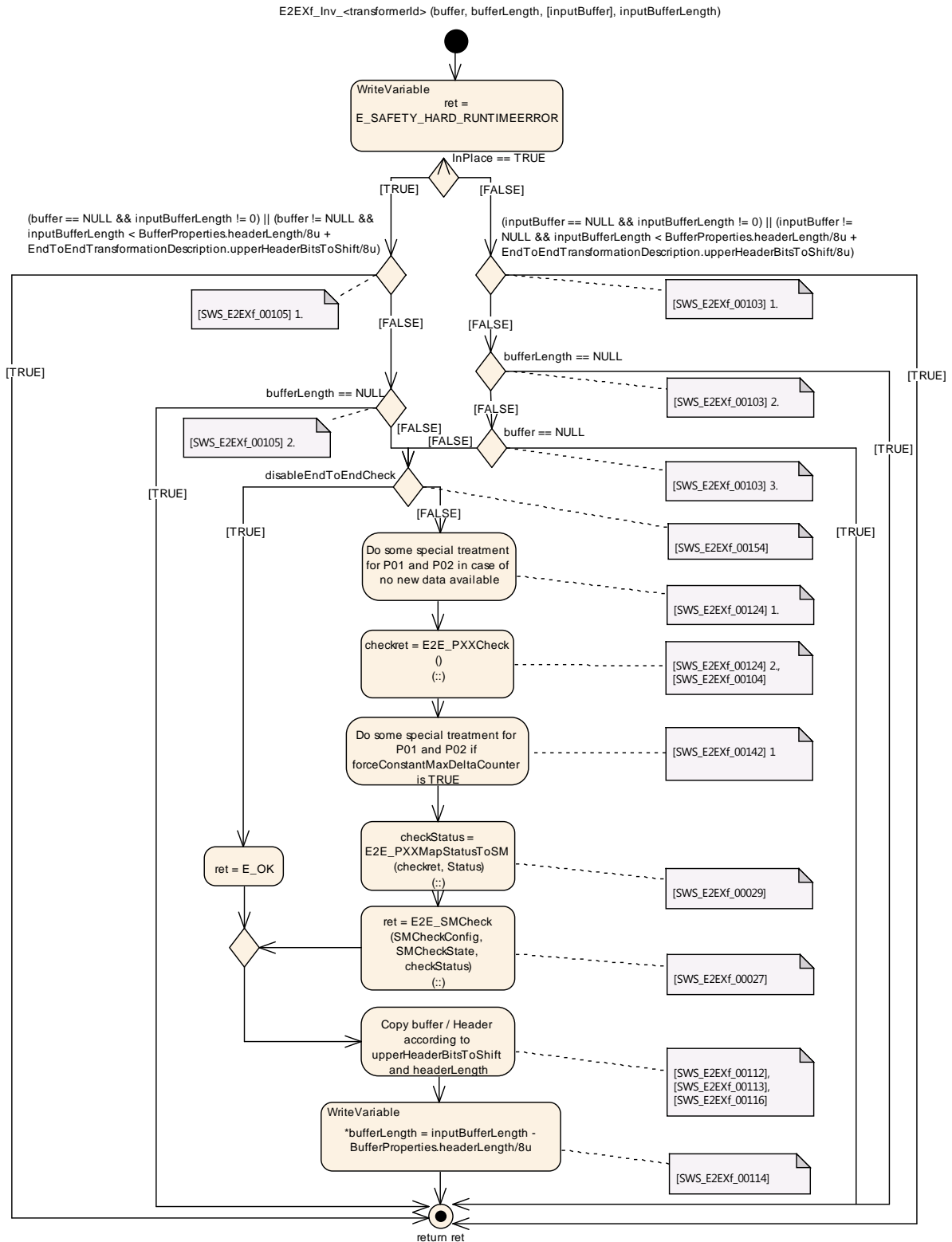
Figure 7-4: E2EXf_Inv_<transformerId>function overview
