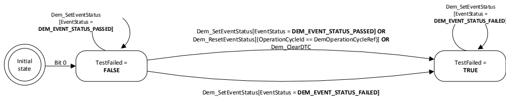
Figure 7.17: UDS status bit 0 TestFailed logic
