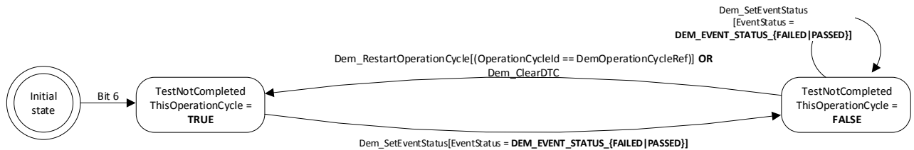
Figure 7.23: UDS status bit 6 TestNotCompleteThisOperationCycle logic
