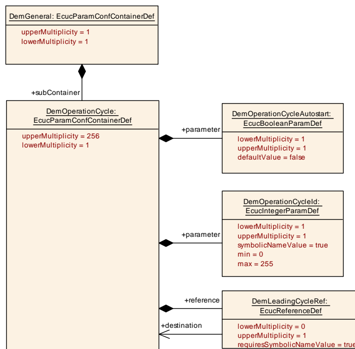
Figure 7.12: Operation cycle configuration
