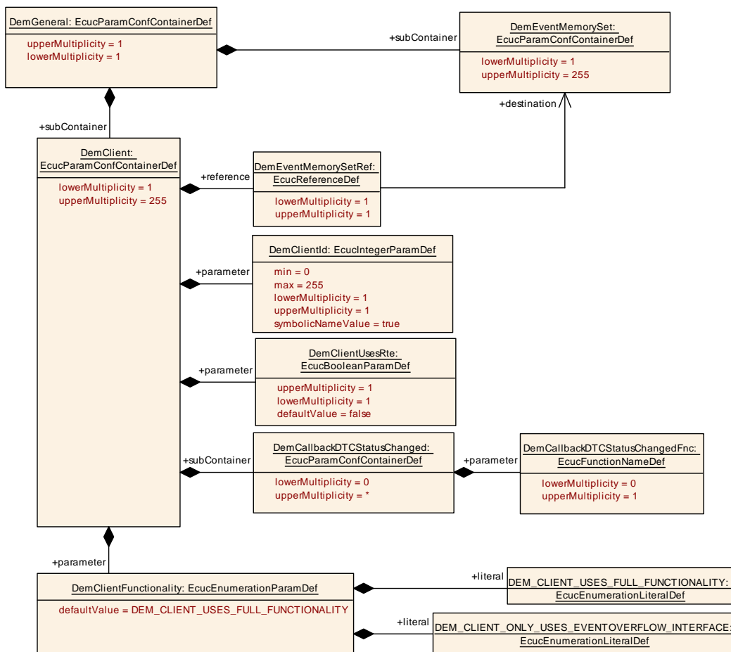
Figure 10.4: DemClient
