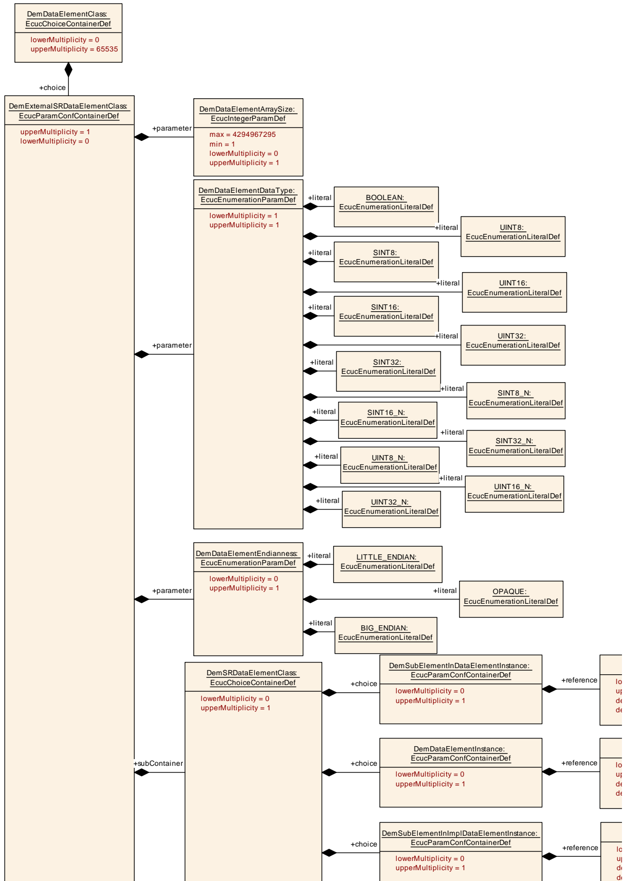
Figure 10.14: DemExternalSRDataElementClass
