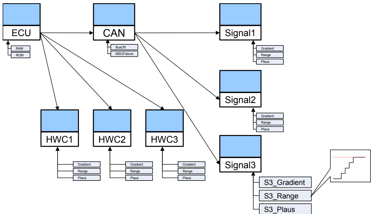
Figure 7.11: Event dependencies
