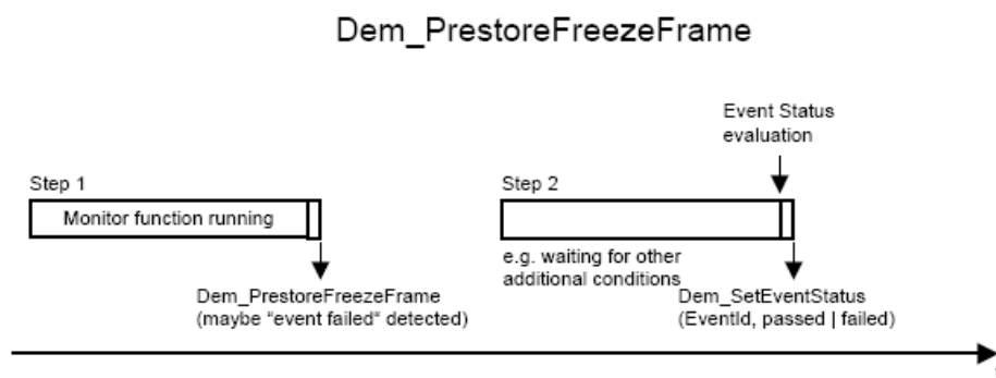
Figure 7.40: Example to use Dem_PrestoreFreezeFrame to prestore freeze frame data
