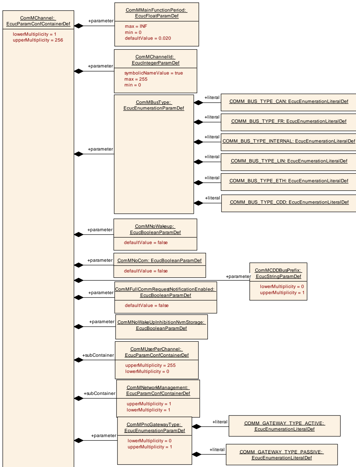
Figure 16: Configuration ComMChannel
