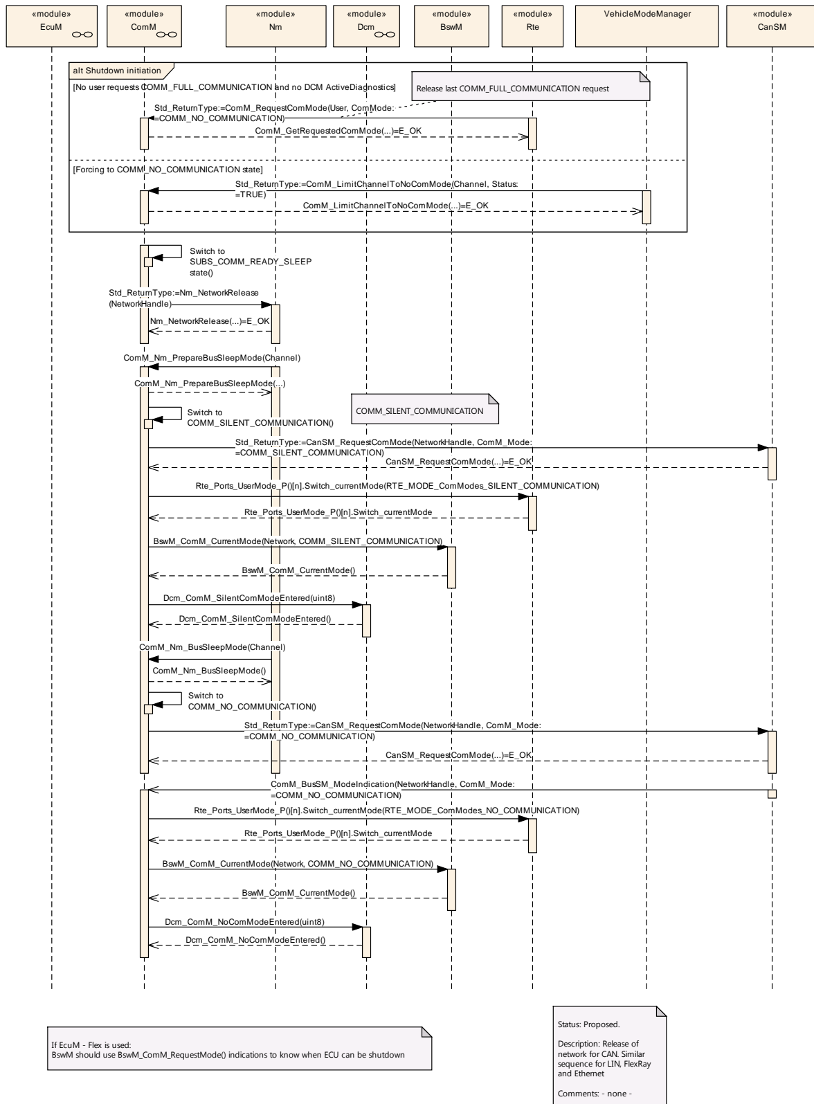
Figure 11 shows the possibilities to shutdown the CAN network. It can be either initiated if the last user releases his COMM_FULL_COMMUNICATION request or ComM_LimitChannelToNoComMode(...) (see SWS ComM_00163 ) is called. The behaviour is equal for LIN, FlexRay and Ethernet just with different API names.
