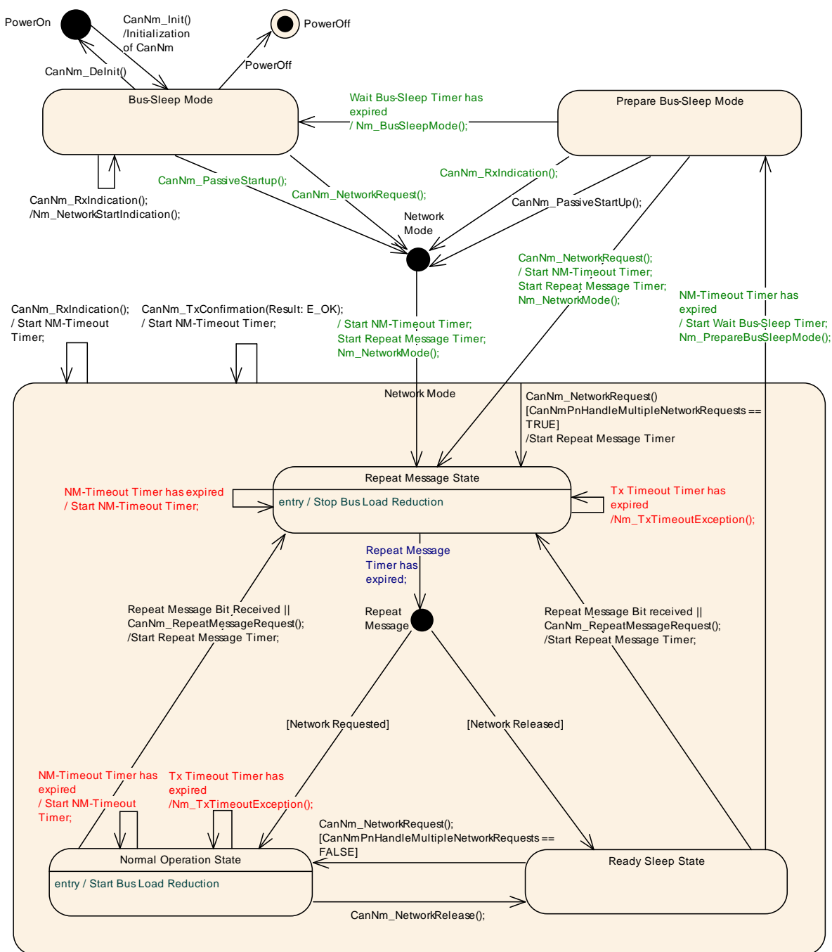
Figure 7-5 CanNm Algorithm
