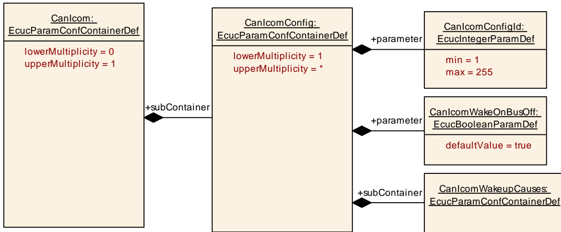
Figure 10-7: CanIcom Layout
