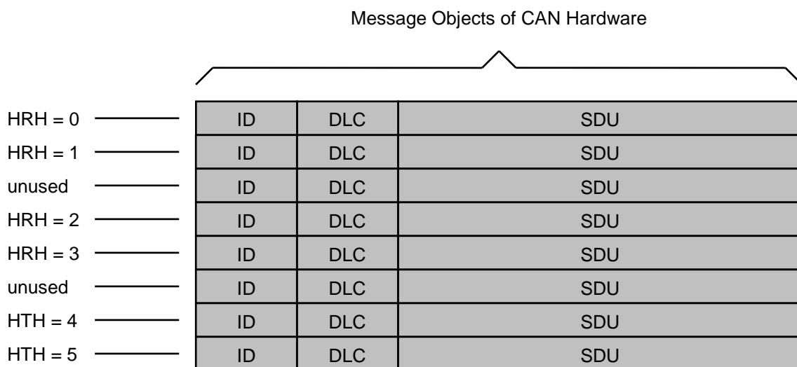
Figure 7-3: Example of assignment of HTHs and HRHs to the Hardware Objects. The numbering of HTHs and HRHs are implementation specific. The chosen numbering is only an example.
