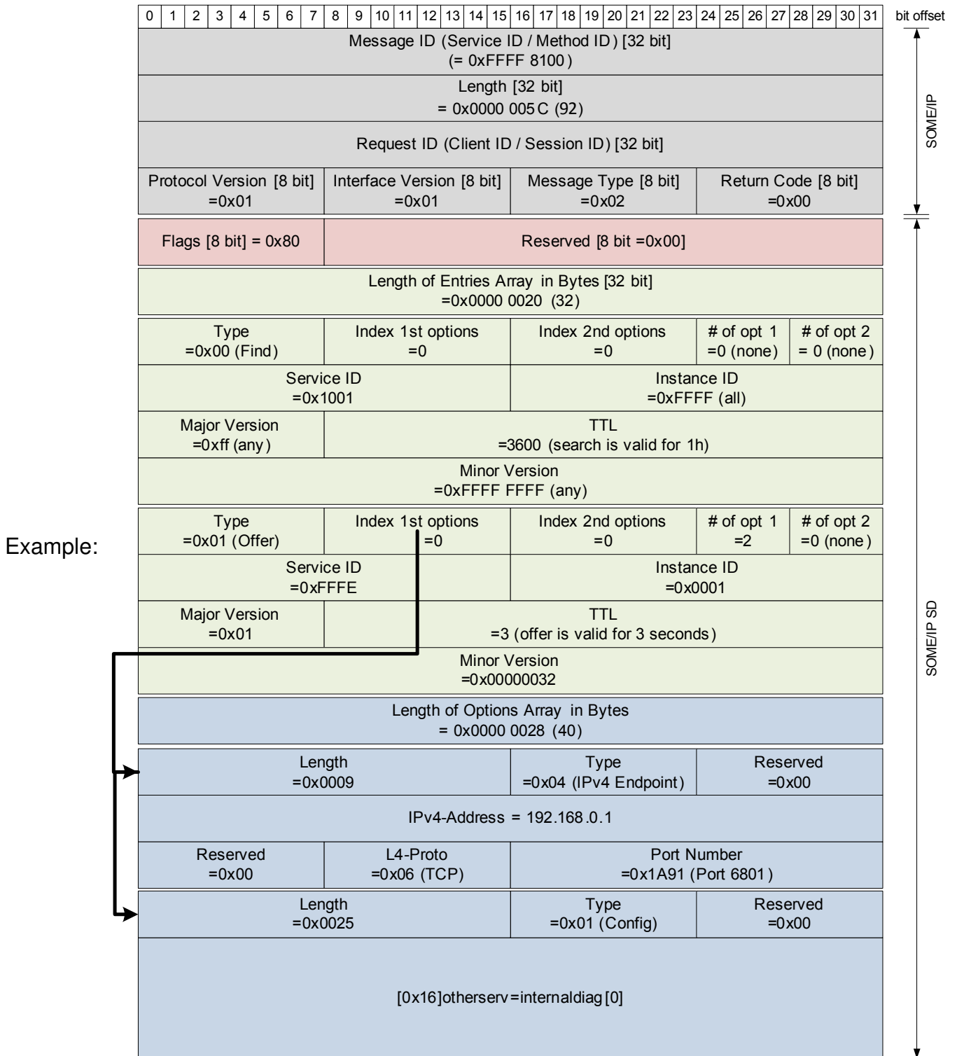
Figure 4.19: SOME/IP-SD Example PDU for Non-SOME/IP-SD
