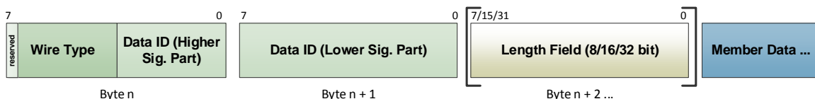
Figure 4.5: Tag Layout
