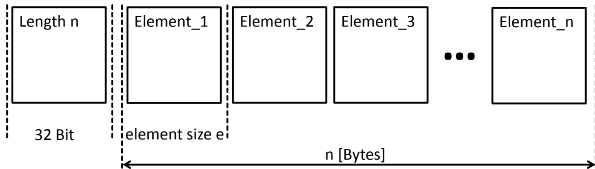
Figure 4.12: One-dimensional array (dynamic length)
