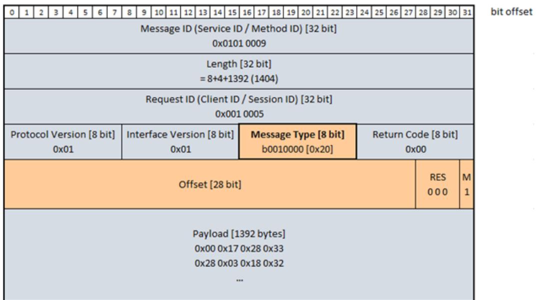
Figure 4.18: Example: Header of the SOME/IP segments
