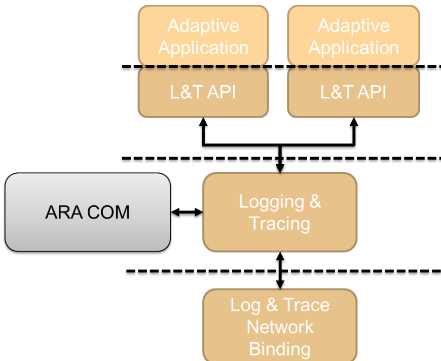
Figure 16-1 Overview Log and Trace
