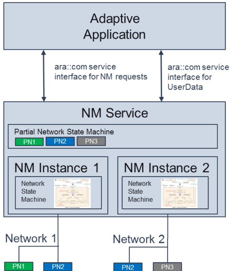
Figure 12-1 Overview Adaptive NM
