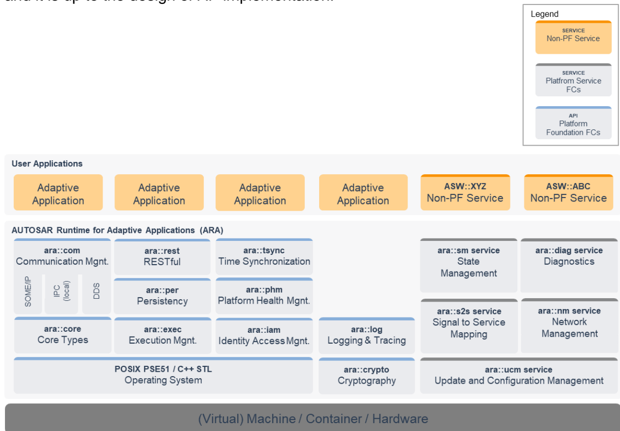
Figure 3-1 AP architecture logical view
