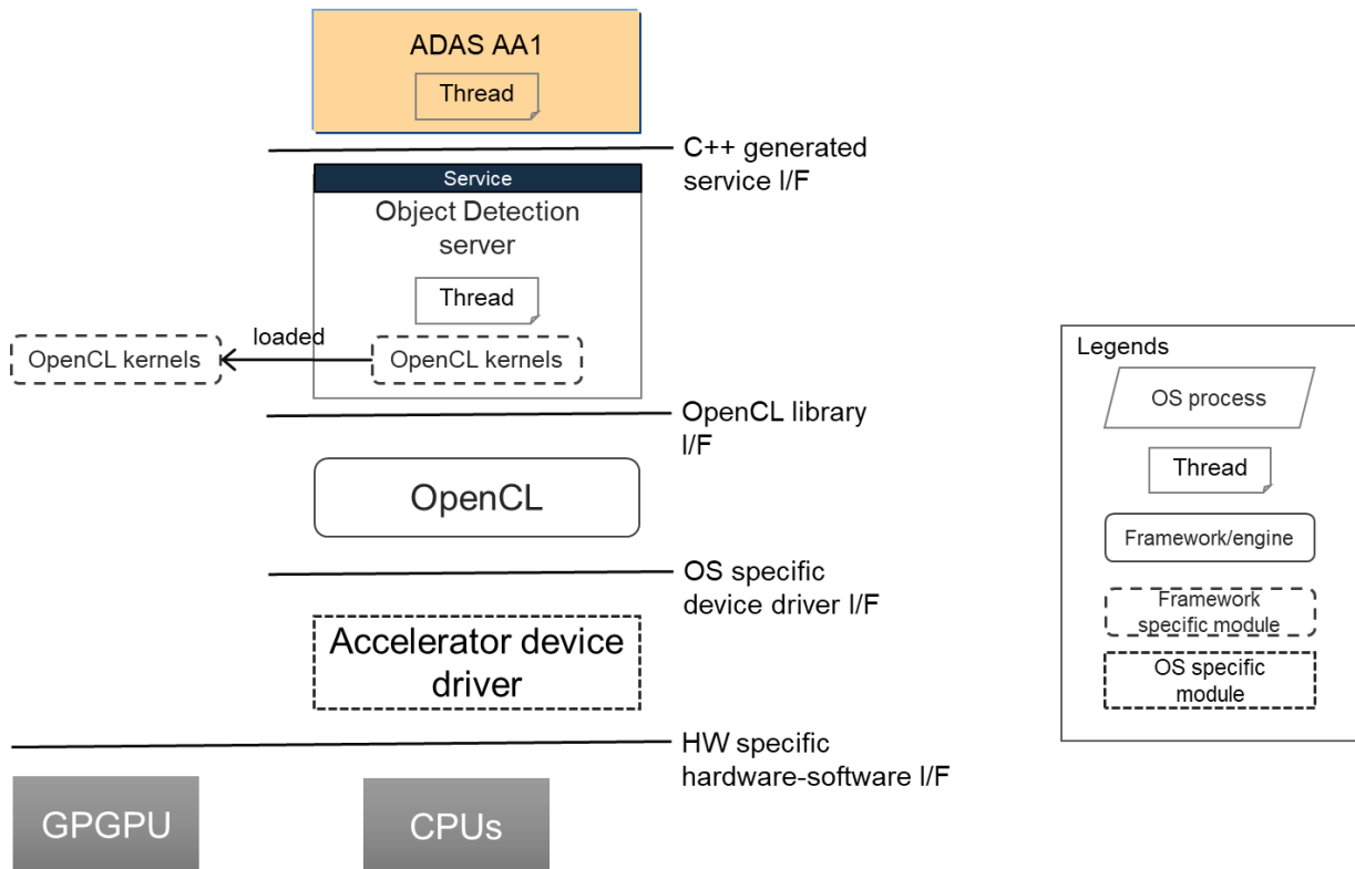
Figure 3-2 Accelerator-model example
