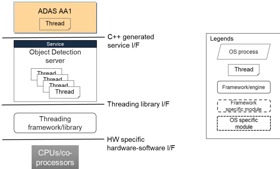
Figure 3-3 CPU/co-processor-model example
