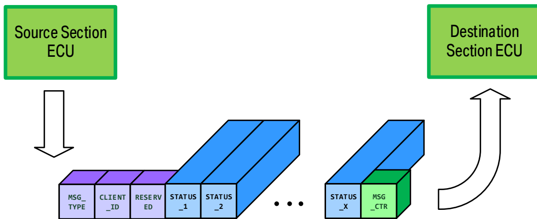
Figure 5.2: DTC Status Message Structure
